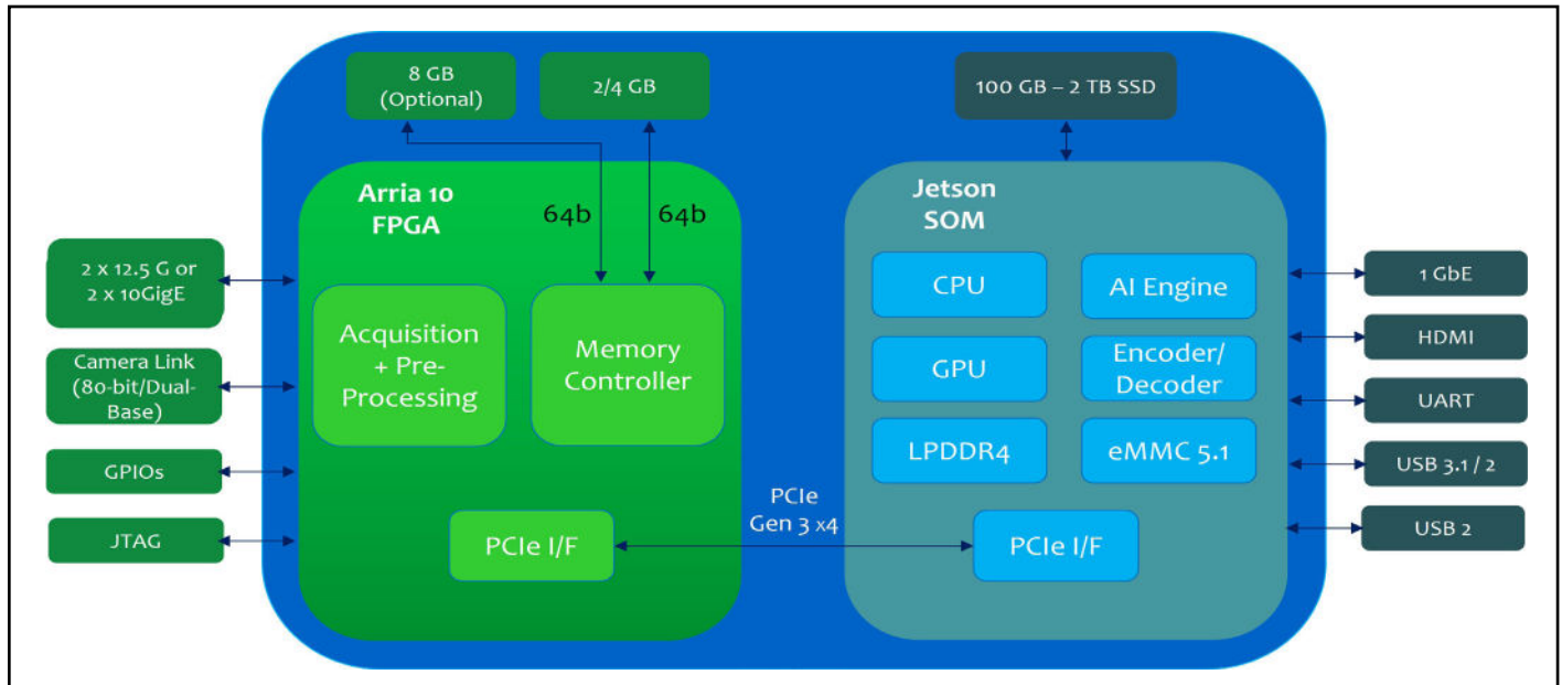
Fanto Vision 20 System Block Diagram
