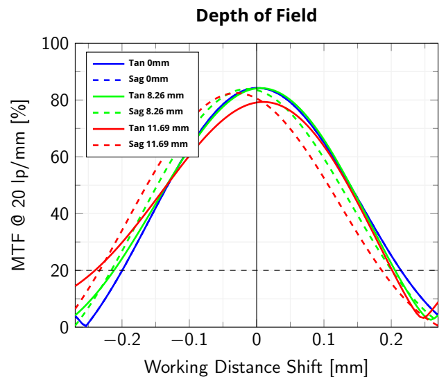
Modulation Transfer Function (MTF) @ 20 lp/mm vs. Working Distance Shift from the best focus Working Distance, wavelength range 400-700 nm, wf/N = 10
