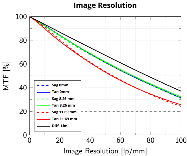
Modulation Transfer Function (MTF) vs. Image Resolution, wavelength range 400-700 nm, wf/N = 10
