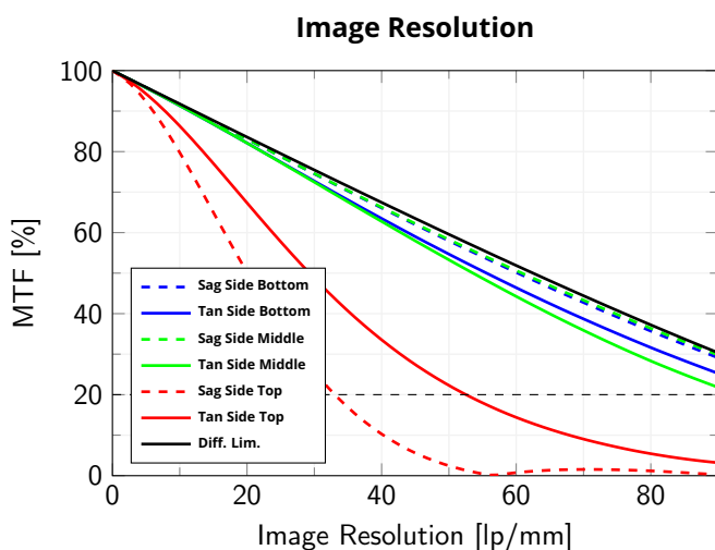
Modulation Transfer Function (MTF) vs. Image Resolution, wavelength range 486 nm - 656 nm of cylindrical object of diameter 50 mm and height of 150 mm at wf/N=11
