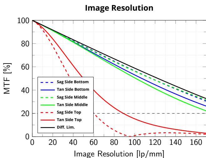
Modulation Transfer Function (MTF) vs. Image Resolution, wavelength range 486 nm - 656 nm of cylindrical object of diameter 50 mm and height of 150 mm at wf/N=5.6
