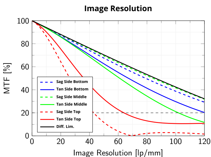
Modulation Transfer Function (MTF) vs. Image Resolution, wavelength range 486 nm - 656 nm of cylindrical object of diameter 50 mm and height of 150 mm at wf/N=8
