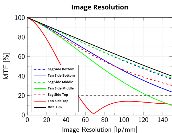
Modulation Transfer Function (MTF) vs. Image Resolution, wavelength range 486 nm - 656 nm of cylindrical object of diameter 110 mm and height of 330 mm at wf/N=5.6
