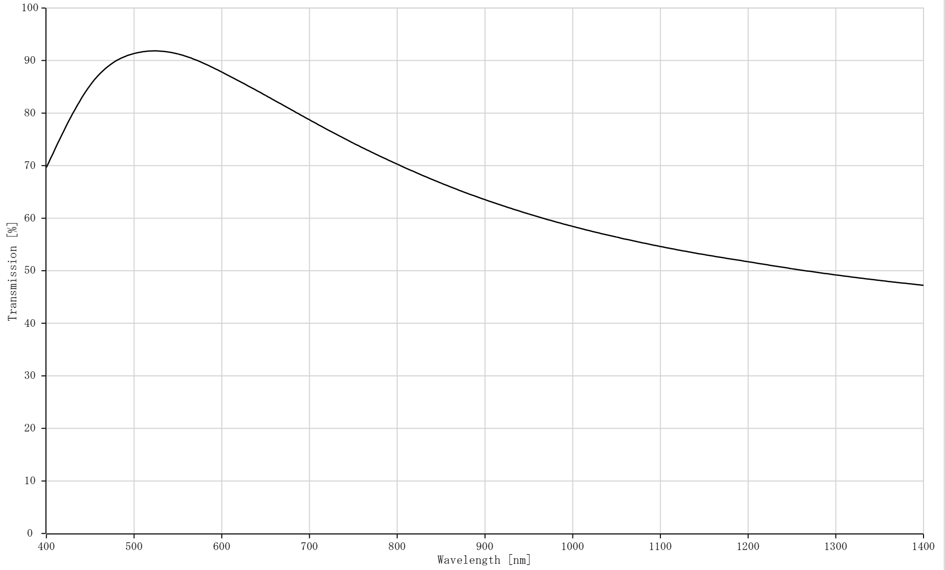
LM8JC5MC-WP Transmission
