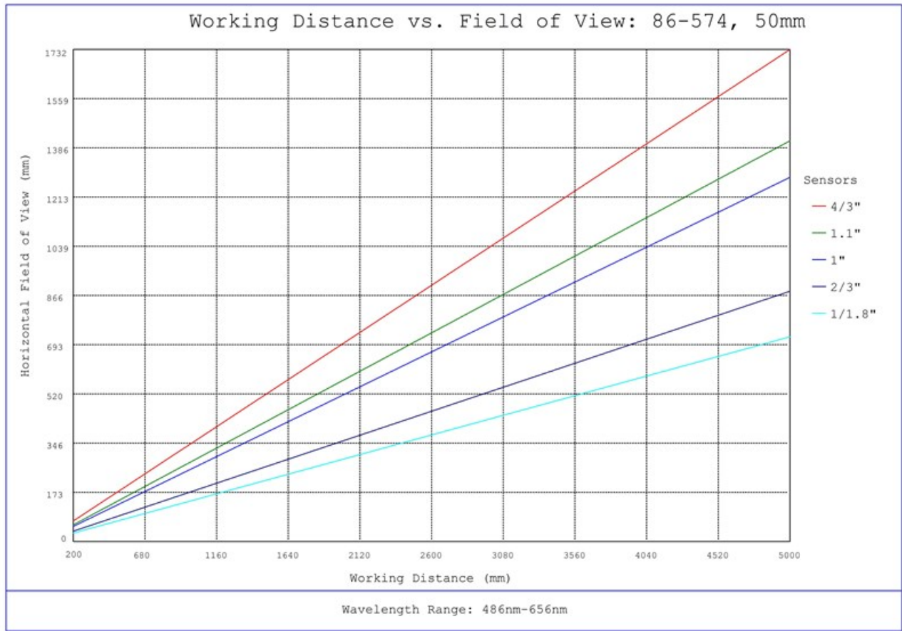
#86-574, 50mm Focal Length, HP Series Fixed Focal Length Lens, Working Distance versus Field of View Plot
