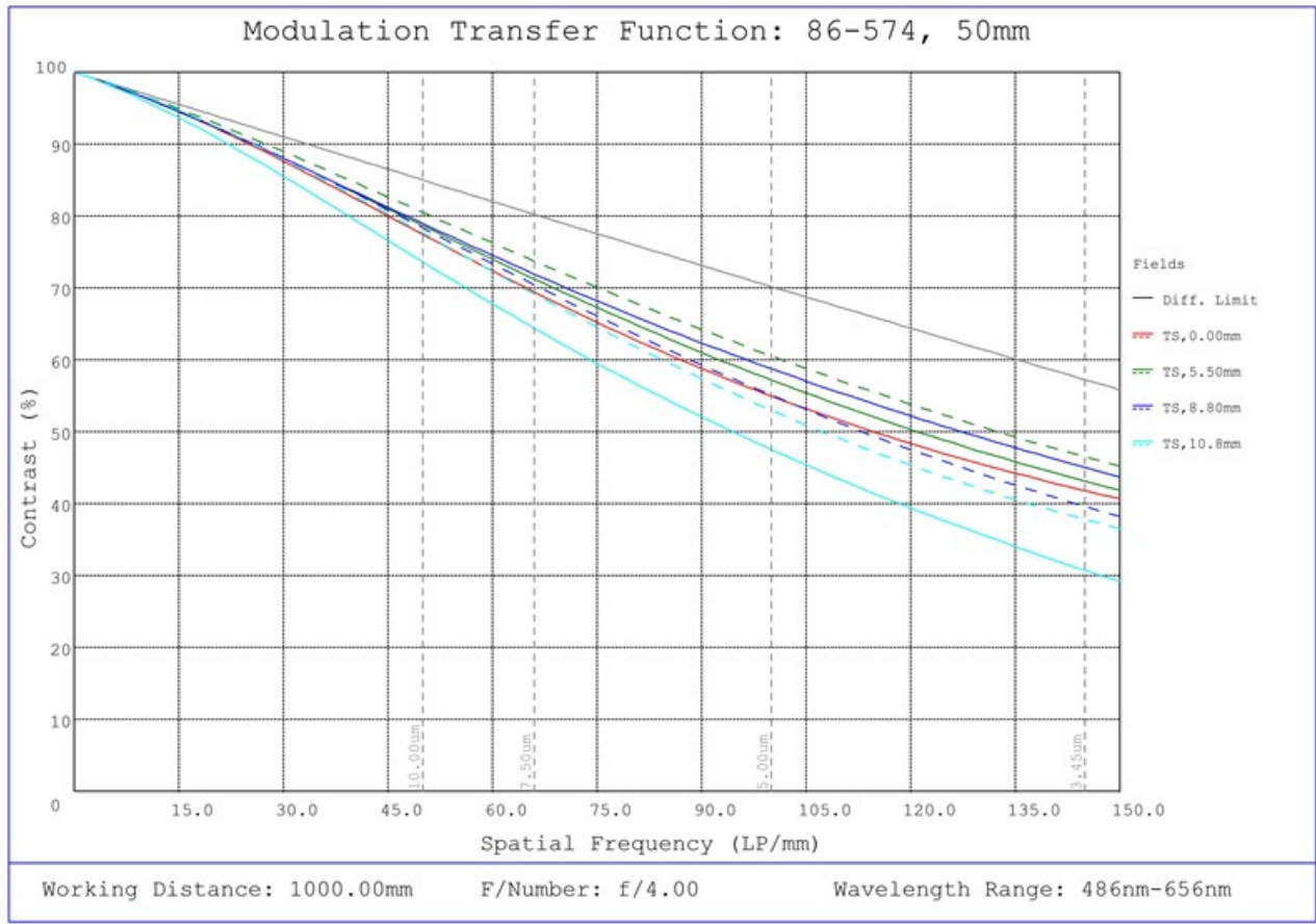
#86-574, 50mm Focal Length, HP Series Fixed Focal Length Lens, Modulated Transfer Function (MTF) Plot, 1000mm Working Distance, f4
