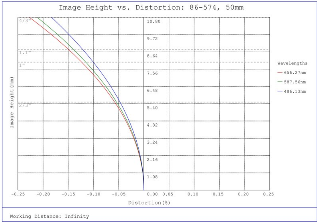
#86-574, 50mm Focal Length, HP Series Fixed Focal Length Lens, Distortion Plot
