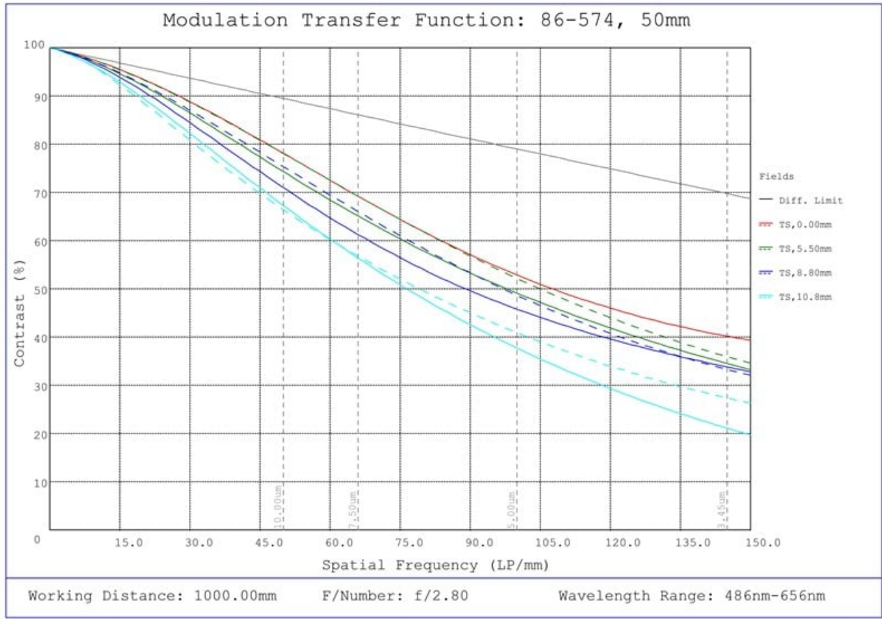
#86-574, 50mm Focal Length, HP Series Fixed Focal Length Lens, Modulated Transfer Function (MTF) Plot, 1000mm Working Distance, f2.8
