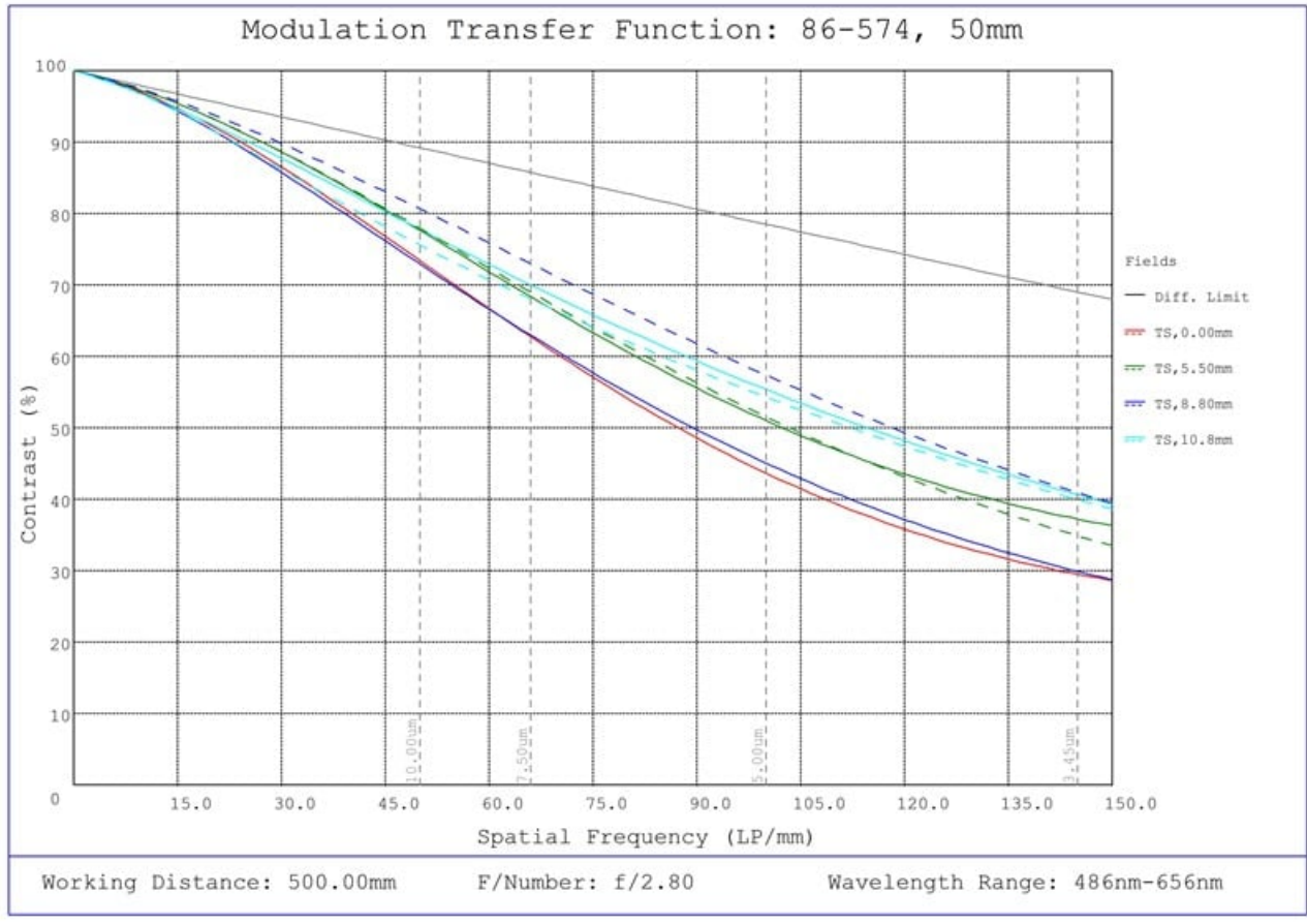
#86-574, 50mm Focal Length, HP Series Fixed Focal Length Lens, Modulated Transfer Function (MTF) Plot, 500mm Working Distance, f2.8
