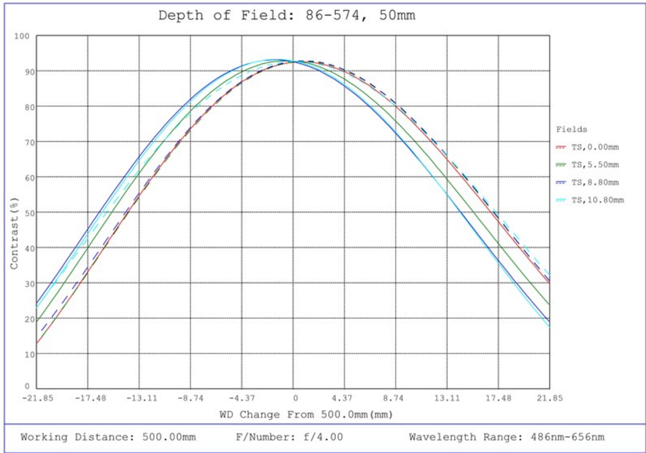
#86-574, 50mm Focal Length, HP Series Fixed Focal Length Lens, Depth of Field Plot, 500mm Working Distance, f4
