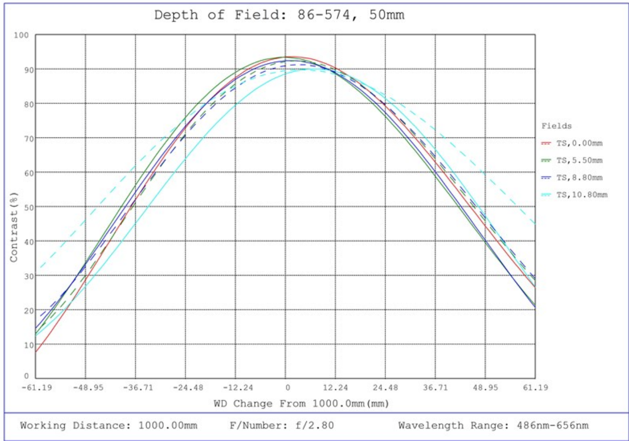
#86-574, 50mm Focal Length, HP Series Fixed Focal Length Lens, Depth of Field Plot, 1000mm Working Distance, f2.8
