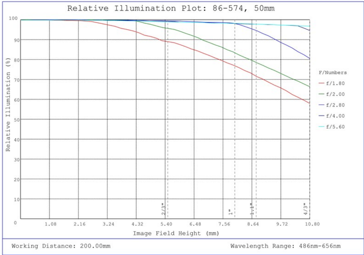
#86-574, 50mm Focal Length, HP Series Fixed Focal Length Lens, Relative Illumination Plot
