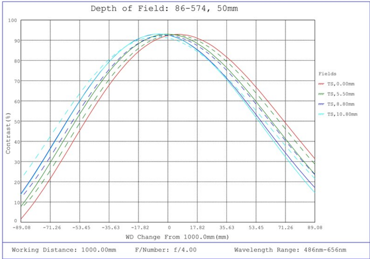
#86-574, 50mm Focal Length, HP Series Fixed Focal Length Lens, Depth of Field Plot, 1000mm Working Distance, f4
