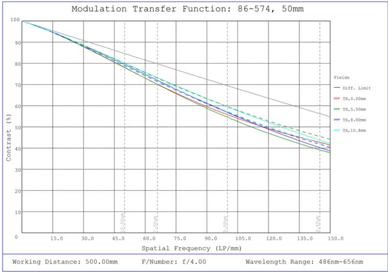
#86-574, 50mm Focal Length, HP Series Fixed Focal Length Lens, Modulated Transfer Function (MTF) Plot, 500mm Working Distance, f4
