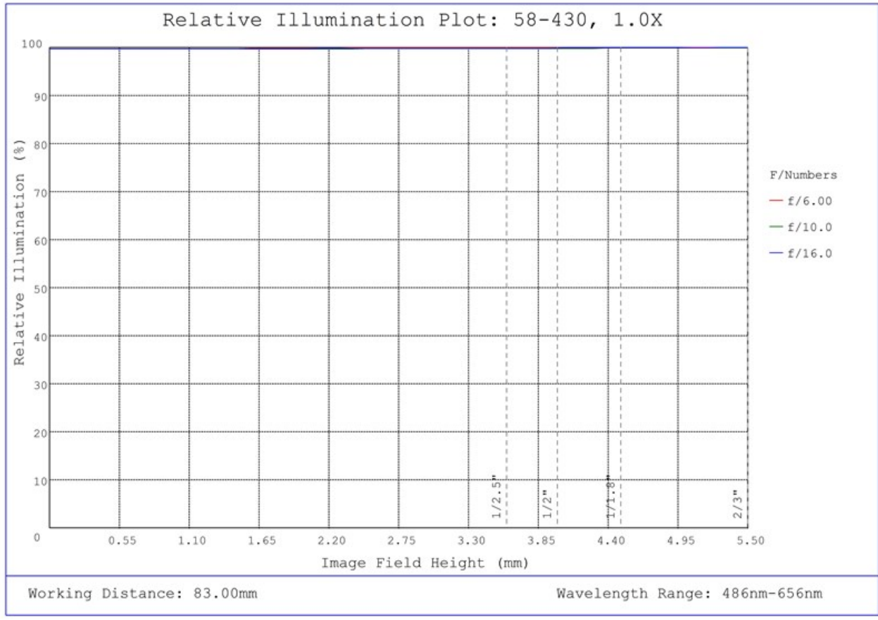
#58-430, 1.0X SilverTL™ Telecentric Lens, Relative Illumination Plot
