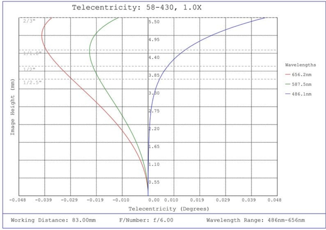
#58-430, 1.0X SilverTL™ Telecentric Lens, Telecentricity Plot
