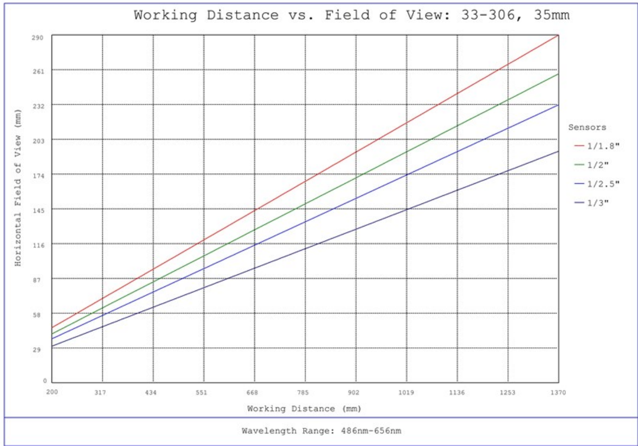
#33-306, 35mm UC Series Fixed Focal Length Lens, Working Distance versus Field of View Plot
