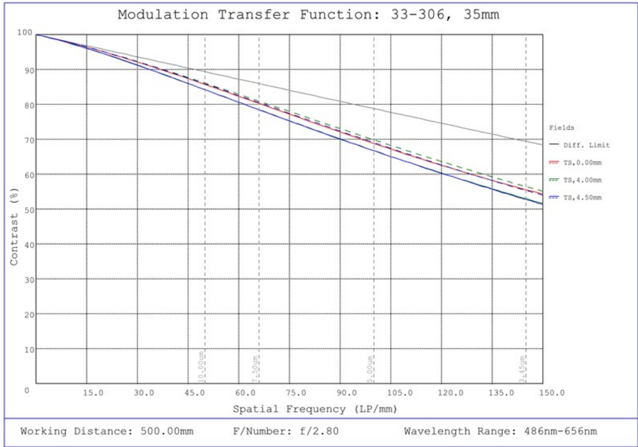
#33-306, 35mm UC Series Fixed Focal Length Lens, Modulated Transfer Function (MTF) Plot, 500mm Working Distance, f2.8
