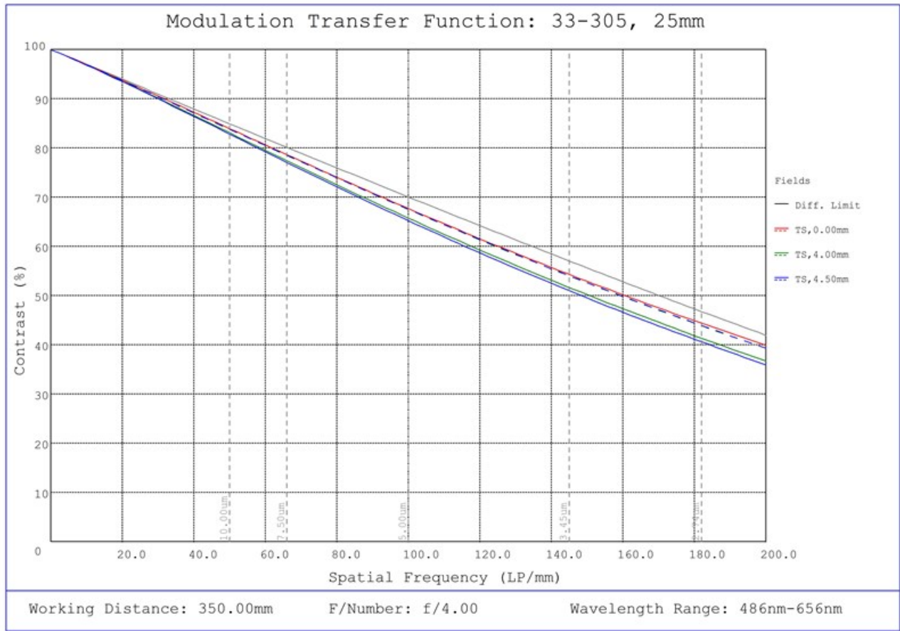
#33-305, 25mm UC Series Fixed Focal Length Lens, Modulated Transfer Function (MTF) Plot, 350mm Working Distance, f4
