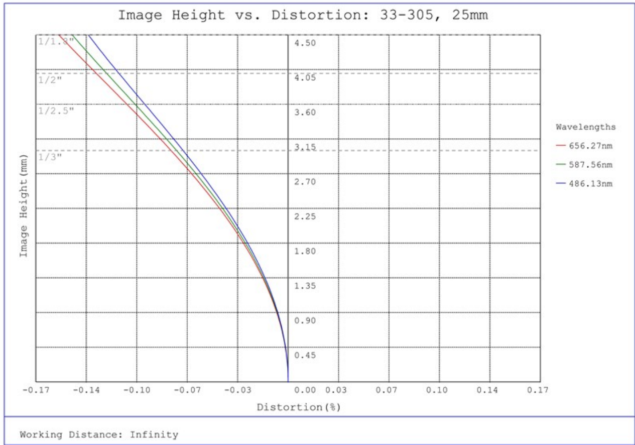
#33-305, 25mm UC Series Fixed Focal Length Lens, Distortion Plot
