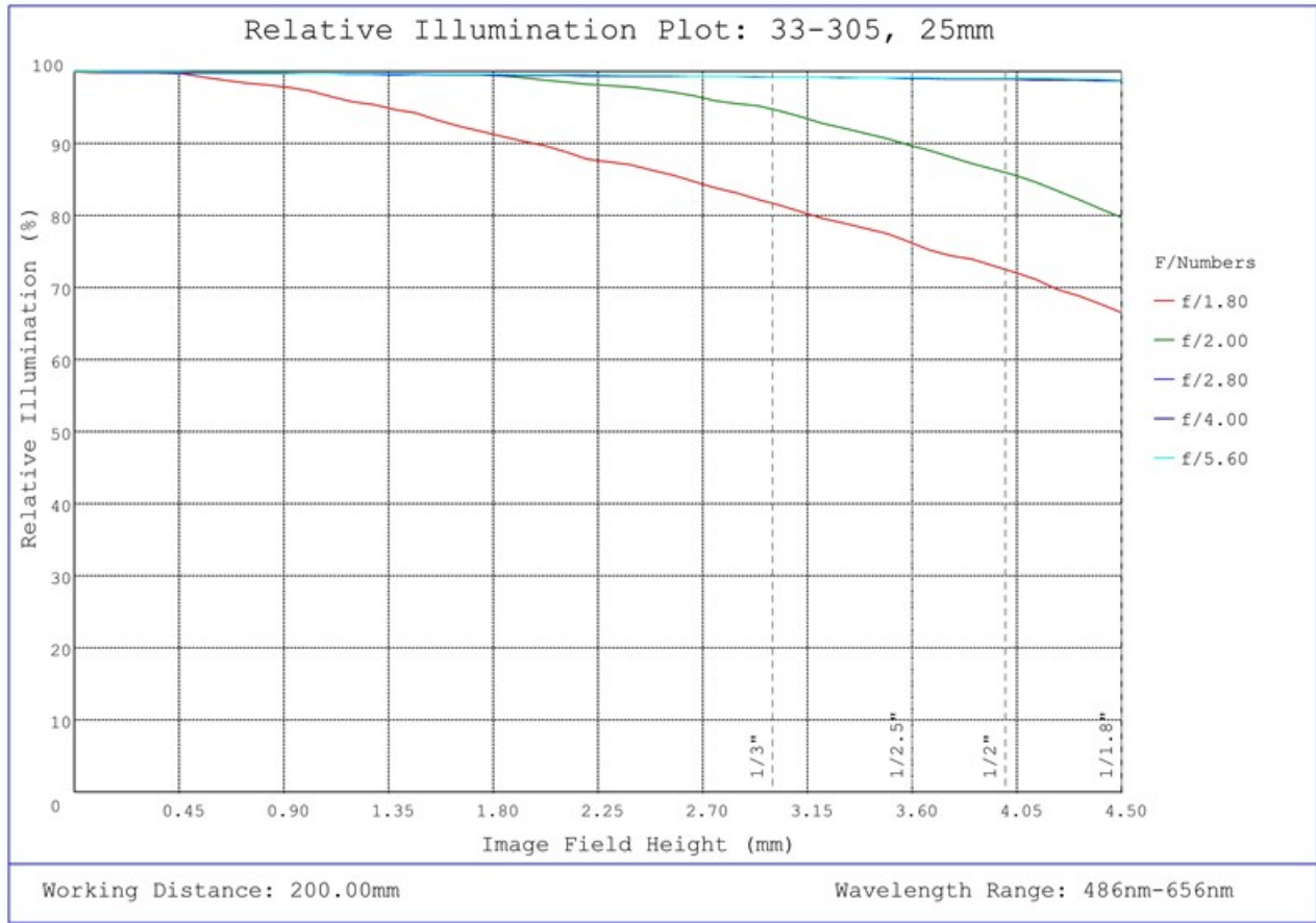
#33-305, 25mm UC Series Fixed Focal Length Lens, Relative Illumination Plot
