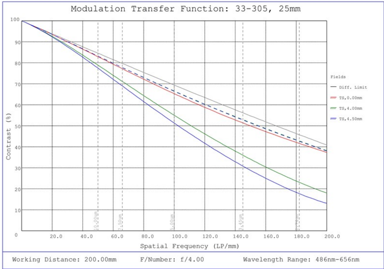
#33-305, 25mm UC Series Fixed Focal Length Lens, Modulated Transfer Function (MTF) Plot, 200mm Working Distance, f4
