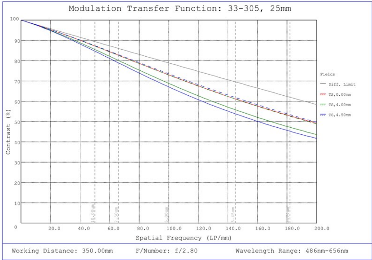
#33-305, 25mm UC Series Fixed Focal Length Lens, Modulated Transfer Function (MTF) Plot, 350mm Working Distance, f2.8
