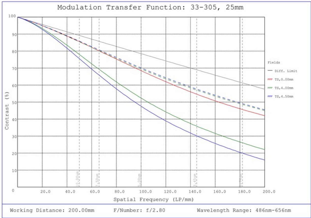
#33-305, 25mm UC Series Fixed Focal Length Lens, Modulated Transfer Function (MTF) Plot, 200mm Working Distance, f2.8
