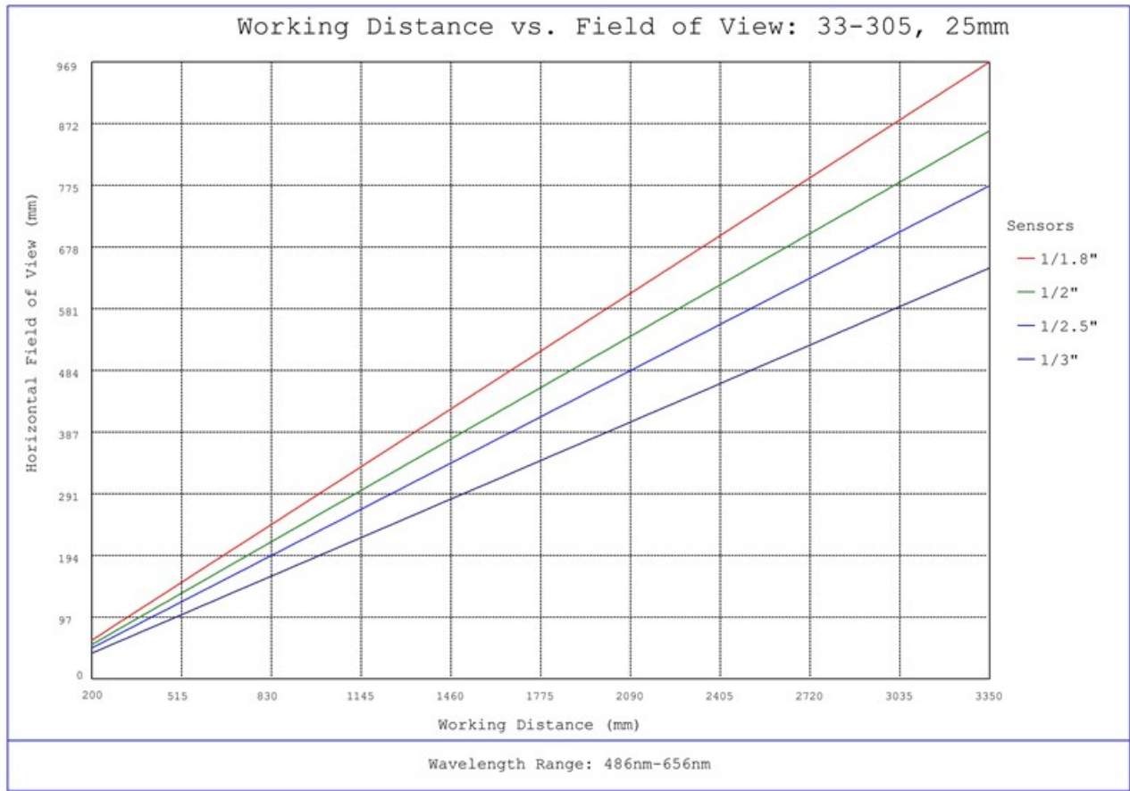
#33-305, 25mm UC Series Fixed Focal Length Lens, Working Distance versus Field of View Plot
