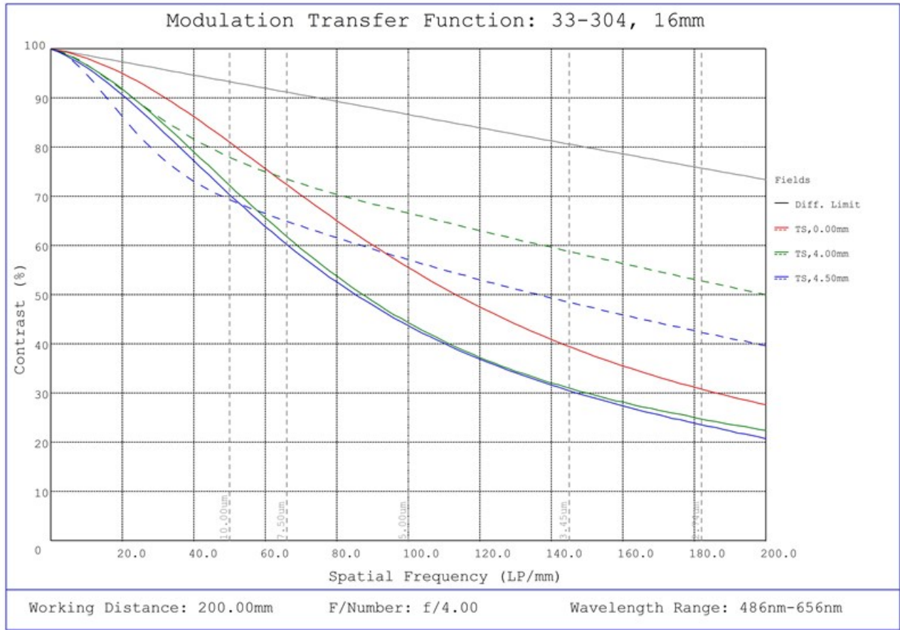
#33-304, 16mm UC Series Fixed Focal Length Lens, Modulated Transfer Function (MTF) Plot, 200mm Working Distance, f4
