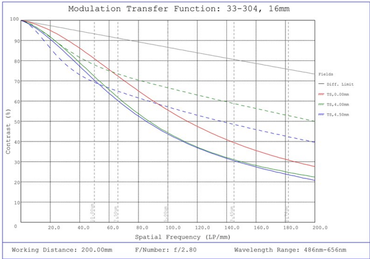
#33-304, 16mm UC Series Fixed Focal Length Lens, Modulated Transfer Function (MTF) Plot, 200mm Working Distance, f2.8
