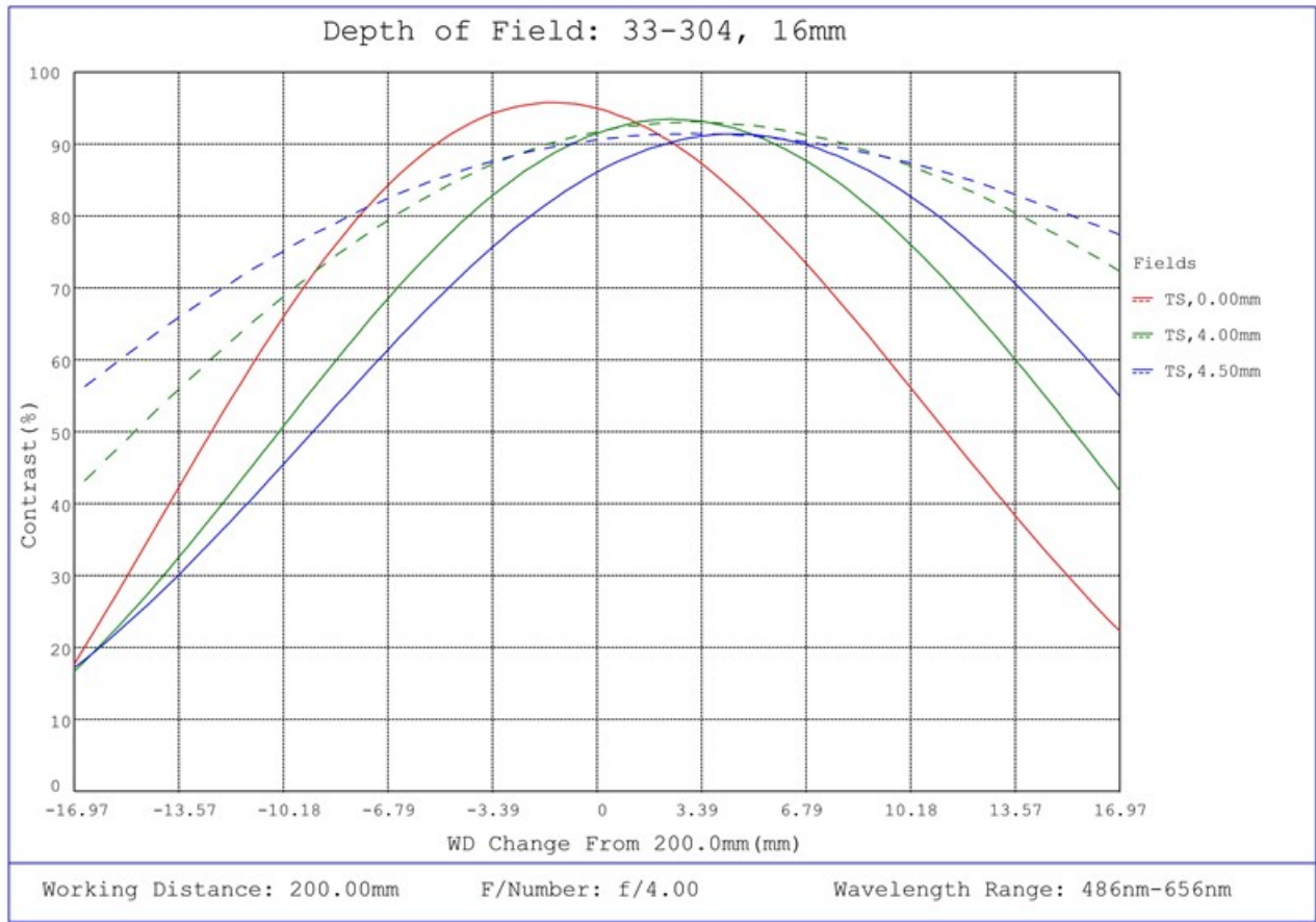
#33-304, 16mm UC Series Fixed Focal Length Lens, Depth of Field Plot, 200mm Working Distance, f4
