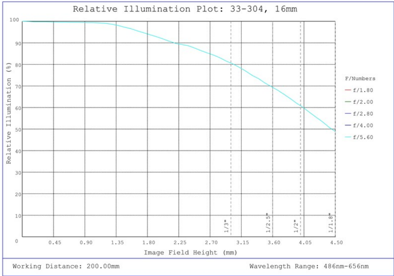
#33-304, 16mm UC Series Fixed Focal Length Lens, Relative Illumination Plot
