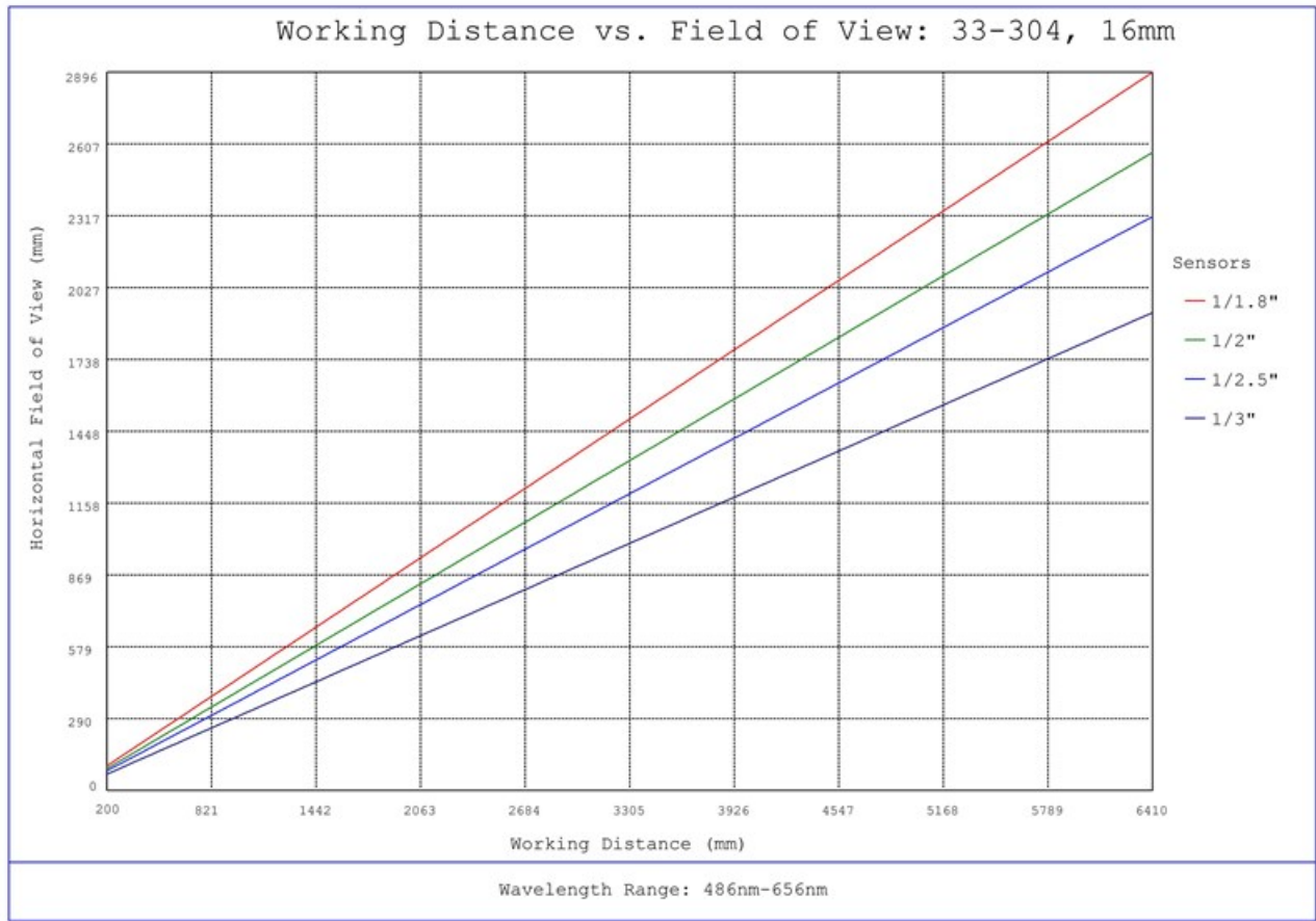
#33-304, 16mm UC Series Fixed Focal Length Lens, Working Distance versus Field of View Plot
