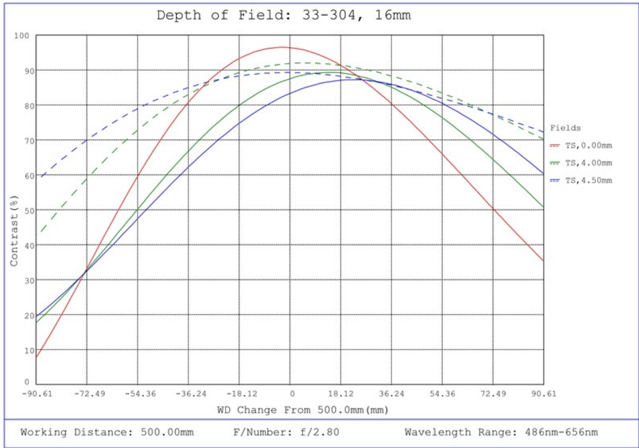
#33-304, 16mm UC Series Fixed Focal Length Lens, Depth of Field Plot, 500mm Working Distance, f2.8
