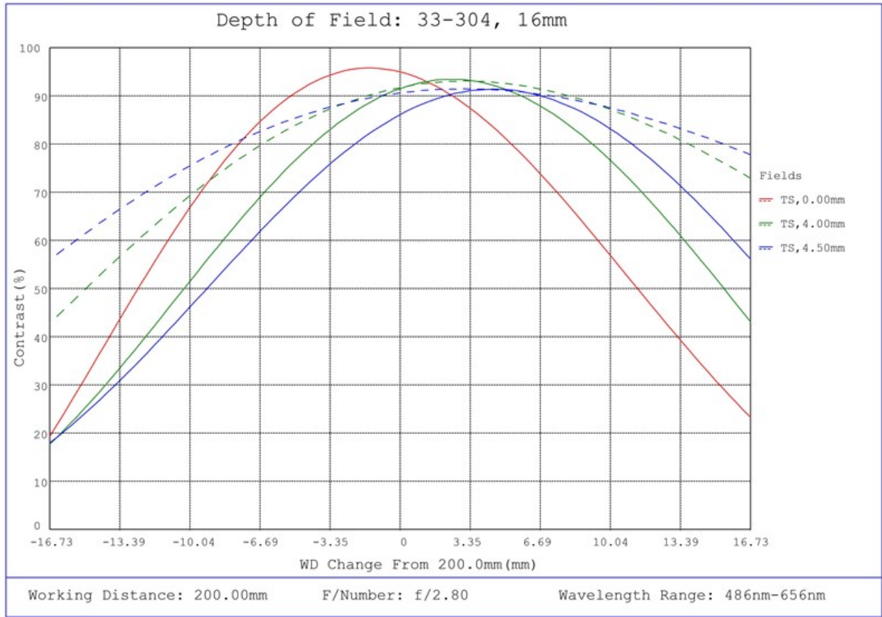
#33-304, 16mm UC Series Fixed Focal Length Lens, Depth of Field Plot, 200mm Working Distance, f2.8
