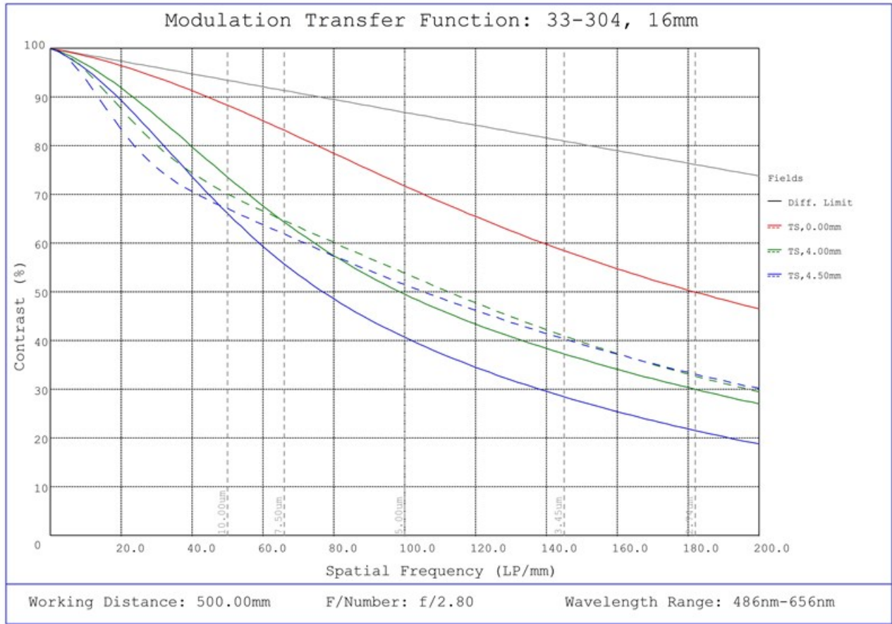
#33-304, 16mm UC Series Fixed Focal Length Lens, Modulated Transfer Function (MTF) Plot, 500mm Working Distance, f2.8
