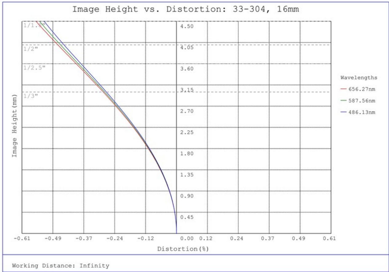
#33-304, 16mm UC Series Fixed Focal Length Lens, Distortion Plot
