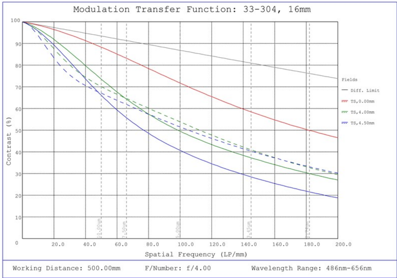
#33-304, 16mm UC Series Fixed Focal Length Lens, Modulated Transfer Function (MTF) Plot, 500mm Working Distance, f4
