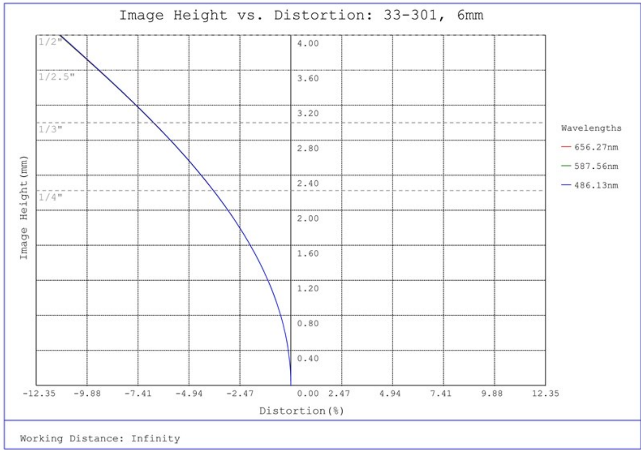
#33-301, 6mm UC Series Fixed Focal Length Lens, Distortion Plot
