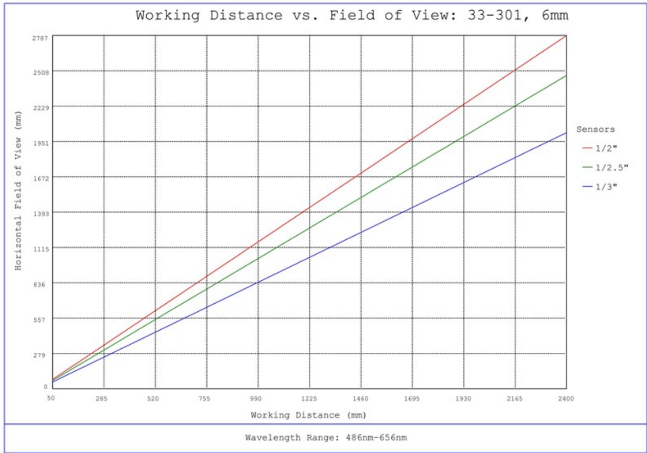
#33-301, 6mm UC Series Fixed Focal Length Lens, Working Distance versus Field of View Plot
