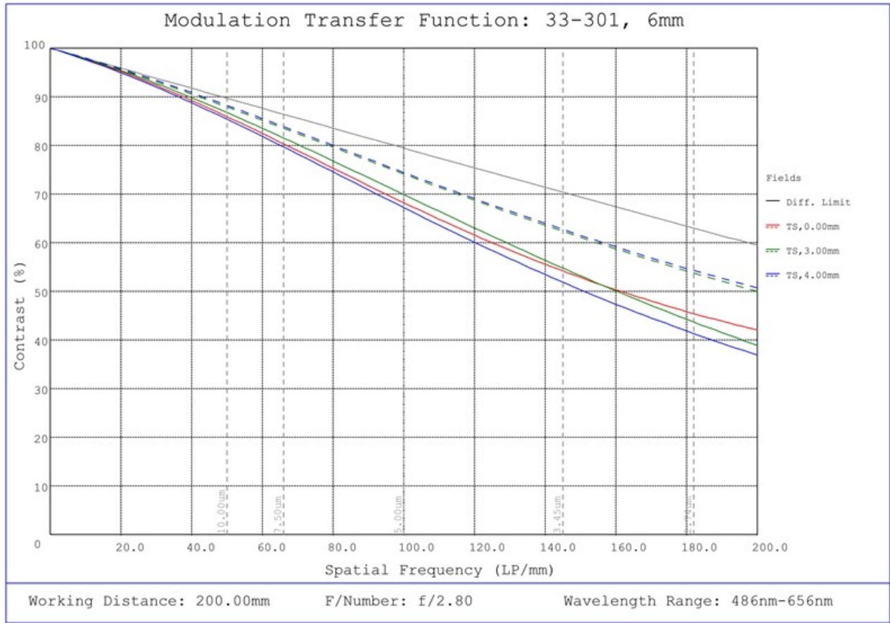
#33-301, 6mm UC Series Fixed Focal Length Lens, Modulated Transfer Function (MTF) Plot, 200mm Working Distance, f2.8
