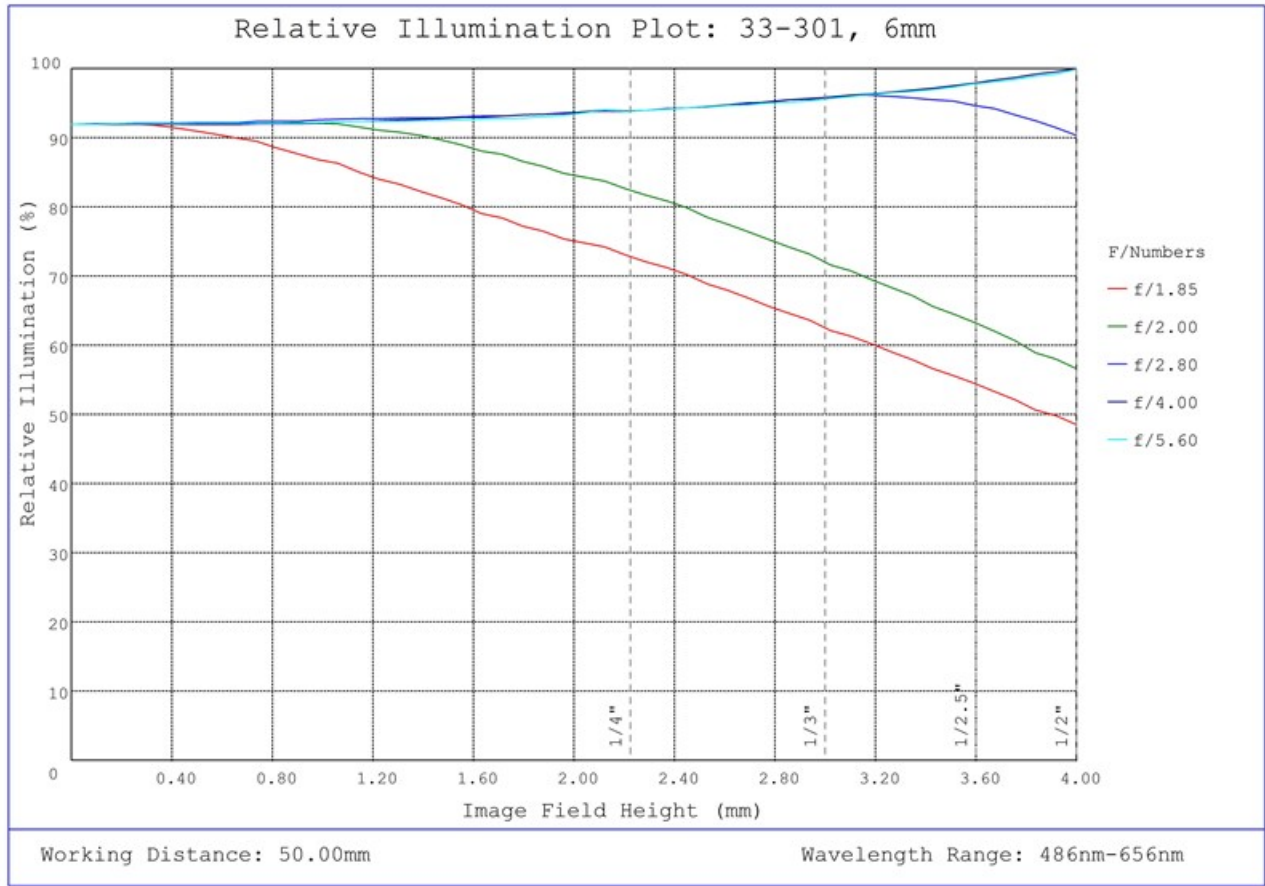
#33-301, 6mm UC Series Fixed Focal Length Lens, Relative Illumination Plot
