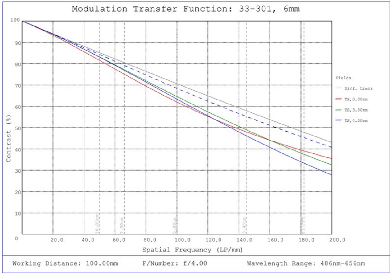
#33-301, 6mm UC Series Fixed Focal Length Lens, Modulated Transfer Function (MTF) Plot, 100mm Working Distance, f4
