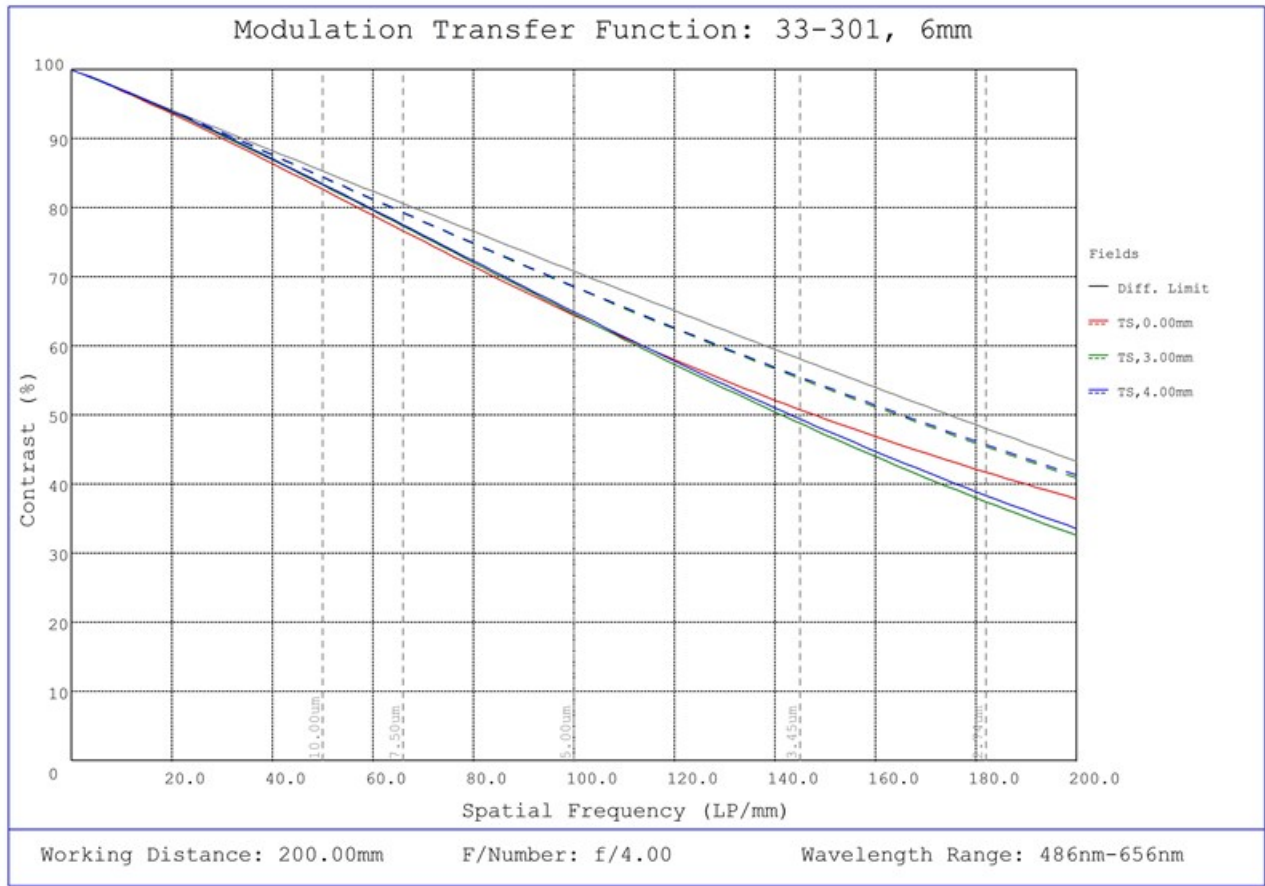
#33-301, 6mm UC Series Fixed Focal Length Lens, Modulated Transfer Function (MTF) Plot, 200mm Working Distance, f4
