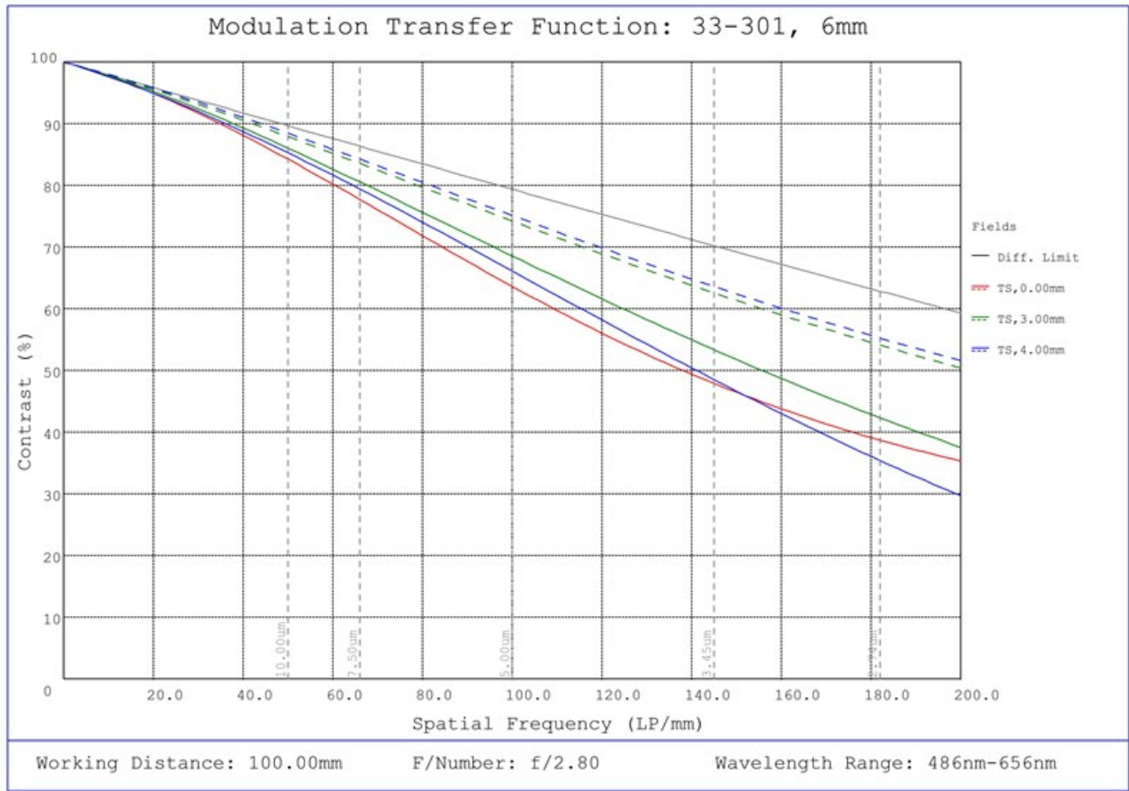
#33-301, 6mm UC Series Fixed Focal Length Lens, Modulated Transfer Function (MTF) Plot, 100mm Working Distance, f2.8
