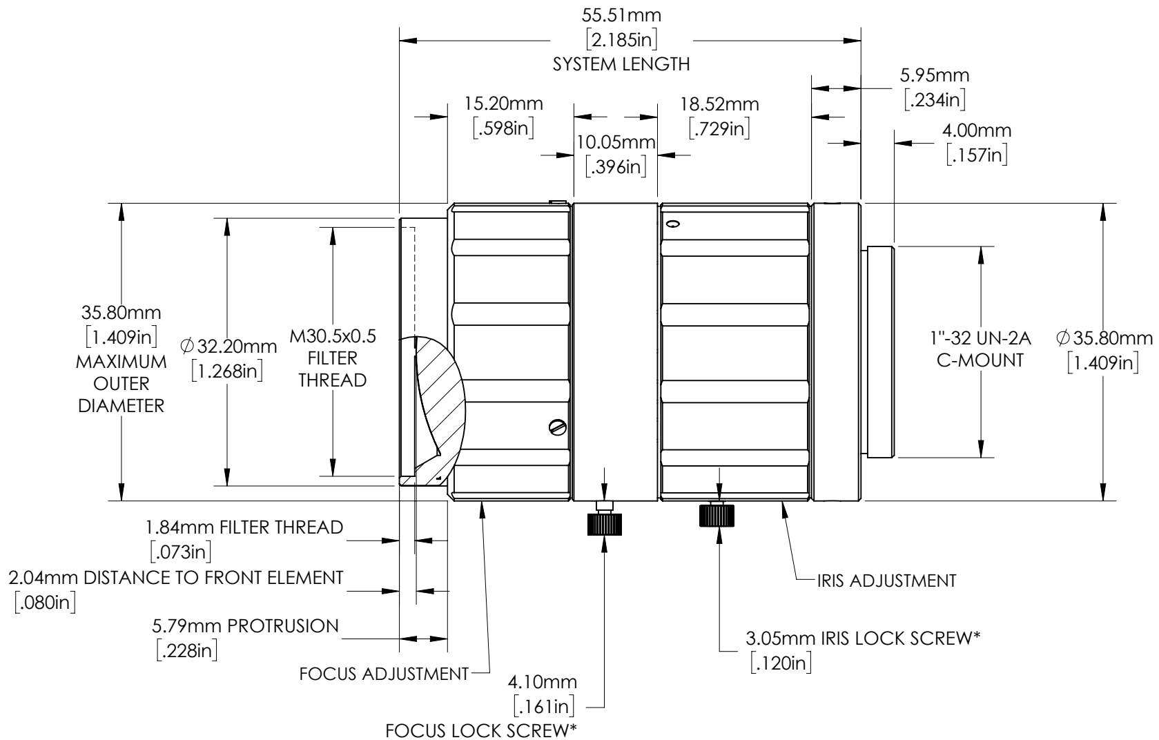
VIEW OF LENS FOCUSED TO 250mm WORKING DISTANCE
