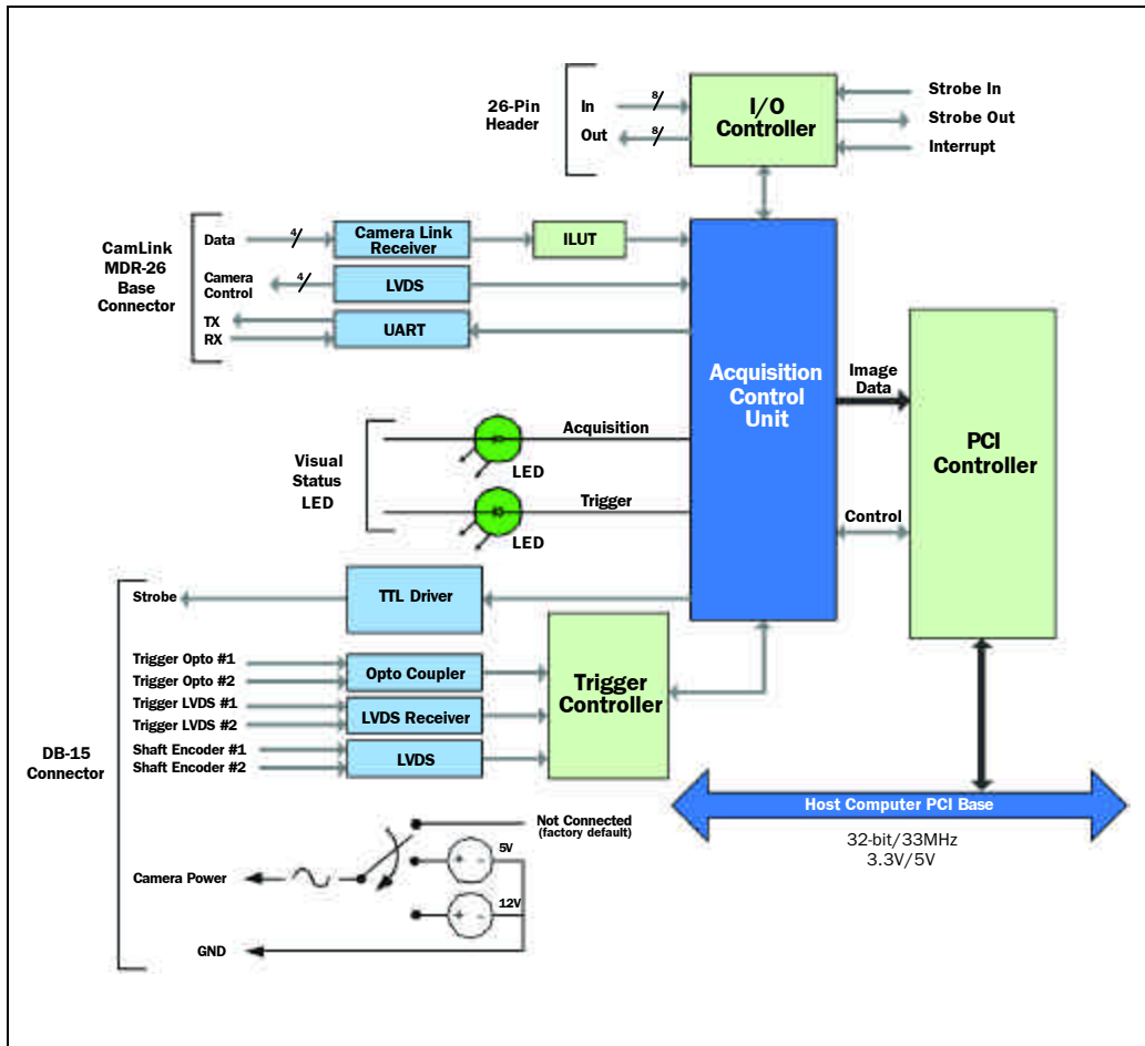
PC2-CamLink Functional Block Diagram
