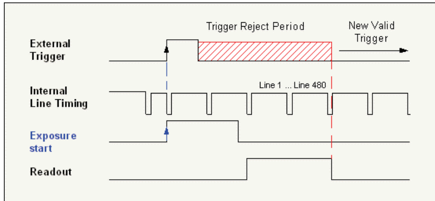
Reset Mode Timing example for Genie C640
