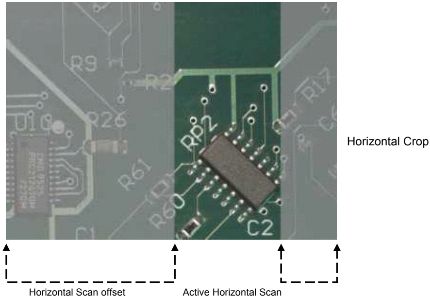
Horizontal Partial Scan Illustration
