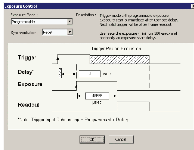
Programmable Reset Mode Exposure Timing
