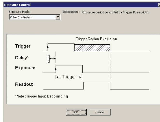
External Trigger Level-controlled Exposure Timing
