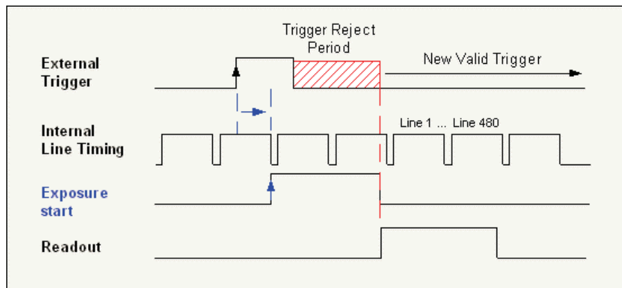
Synchronous Mode Timing example for Genie C640
