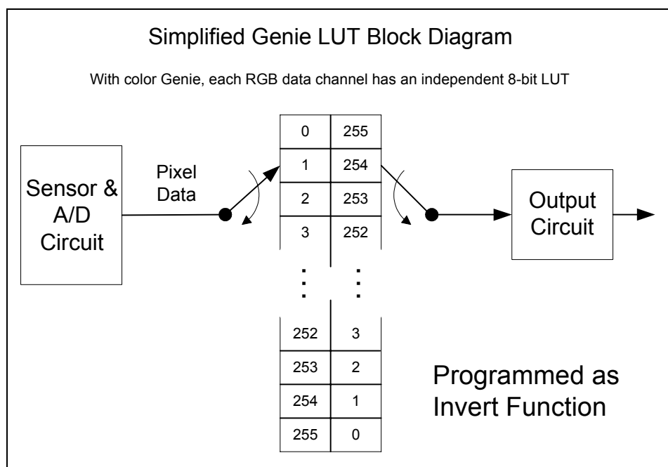
Simplified 8-bit LUT Block Diagram
