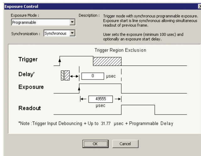
Programmable Synchronous Mode Exposure Timing
