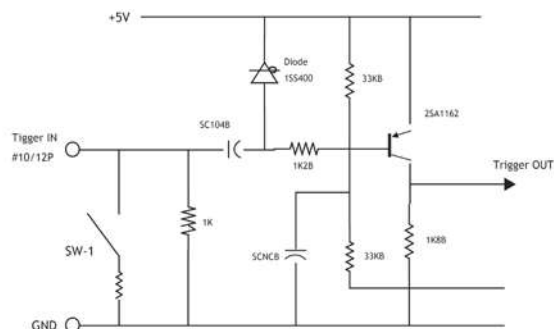
Fig. 4 Trigger input (12-pin)
