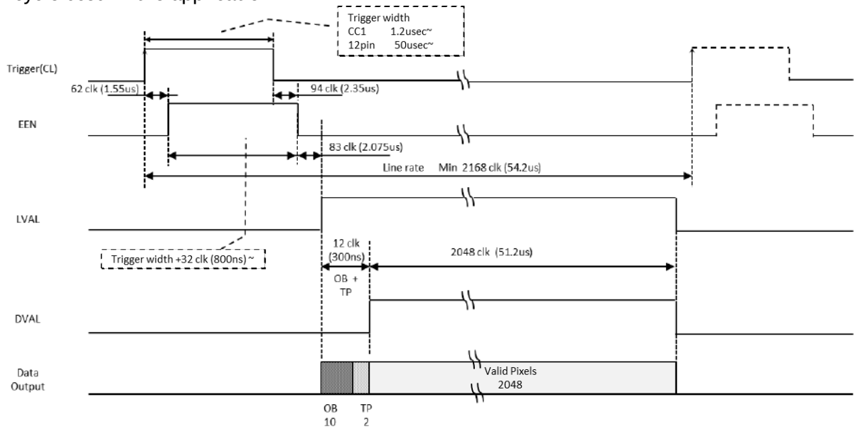
Fig. 13 Pulse Width Control mode
