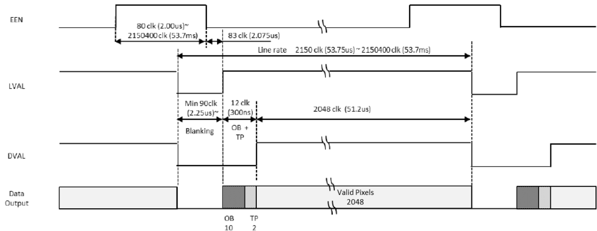
Fig. 11 Shutter-Select mode with Internal line rate generator (and individual exposure)
