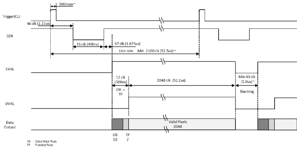
Fig. 10 No-Shutter mode with External Trigger
