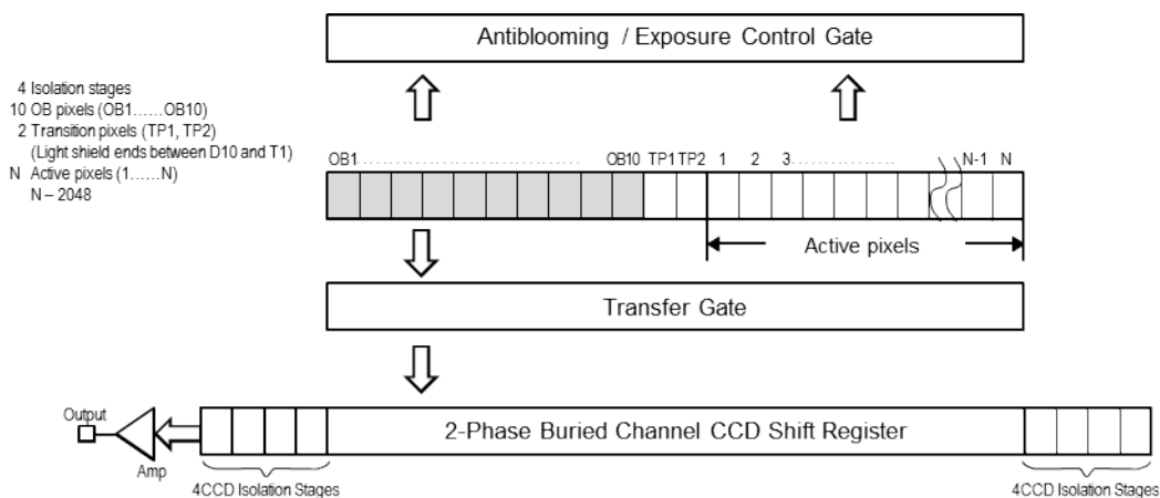
Fig. 7 Sensor block diagram
