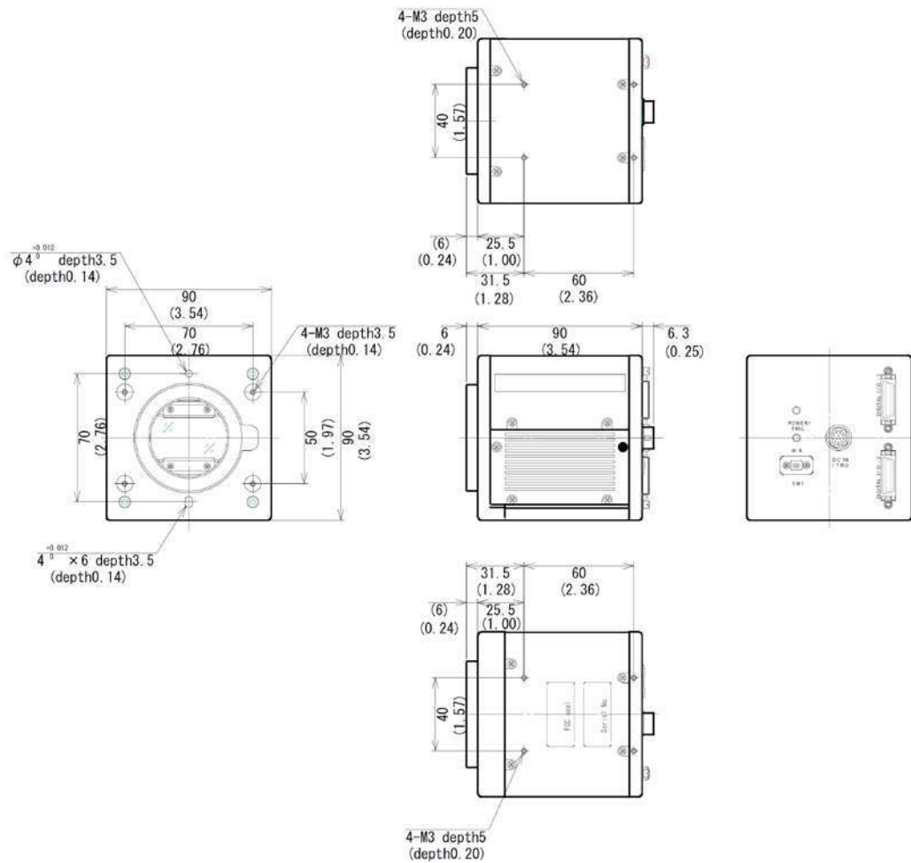
Fig.20 External Appearance and Dimensions
