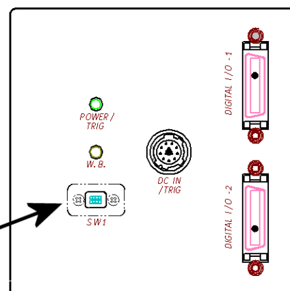
Fig. 15 Rear panel DIP-switch
