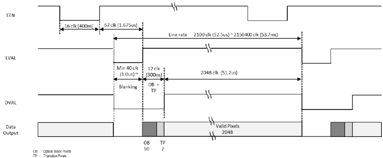
Fig. 9 No-Shutter mode with Internal line rate generator
