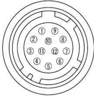
Fig. 2 12-pin connector
