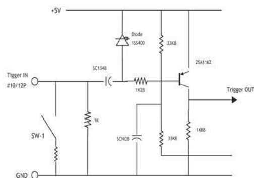
Fig. 6 Trigger input (12-pin Hirose)
