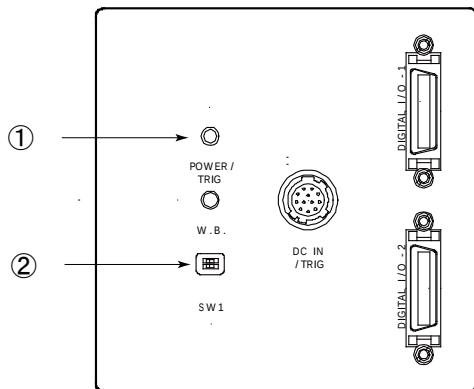
Fig2. Rear panel
