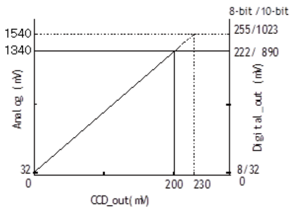
Fig.8 Video output
