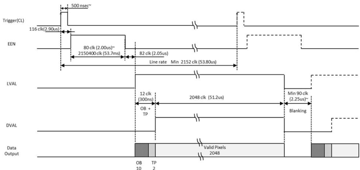
Fig. 15 Shutter-Select mode with external trigger (and individual exposure)
