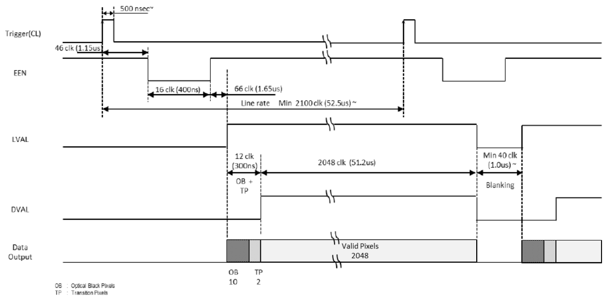
Fig. 13 No-Shutter mode with external trigger
