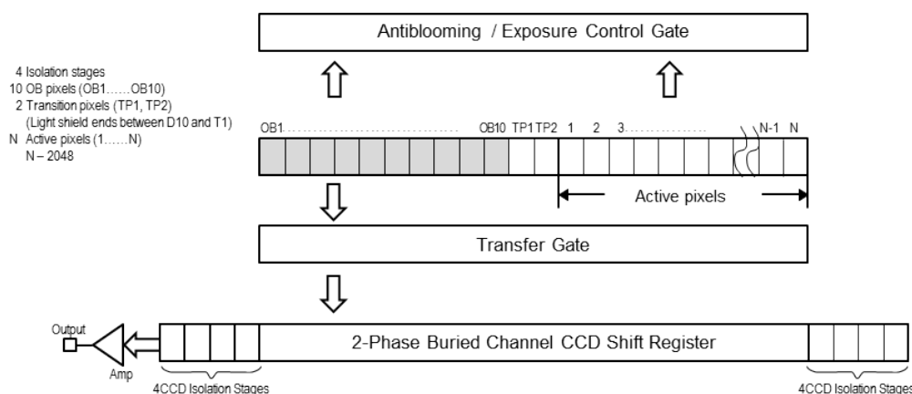
Fig.10 Sensor layout
