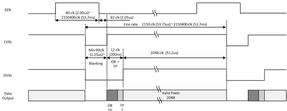
Fig. 14 Shutter-Select mode with internal line rate generator (and individual exposure)
