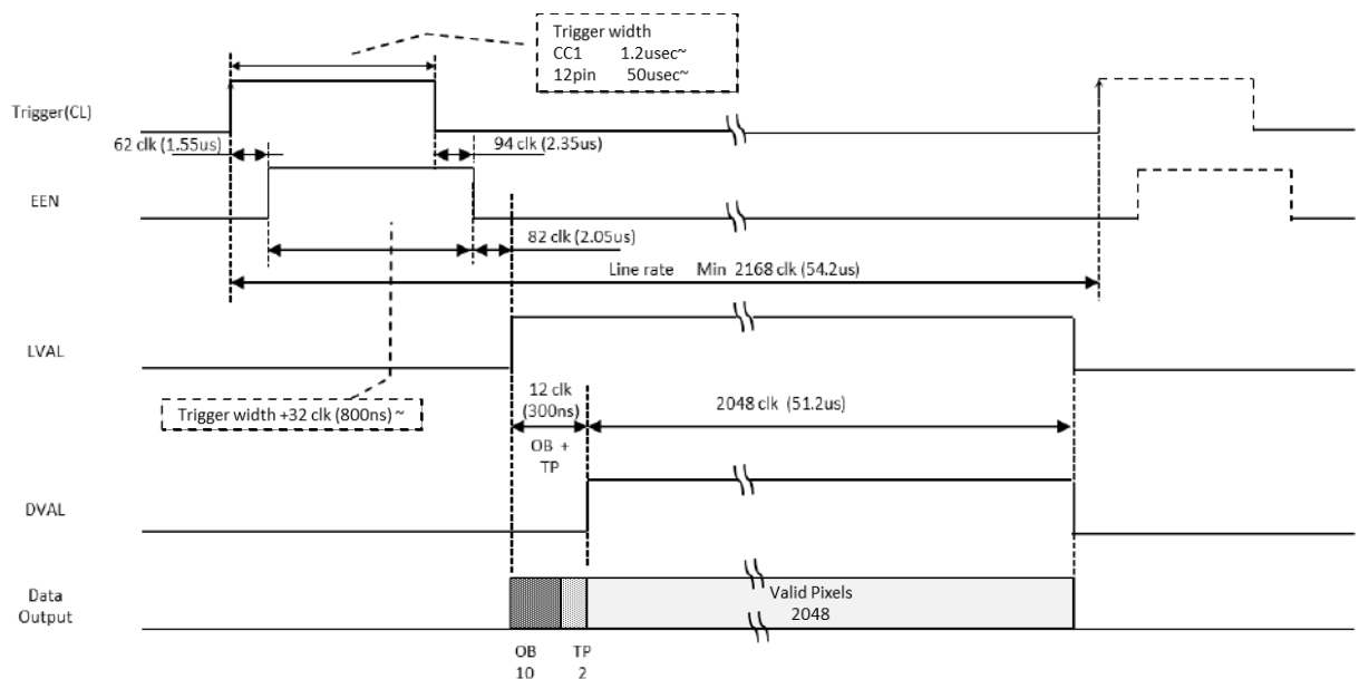
Fig. 16 Pulse Width Control mode
