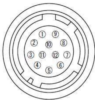
Fig. 4 12-pin connector
