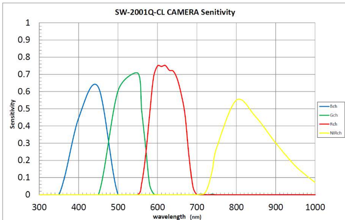
Fig. 27 Camera Spectral sensitivity
