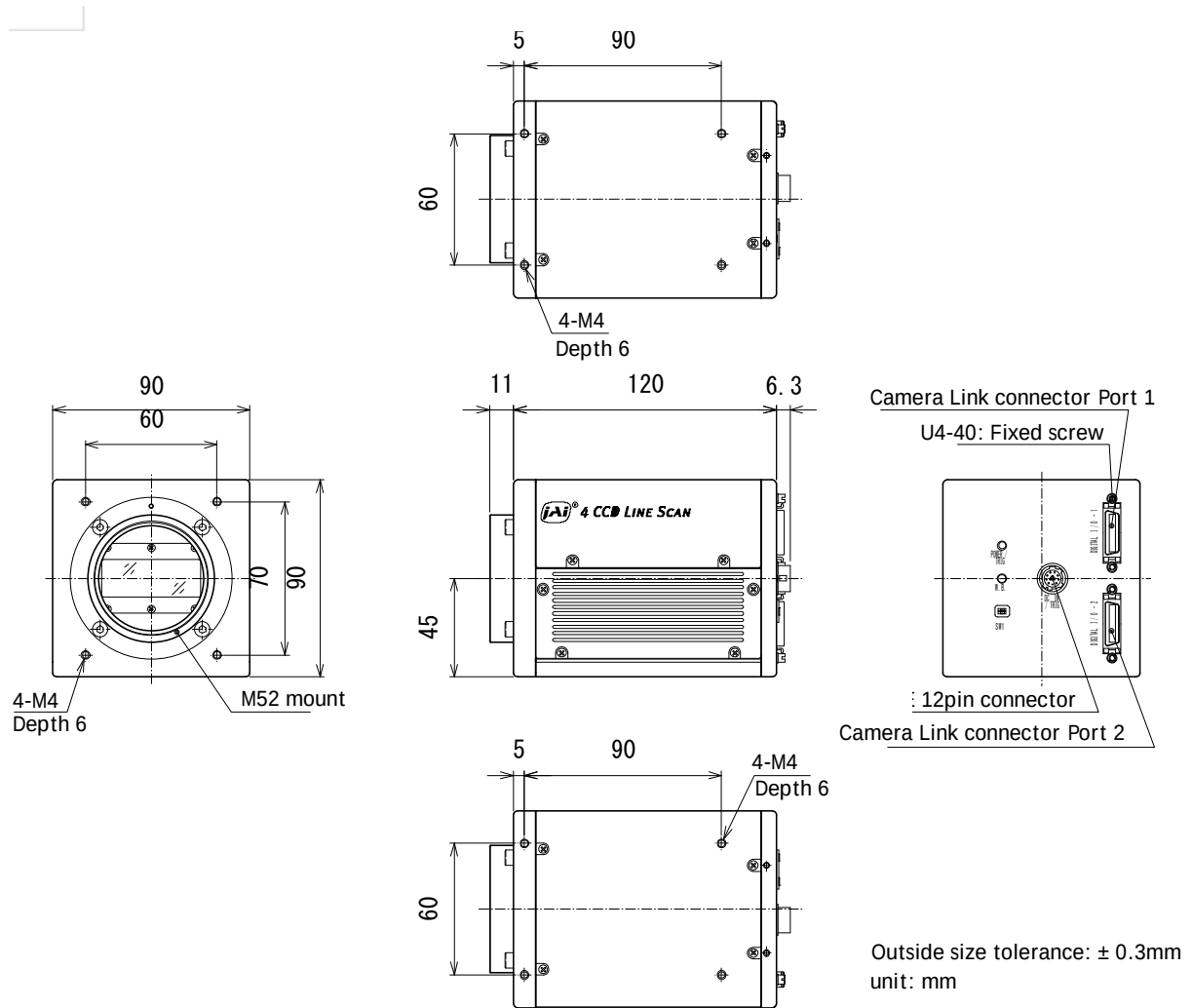
Fig.26 External Appearance and Dimensions
