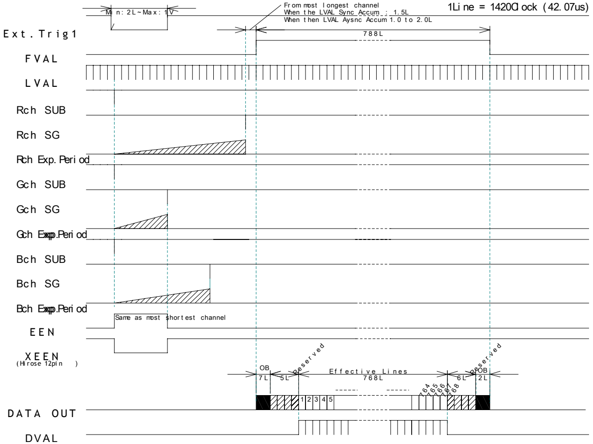
Fig. 27. Edge pre-select. LVAL synchronized.
