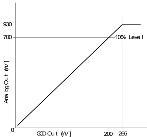
Fig.14 Lens Iris Analogue output
