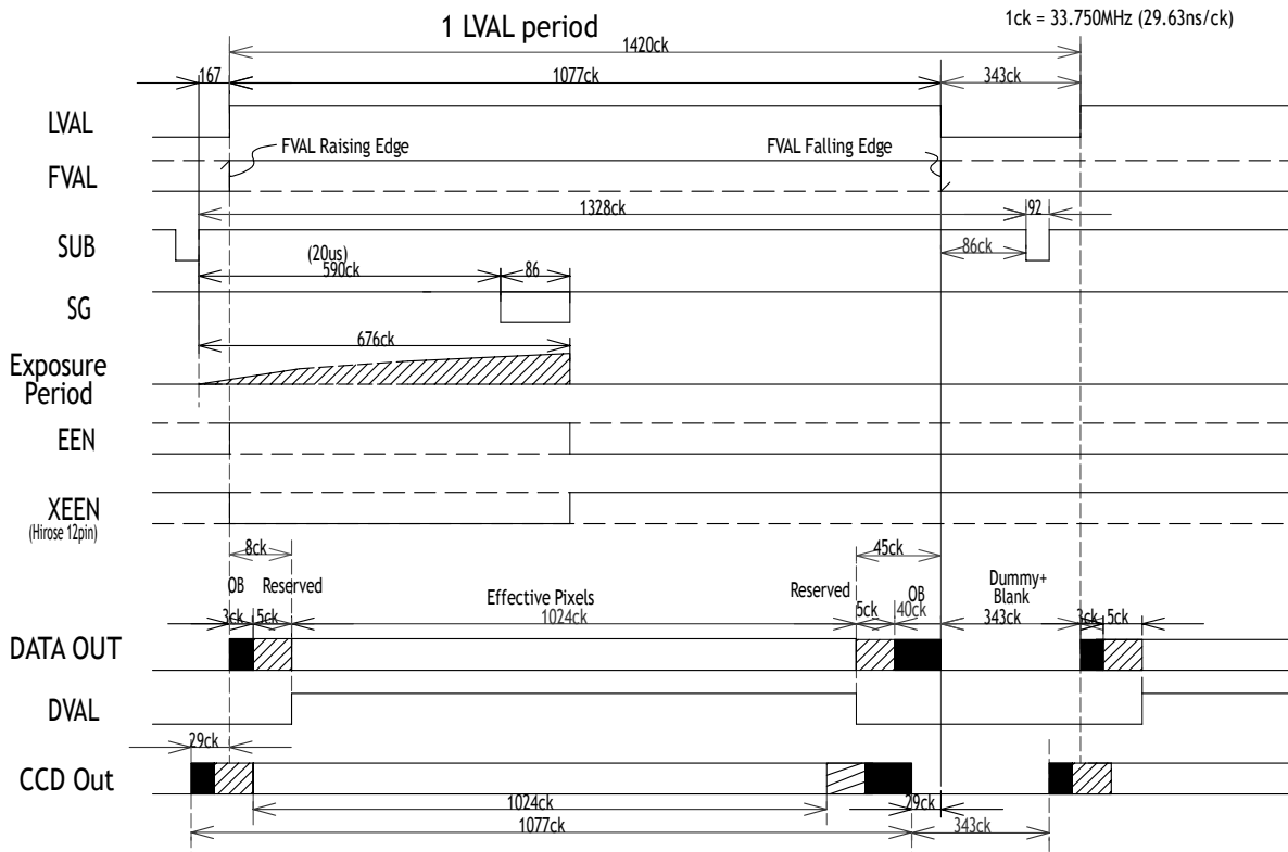
Fig. 16. Horizontal timing
