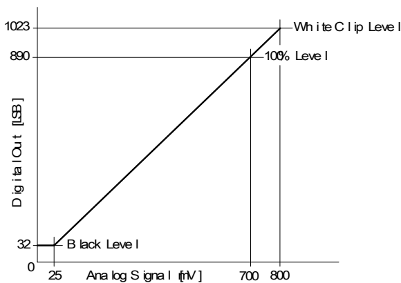
Fig.8 Digital Output
