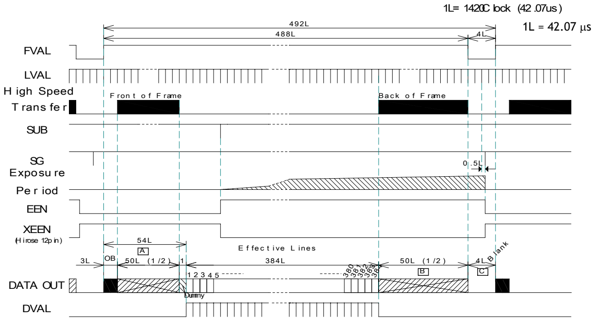
Fig. 18 Vertical timing for 1/2 partial scan
