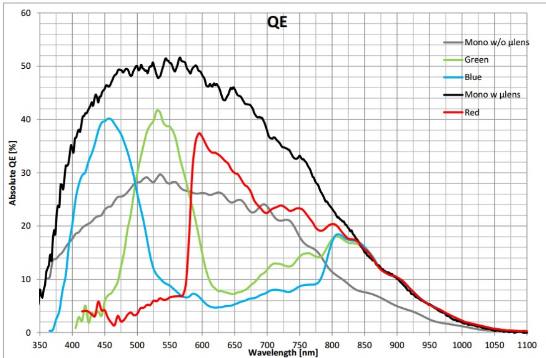
Typical QE of a CHR70M
