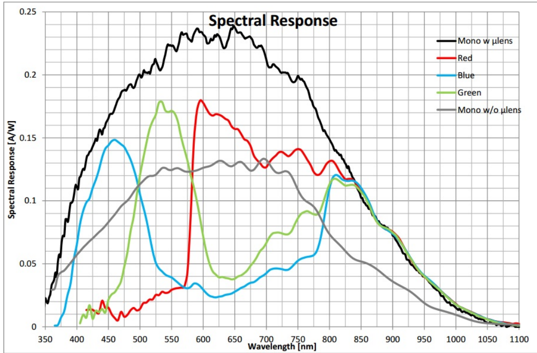
Typical spectral response of a CHR70M
