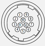
Hirose 12 Pin
