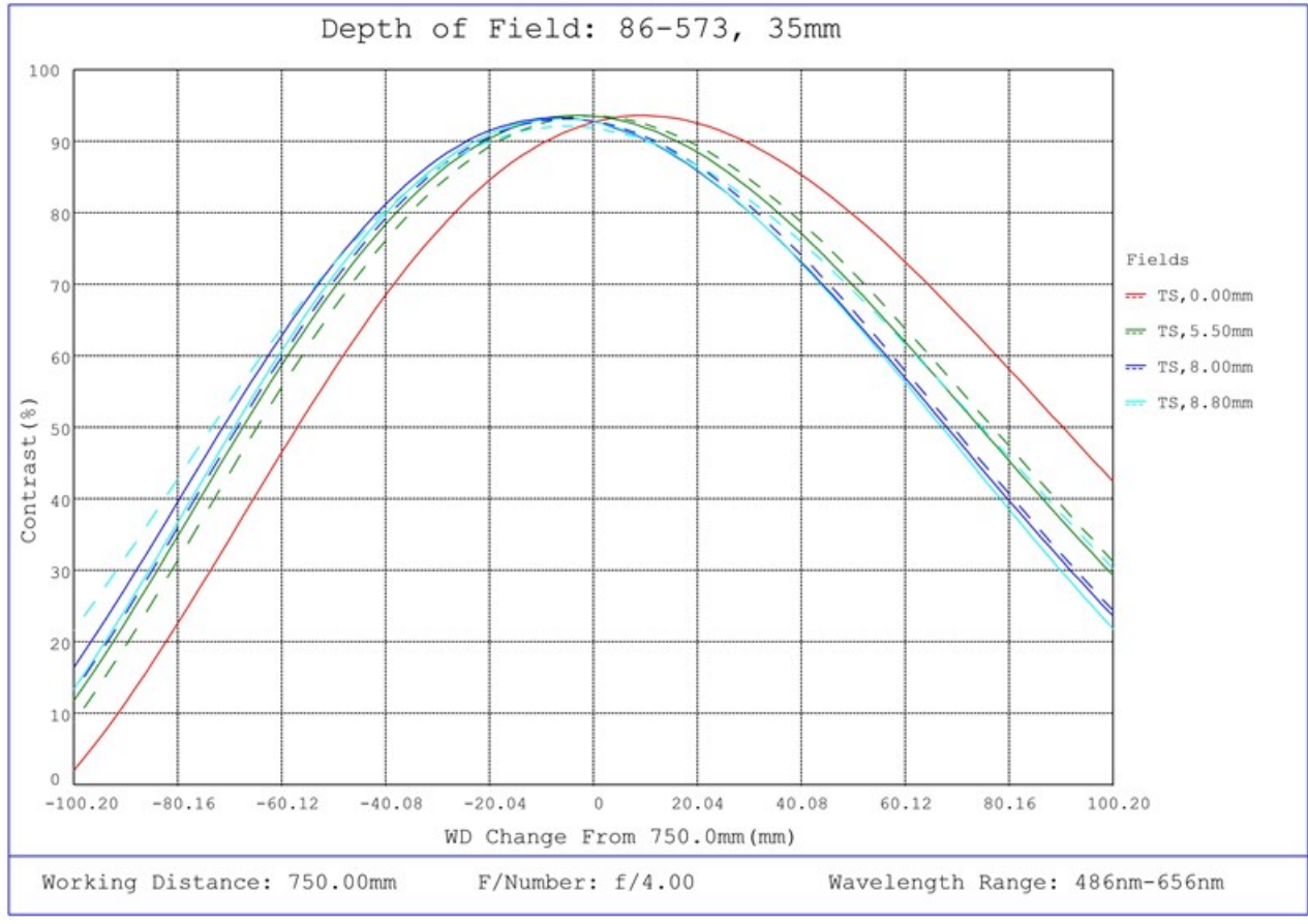
#86-573, 35mm Focal Length, HP Series Fixed Focal Length Lens, Depth of Field Plot, 750mm Working Distance, f4
