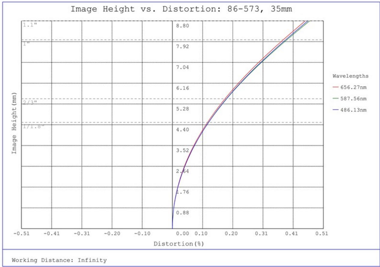
#86-573, 35mm Focal Length, HP Series Fixed Focal Length Lens, Distortion Plot
