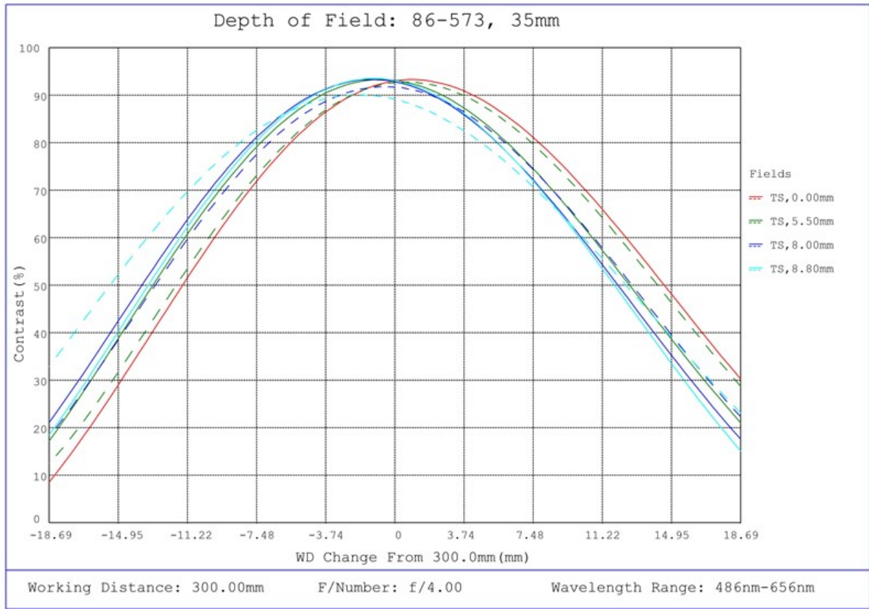
#86-573, 35mm Focal Length, HP Series Fixed Focal Length Lens, Depth of Field Plot, 300mm Working Distance, f4
