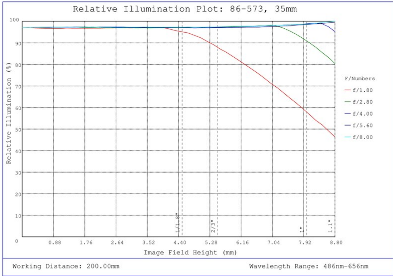
#86-573, 35mm Focal Length, HP Series Fixed Focal Length Lens, Relative Illumination Plot
