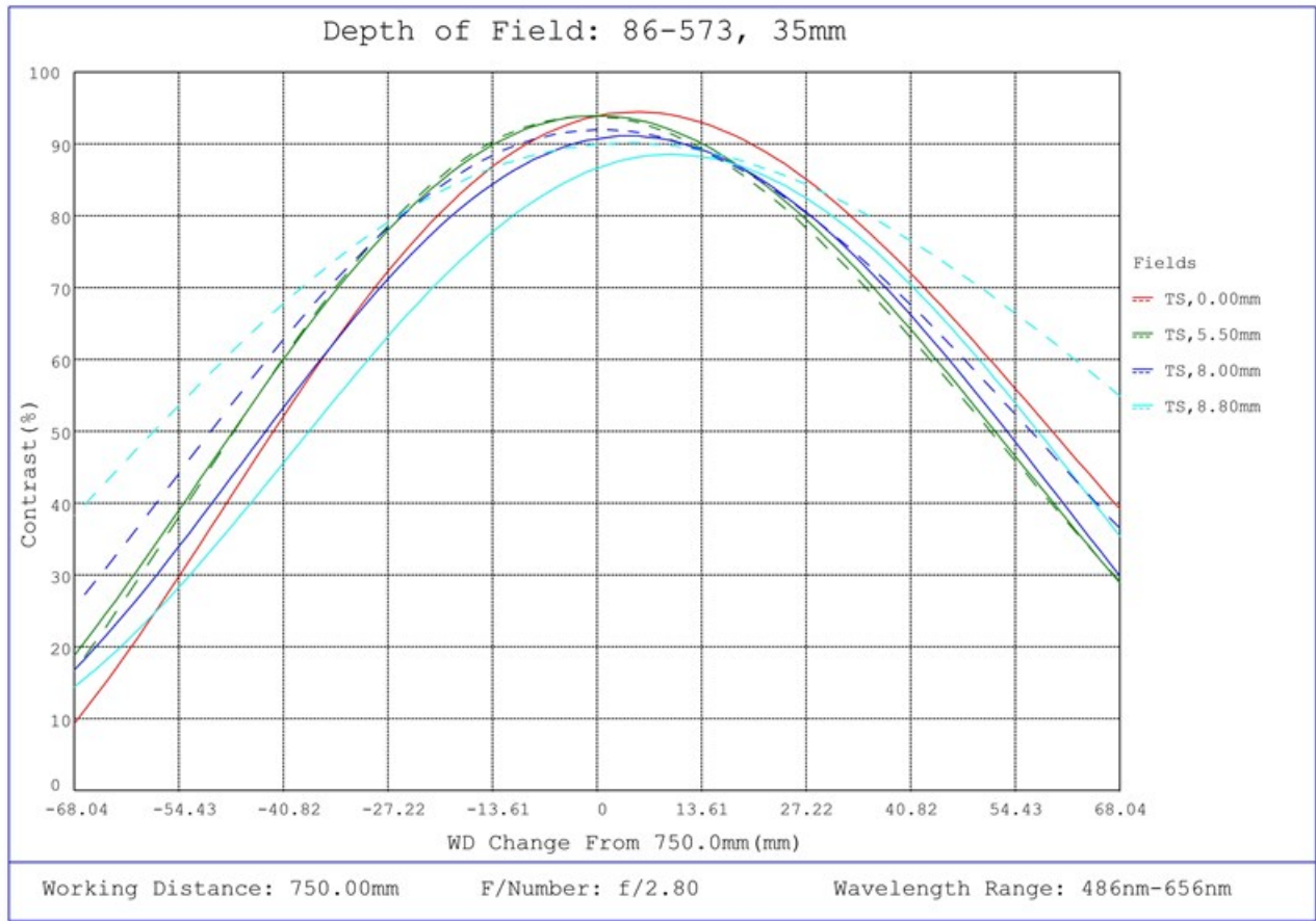
#86-573, 35mm Focal Length, HP Series Fixed Focal Length Lens, Depth of Field Plot, 750mm Working Distance, f2.8
