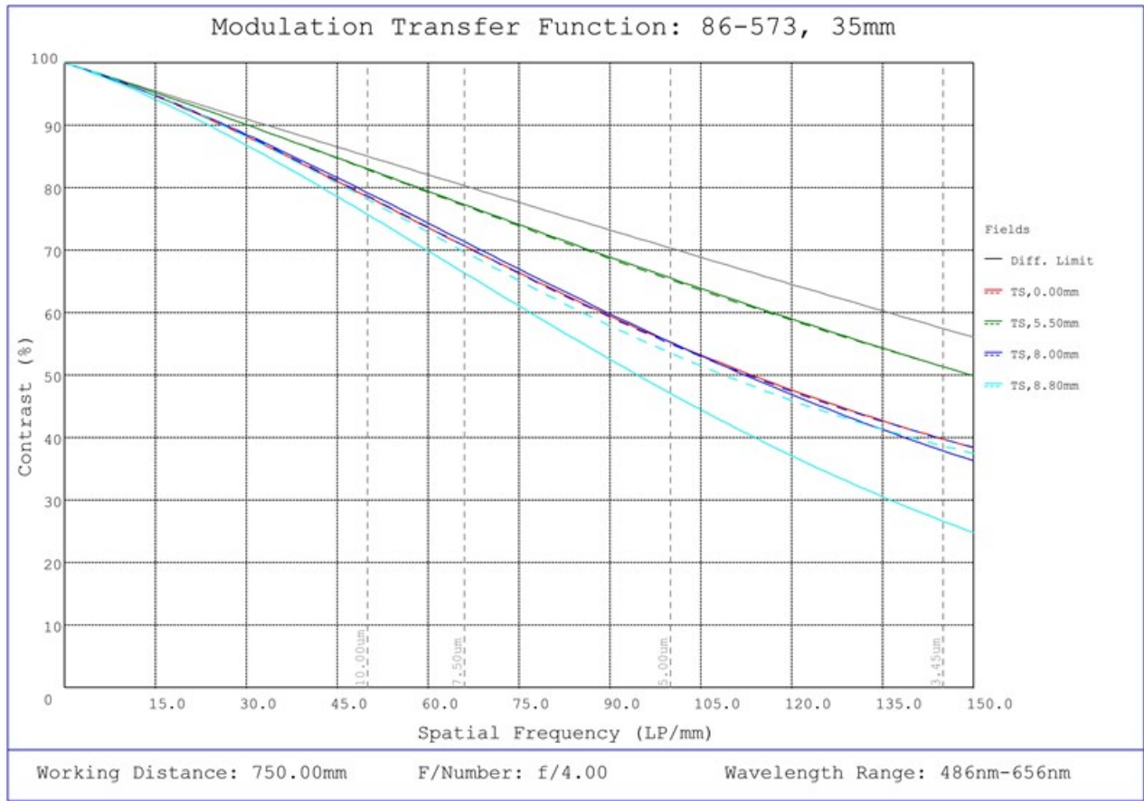
#86-573, 35mm Focal Length, HP Series Fixed Focal Length Lens, Modulated Transfer Function (MTF) Plot, 750mm Working Distance, f4
