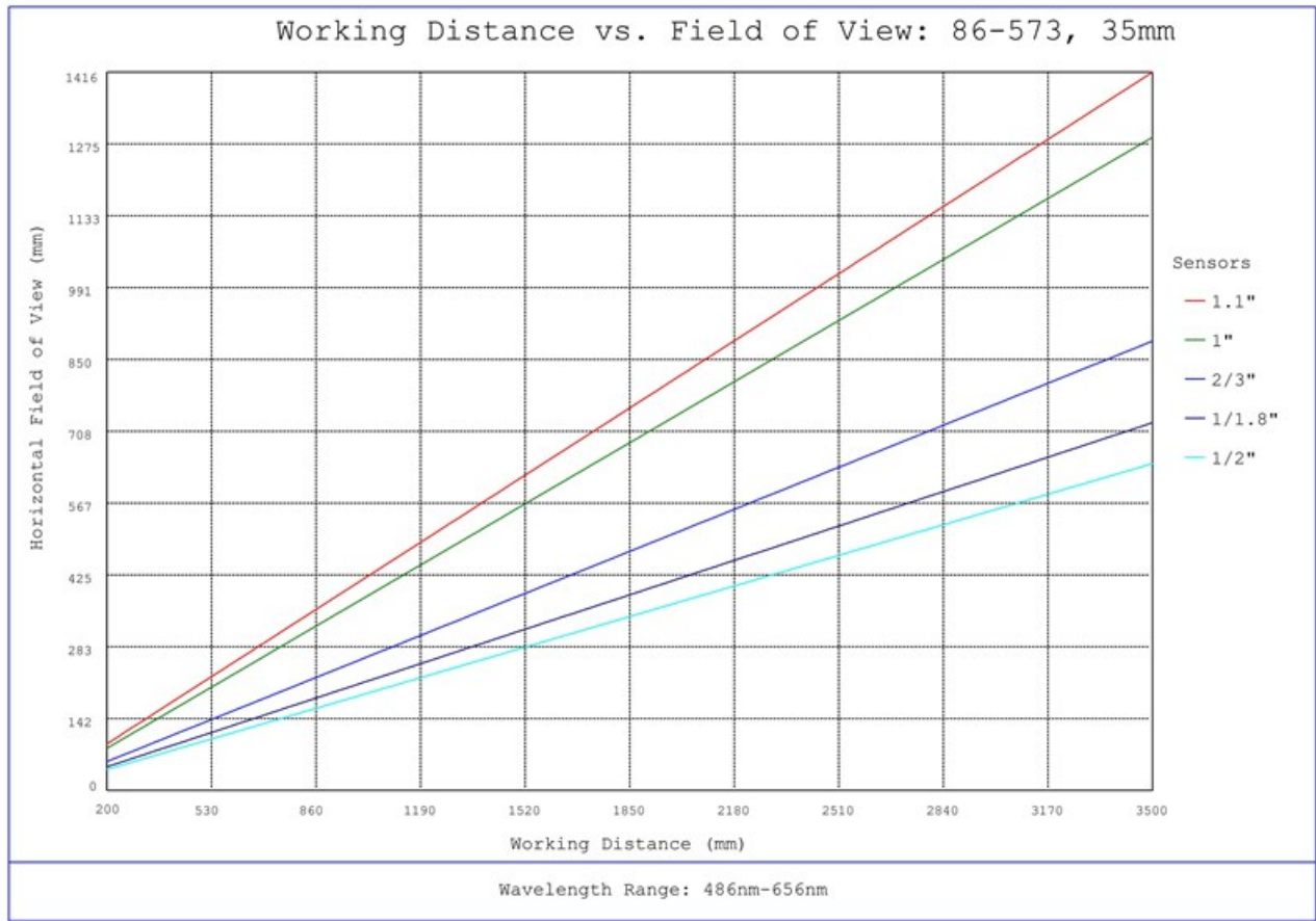
#86-573, 35mm Focal Length, HP Series Fixed Focal Length Lens, Working Distance versus Field of View Plot
