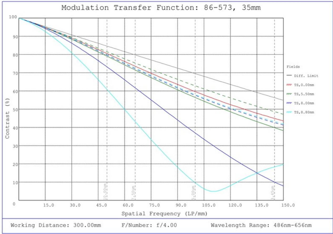
#86-573, 35mm Focal Length, HP Series Fixed Focal Length Lens, Modulated Transfer Function (MTF) Plot, 300mm Working Distance, f4
