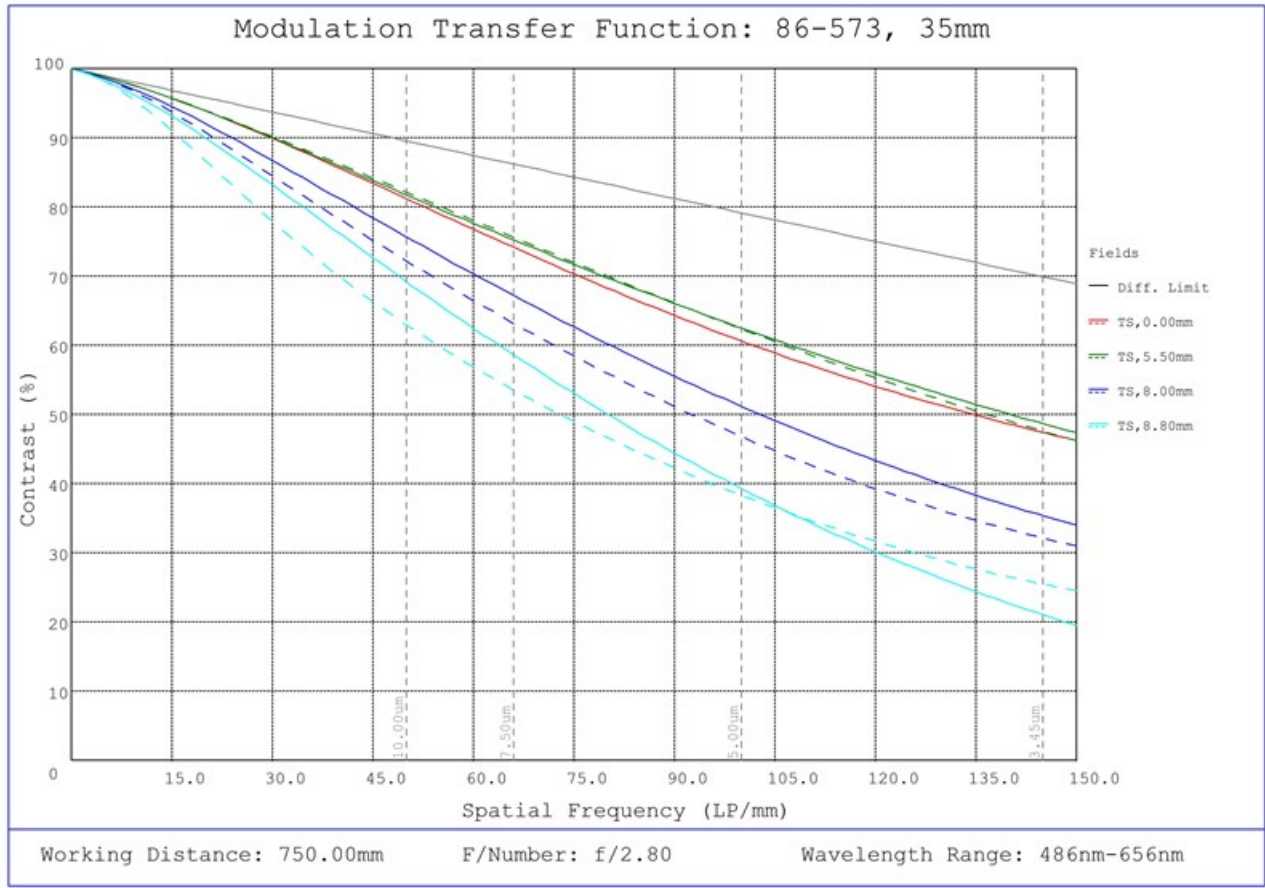
#86-573, 35mm Focal Length, HP Series Fixed Focal Length Lens, Modulated Transfer Function (MTF) Plot, 750mm Working Distance, f2.8
