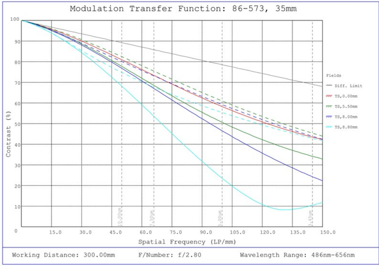
#86-573, 35mm Focal Length, HP Series Fixed Focal Length Lens, Modulated Transfer Function (MTF) Plot, 300mm Working Distance, f2.8
