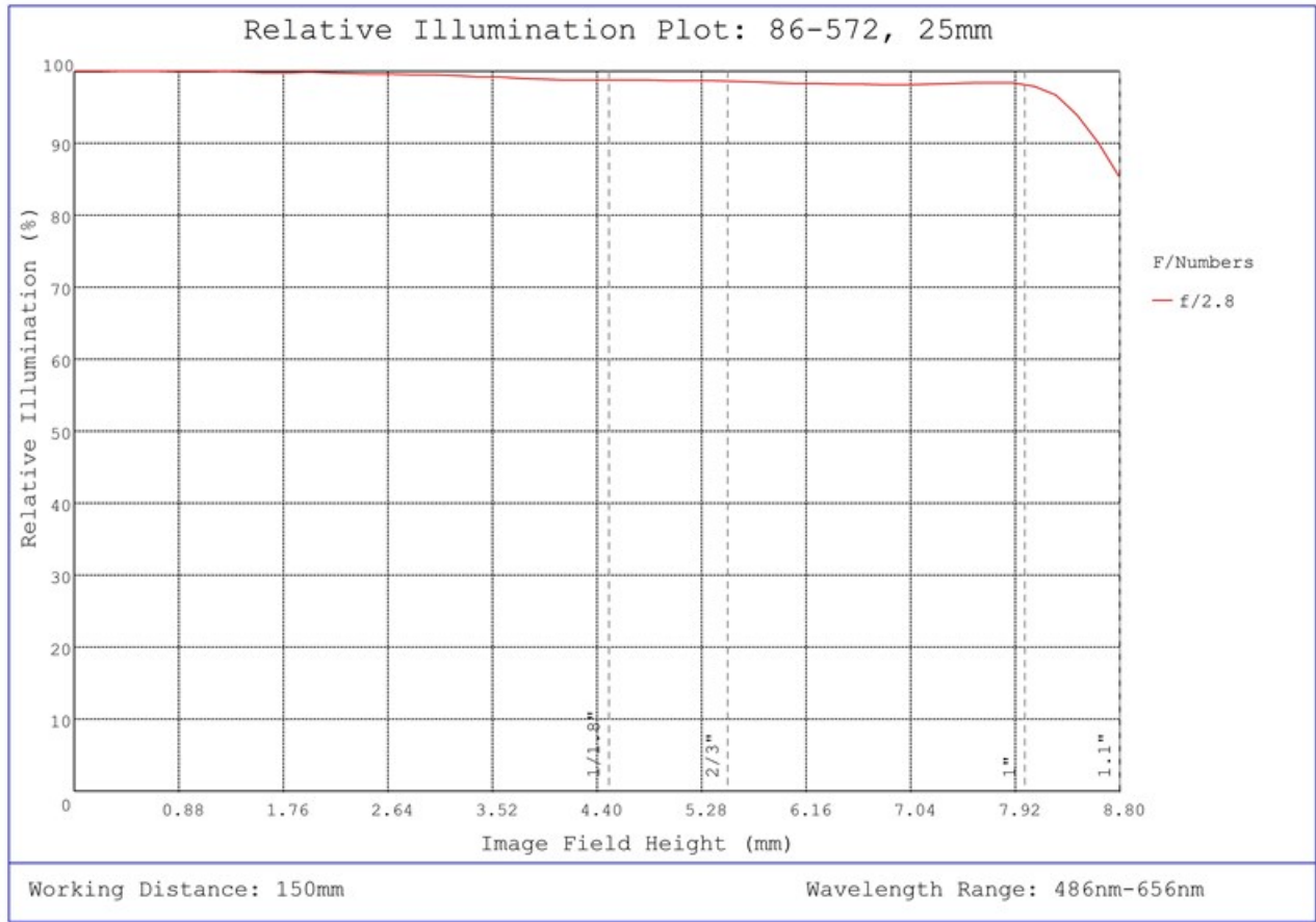
#86-572, 25mm Focal Length, HP Series Fixed Focal Length Lens, Relative Illumination Plot
