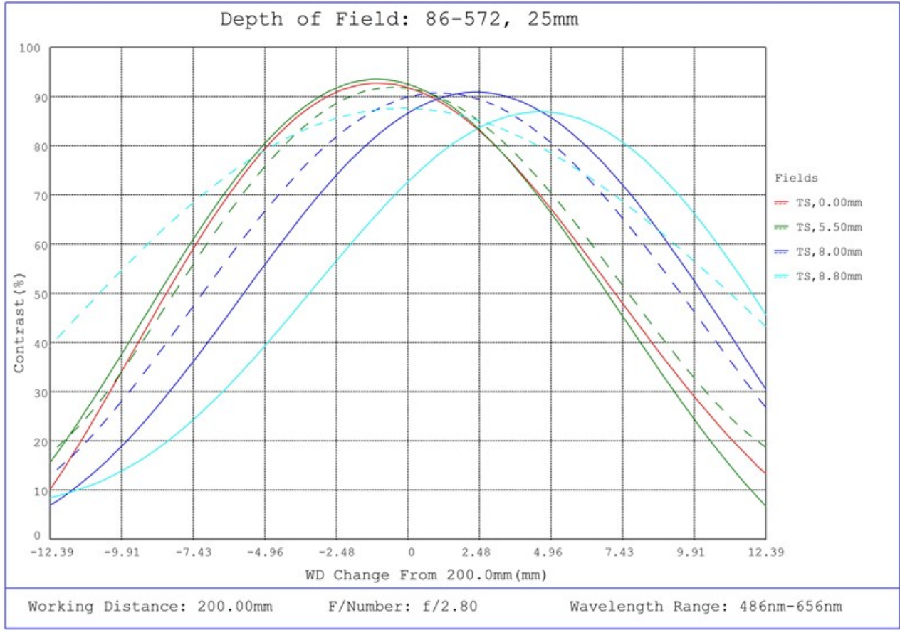
#86-572, 25mm Focal Length, HP Series Fixed Focal Length Lens, Depth of Field Plot, 200mm Working Distance, f2.8
