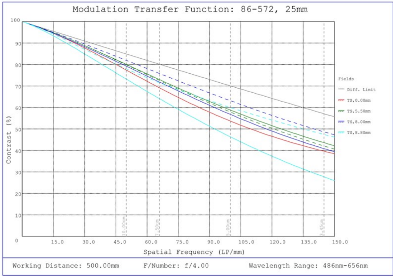
#86-572, 25mm Focal Length, HP Series Fixed Focal Length Lens, Modulated Transfer Function (MTF) Plot, 500mm Working Distance, f4
