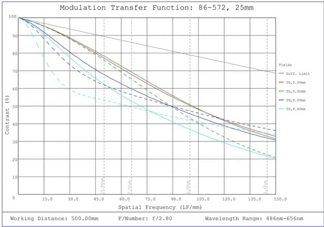
#86-572, 25mm Focal Length, HP Series Fixed Focal Length Lens, Modulated Transfer Function (MTF) Plot, 500mm Working Distance, f2.8
