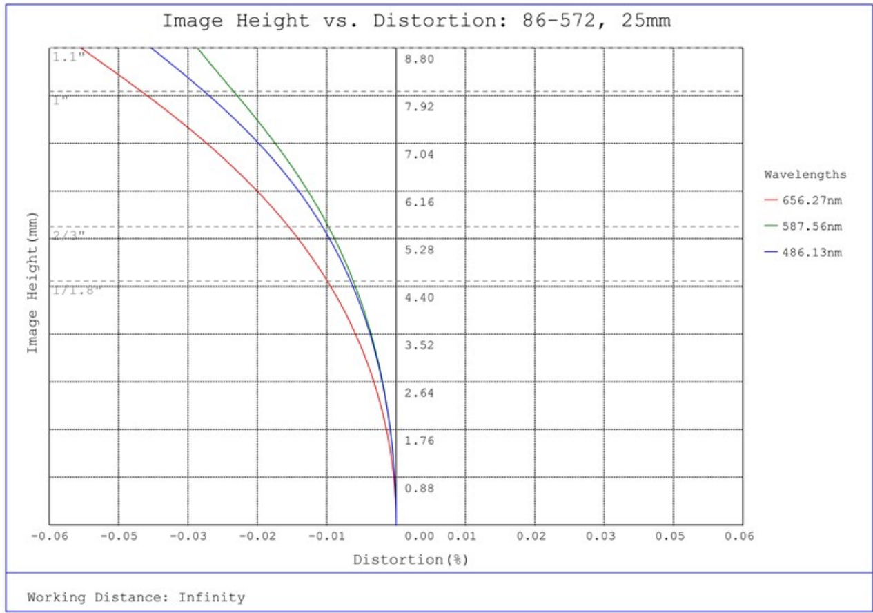
#86-572, 25mm Focal Length, HP Series Fixed Focal Length Lens, Distortion Plot
