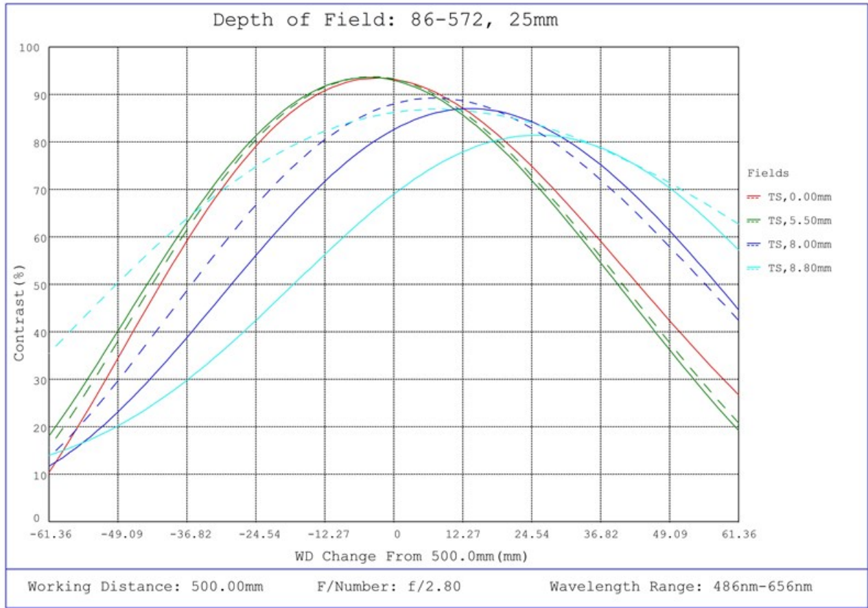
#86-572, 25mm Focal Length, HP Series Fixed Focal Length Lens, Depth of Field Plot, 500mm Working Distance, f2.8
