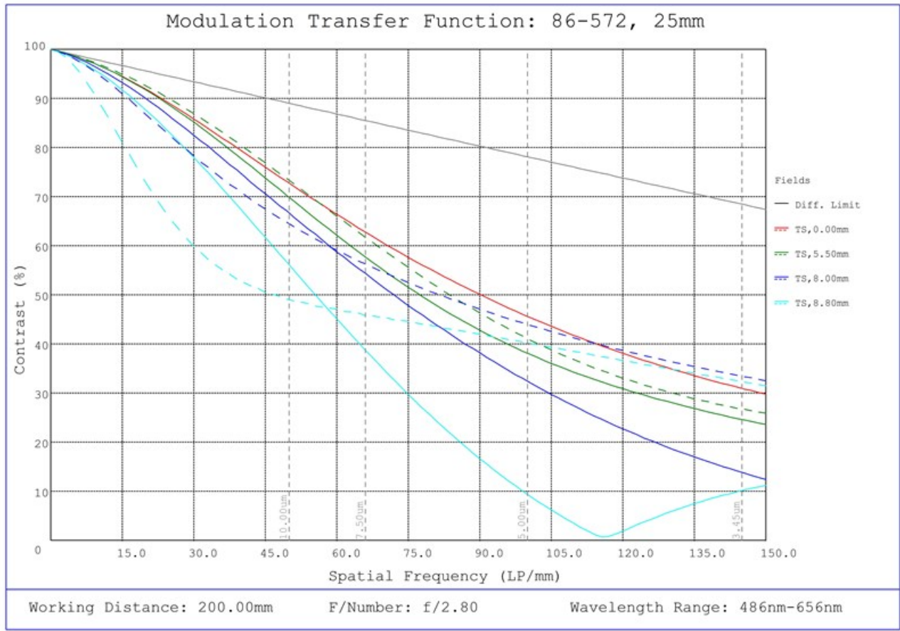
#86-572, 25mm Focal Length, HP Series Fixed Focal Length Lens, Modulated Transfer Function (MTF) Plot, 200mm Working Distance, f2.8
