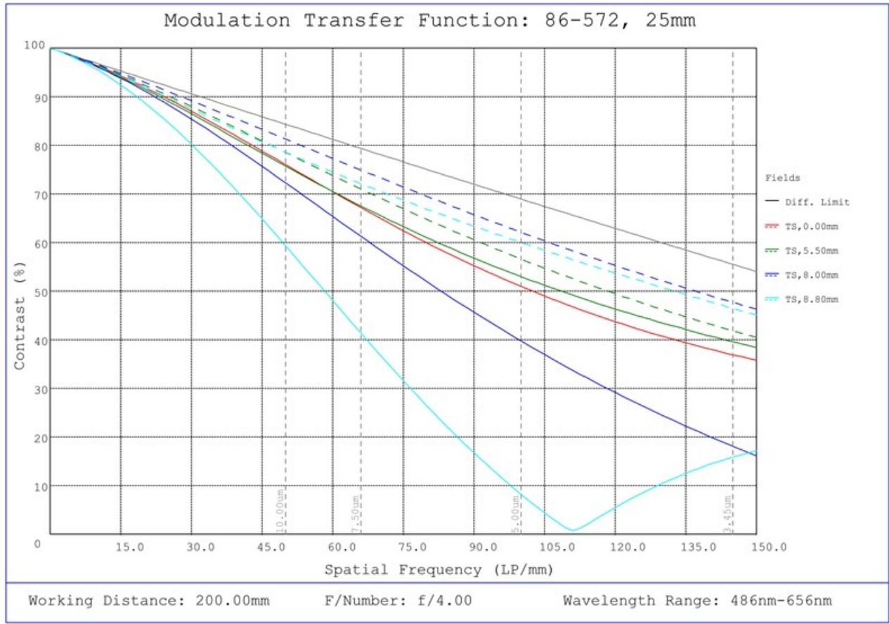
#86-572, 25mm Focal Length, HP Series Fixed Focal Length Lens, Modulated Transfer Function (MTF) Plot, 200mm Working Distance, f4
