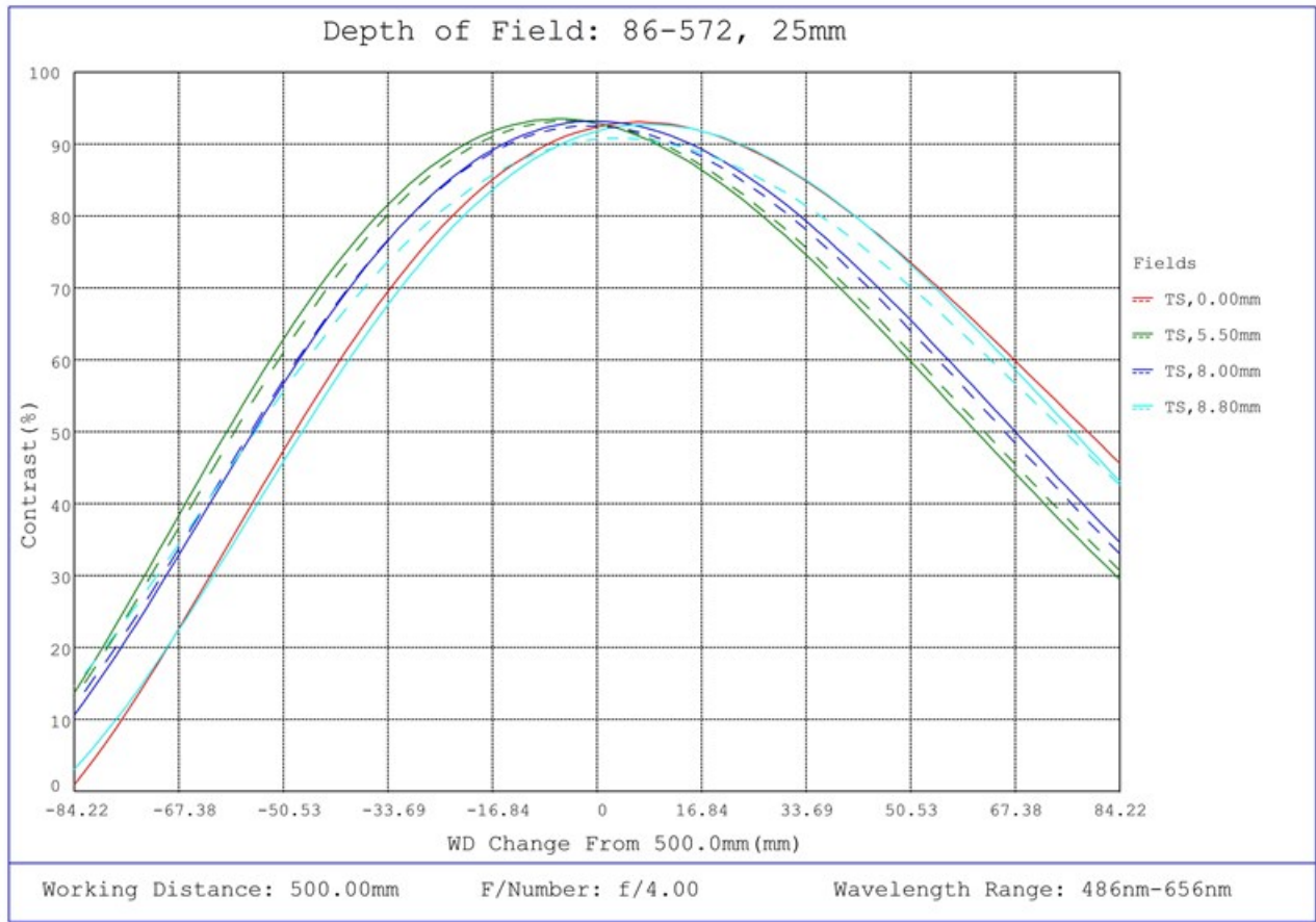
#86-572, 25mm Focal Length, HP Series Fixed Focal Length Lens, Depth of Field Plot, 500mm Working Distance, f4
