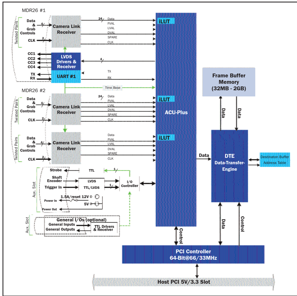
X64-CL Full - Functional Block Diagram
