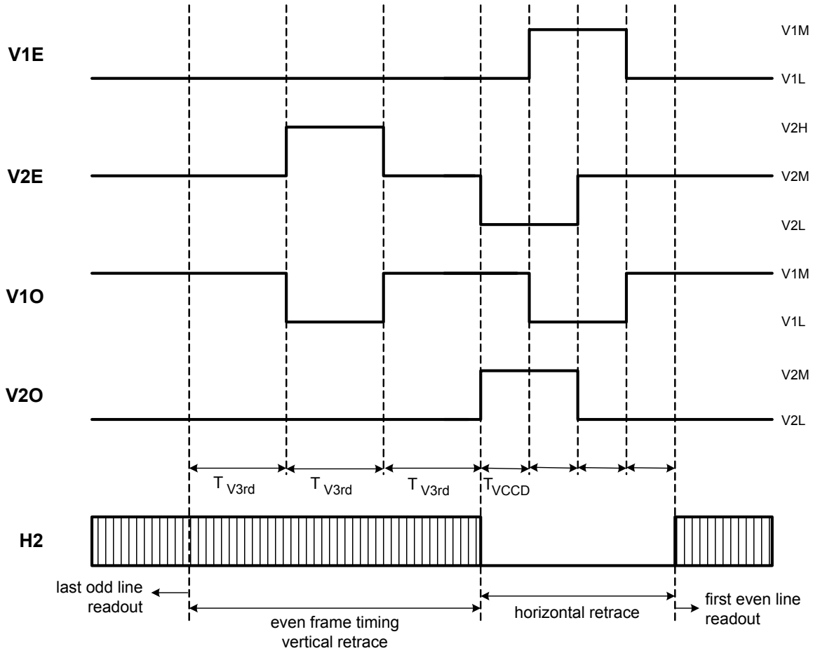
Figure 20: Non-Summed Interlaced Scan Even Frame Timing
