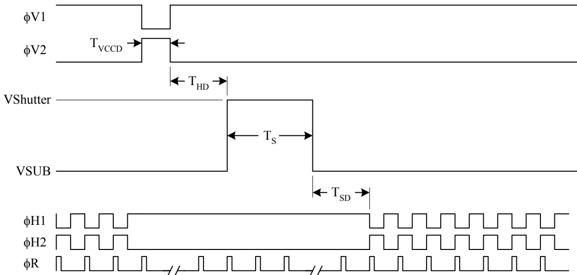
Figure 35: Electronic Shutter Line Timing
