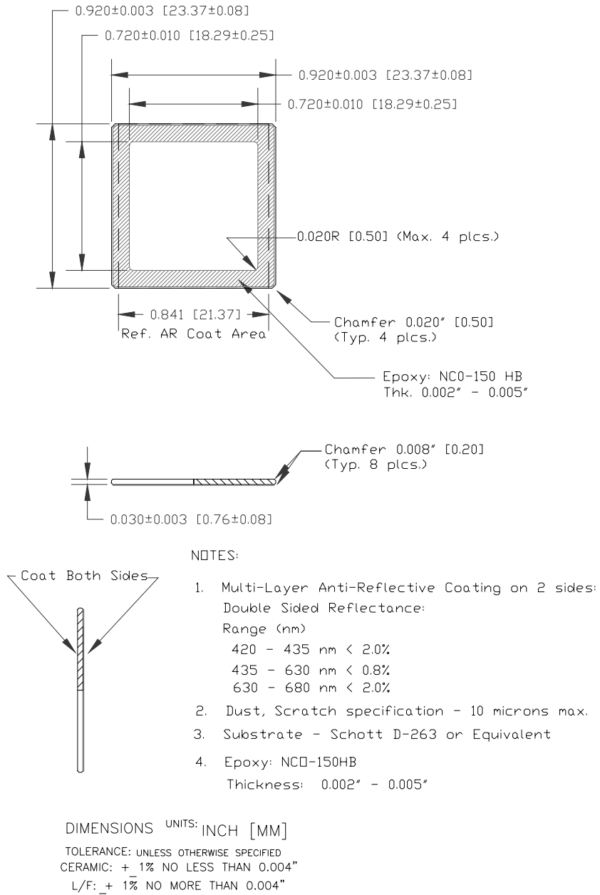
Figure 39: Glass Drawing
