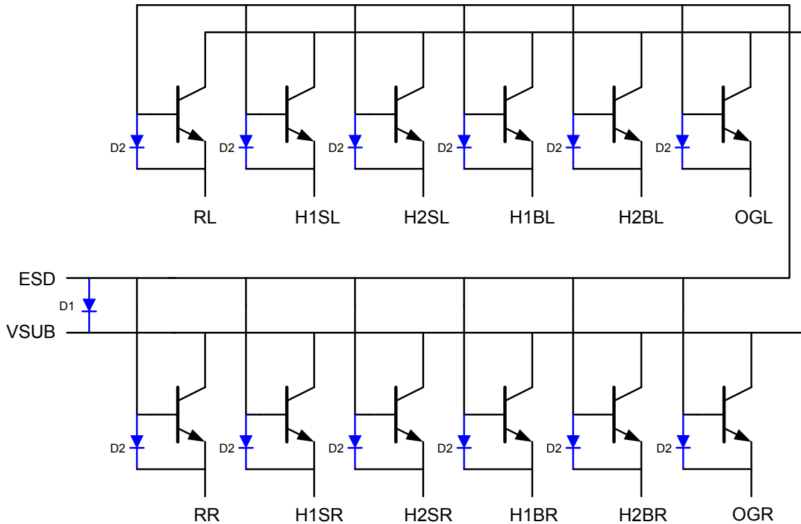
Figure 7: ESD Protection
