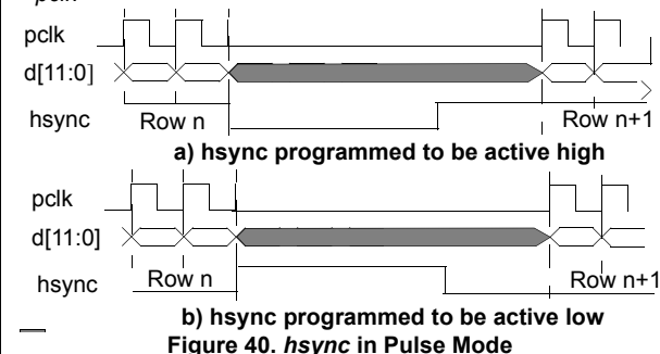
Figure 40. hsync in Pulse Mode
