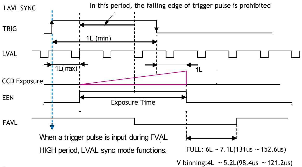
Fig. 26. Pulse width control. LVAL sync.
