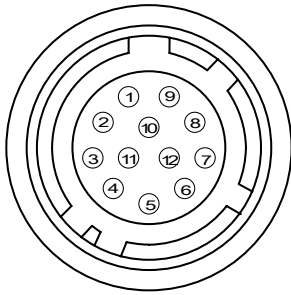
Fig. 2. 12-pin connector.
