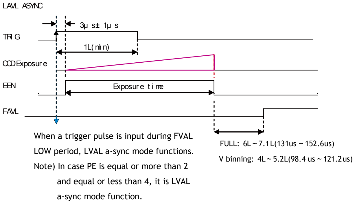
Fig.25. Edge Pre-select LVAL a-sync Timing
