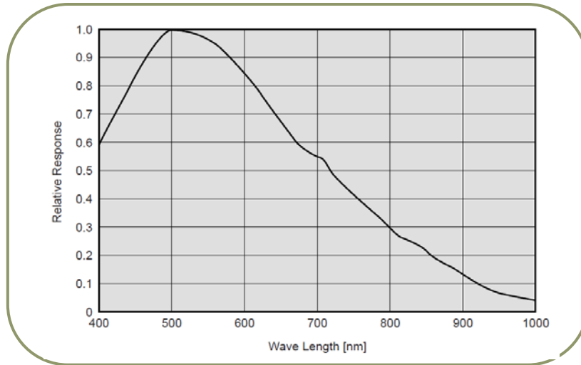
Fig. 29. Spectral response for CM-030GE
