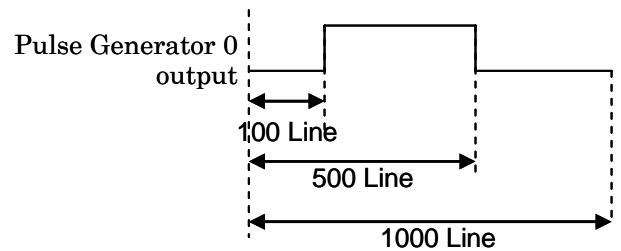
Fig.9. Pulse Generator 0 timing Example 2
