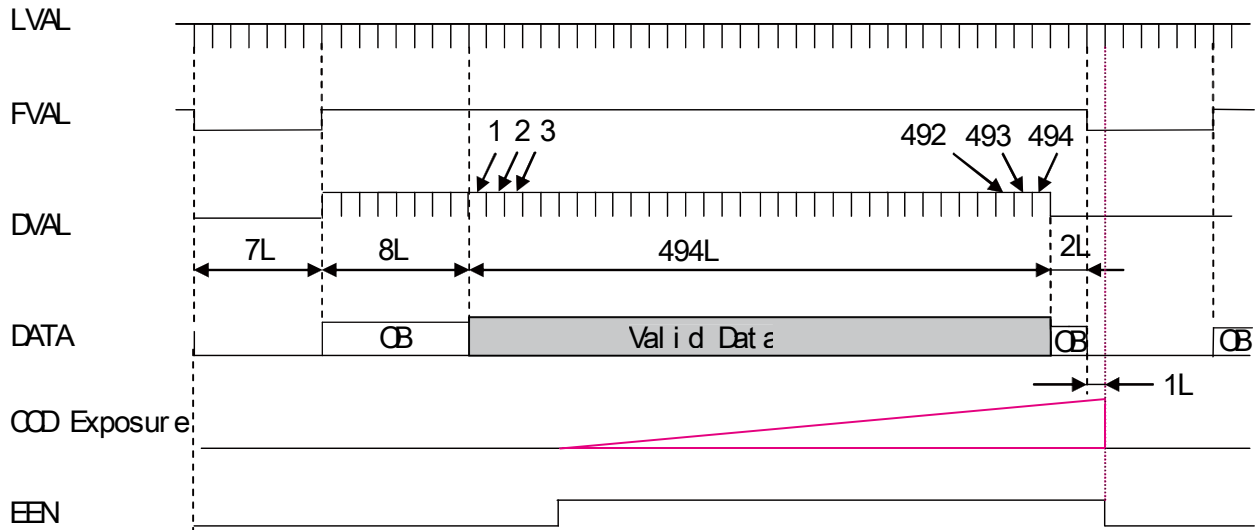
Fig. 19. Vertical timing for full scan
