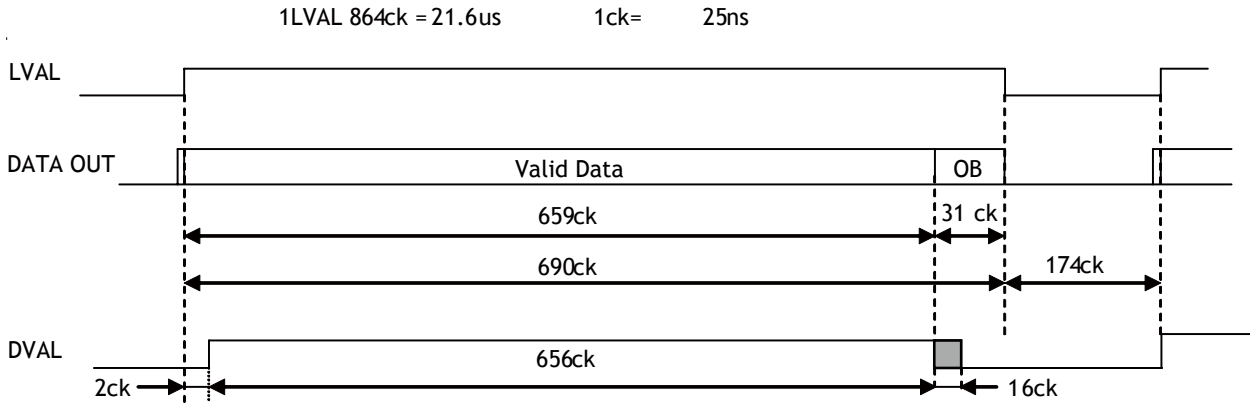
Fig.21. Horizontal Timing for Partial Scanning
