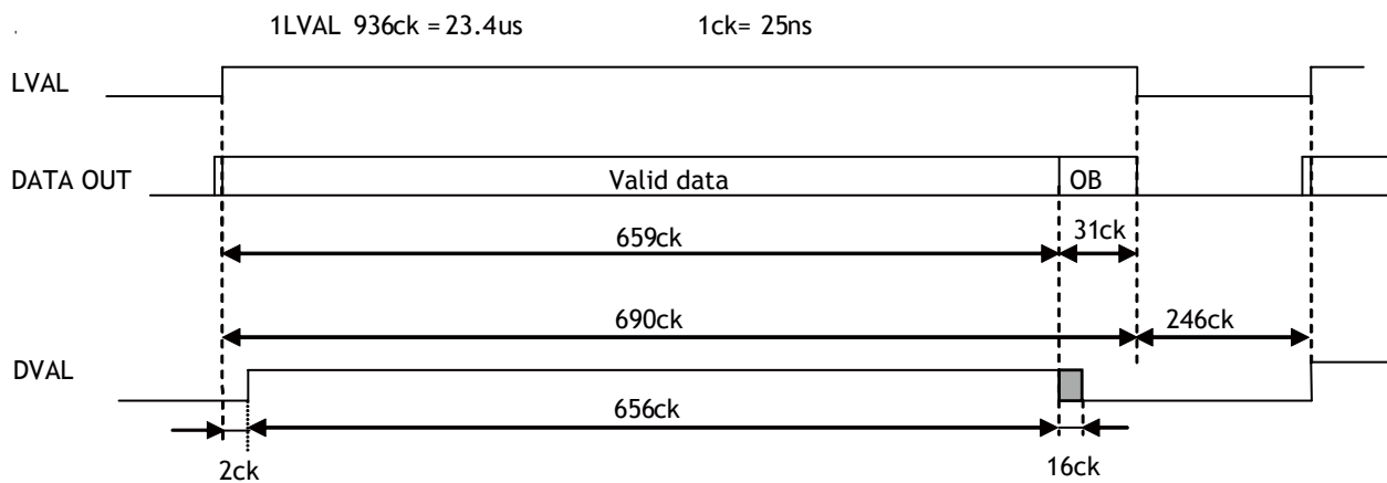
Fig.22. Horizontal Timing for Vertical Binning
