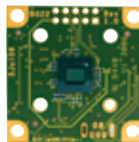
uEye® LE OEM 2 camera without lens adapter 36 x 36 x 8 mm (W x H x D) Weight: 8 g
