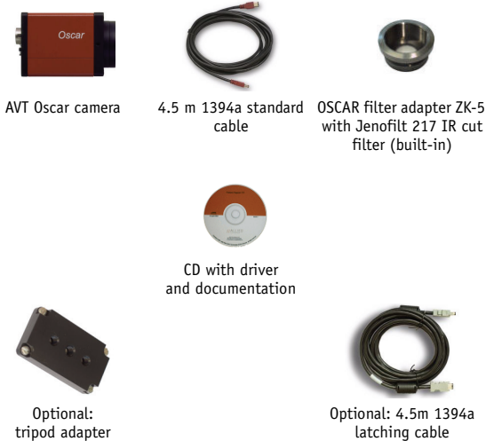
Figure 1: System components
