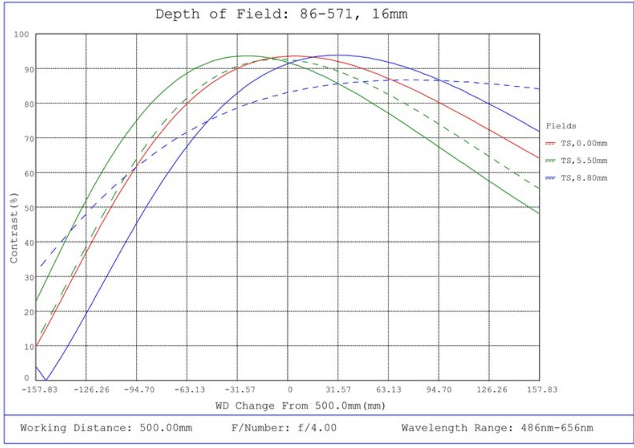
#86-571, 16mm Focal Length, HP Series Fixed Focal Length Lens, Depth of Field Plot, 500mm Working Distance, f4
