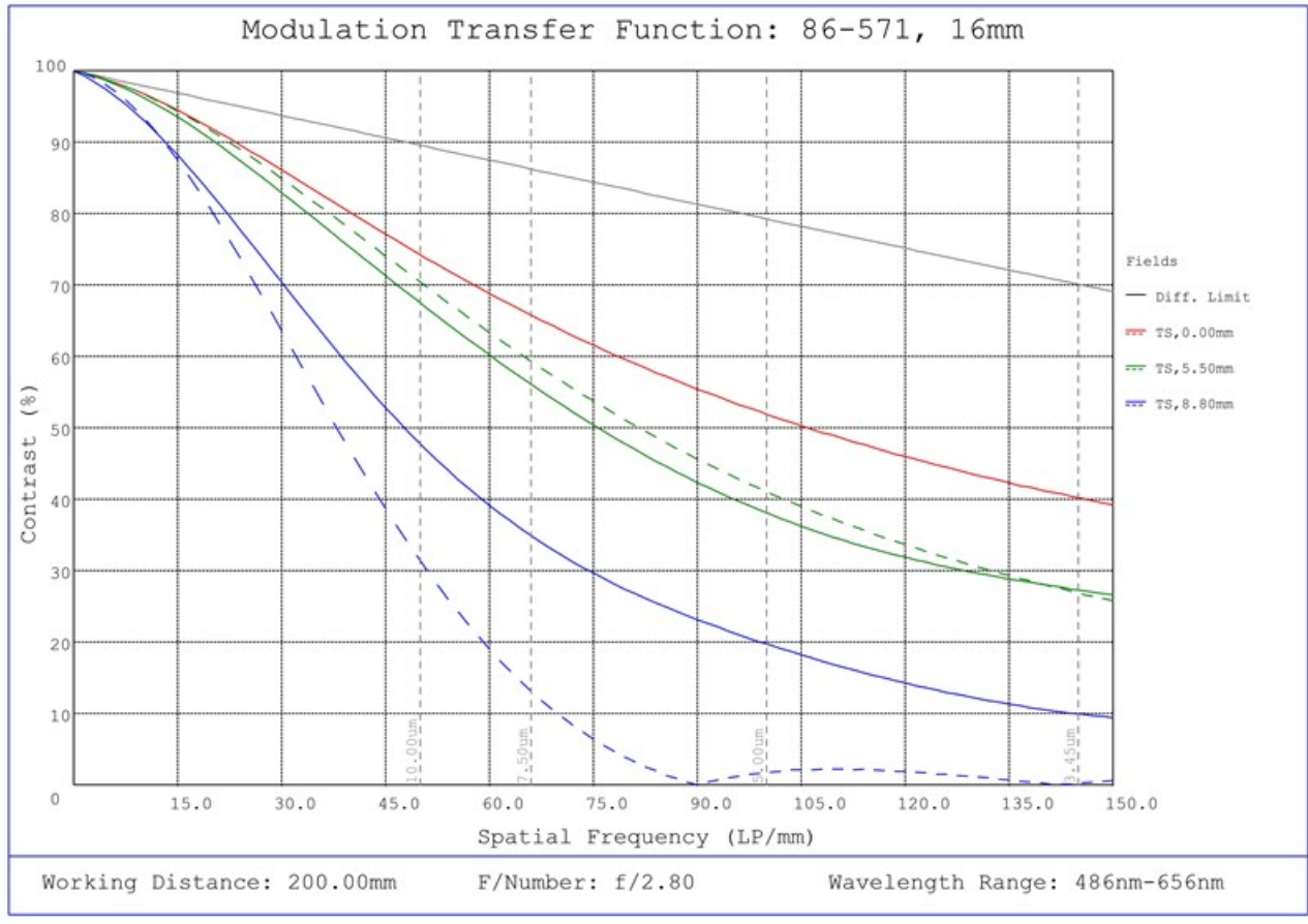
#86-571, 16mm Focal Length, HP Series Fixed Focal Length Lens, Modulated Transfer Function (MTF) Plot, 200mm Working Distance, f2.8
