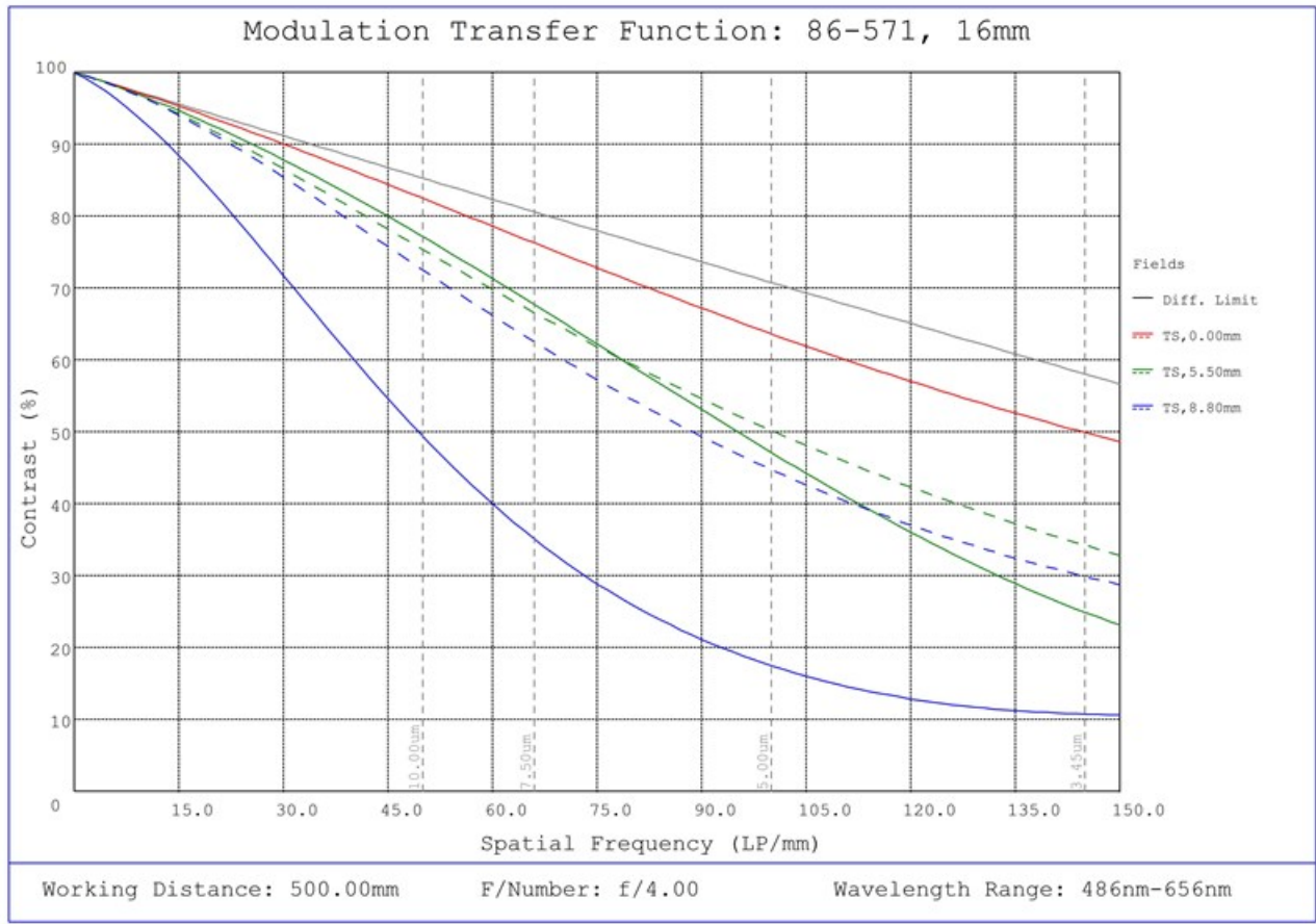
#86-571, 16mm Focal Length, HP Series Fixed Focal Length Lens, Modulated Transfer Function (MTF) Plot, 500mm Working Distance, f4
