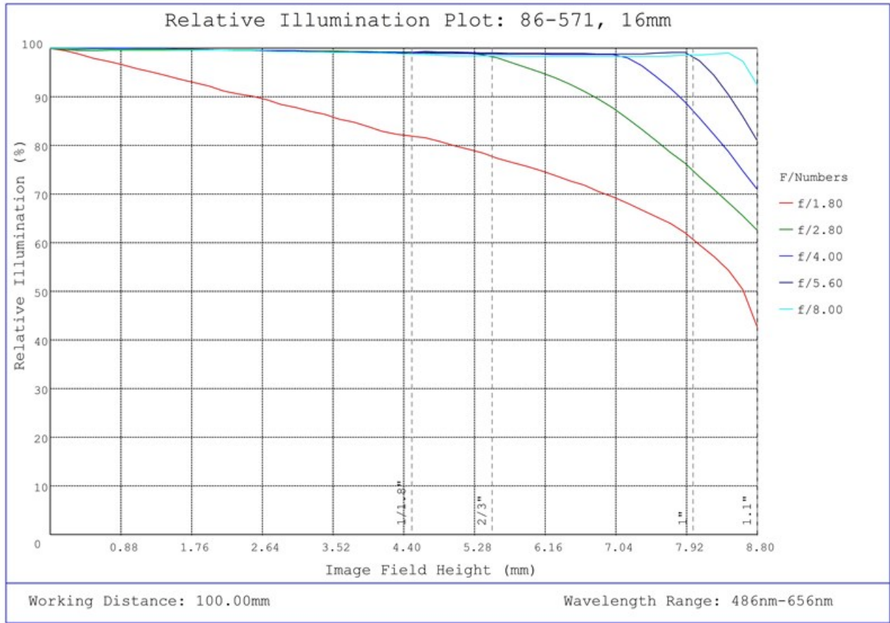
#86-571, 16mm Focal Length, HP Series Fixed Focal Length Lens, Relative Illumination Plot
