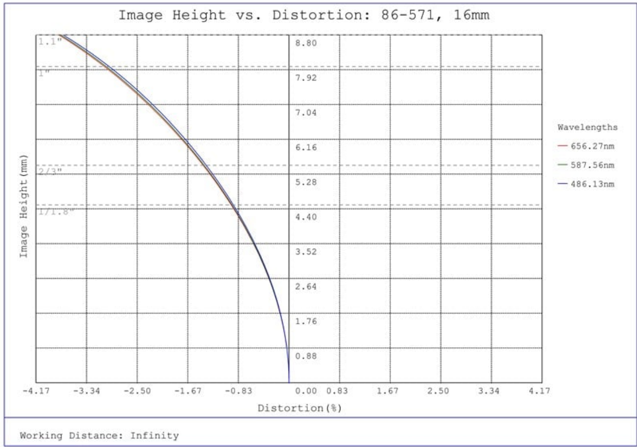
#86-571, 16mm Focal Length, HP Series Fixed Focal Length Lens, Distortion Plot
