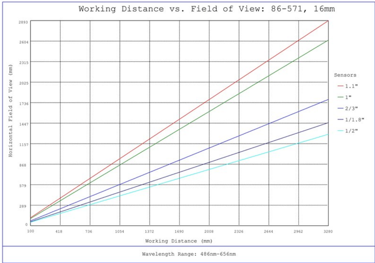
#86-571, 16mm Focal Length, HP Series Fixed Focal Length Lens, Working Distance versus Field of View Plot
