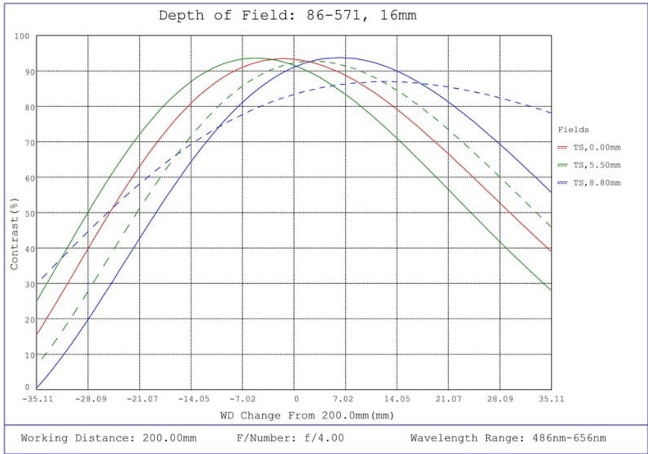
#86-571, 16mm Focal Length, HP Series Fixed Focal Length Lens, Depth of Field Plot, 200mm Working Distance, f4
