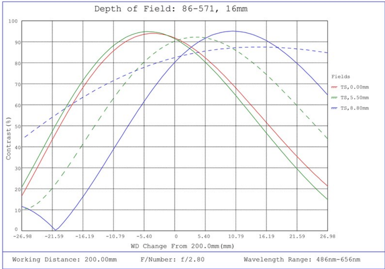
#86-571, 16mm Focal Length, HP Series Fixed Focal Length Lens, Depth of Field Plot, 200mm Working Distance, f2.8
