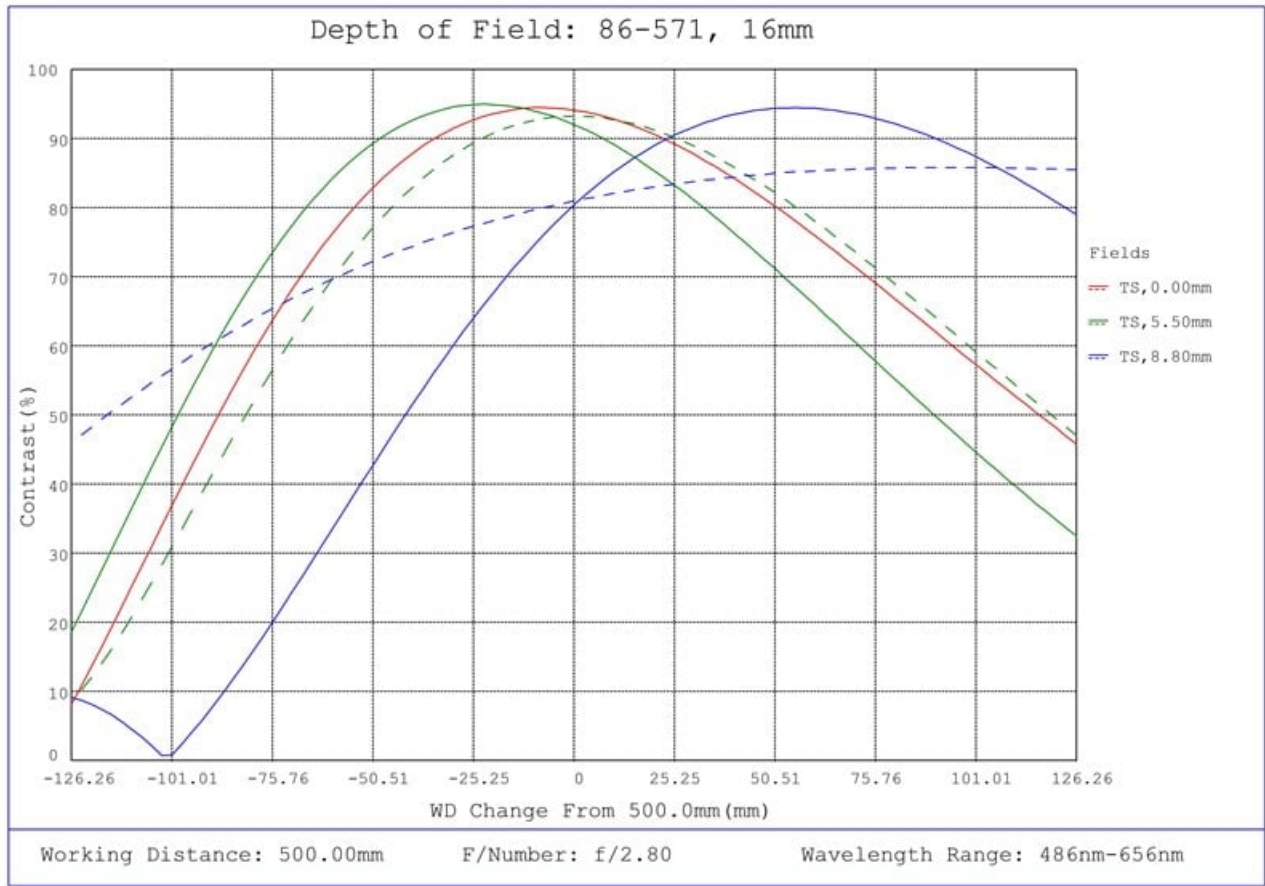
#86-571, 16mm Focal Length, HP Series Fixed Focal Length Lens, Depth of Field Plot, 500mm Working Distance, f2.8
