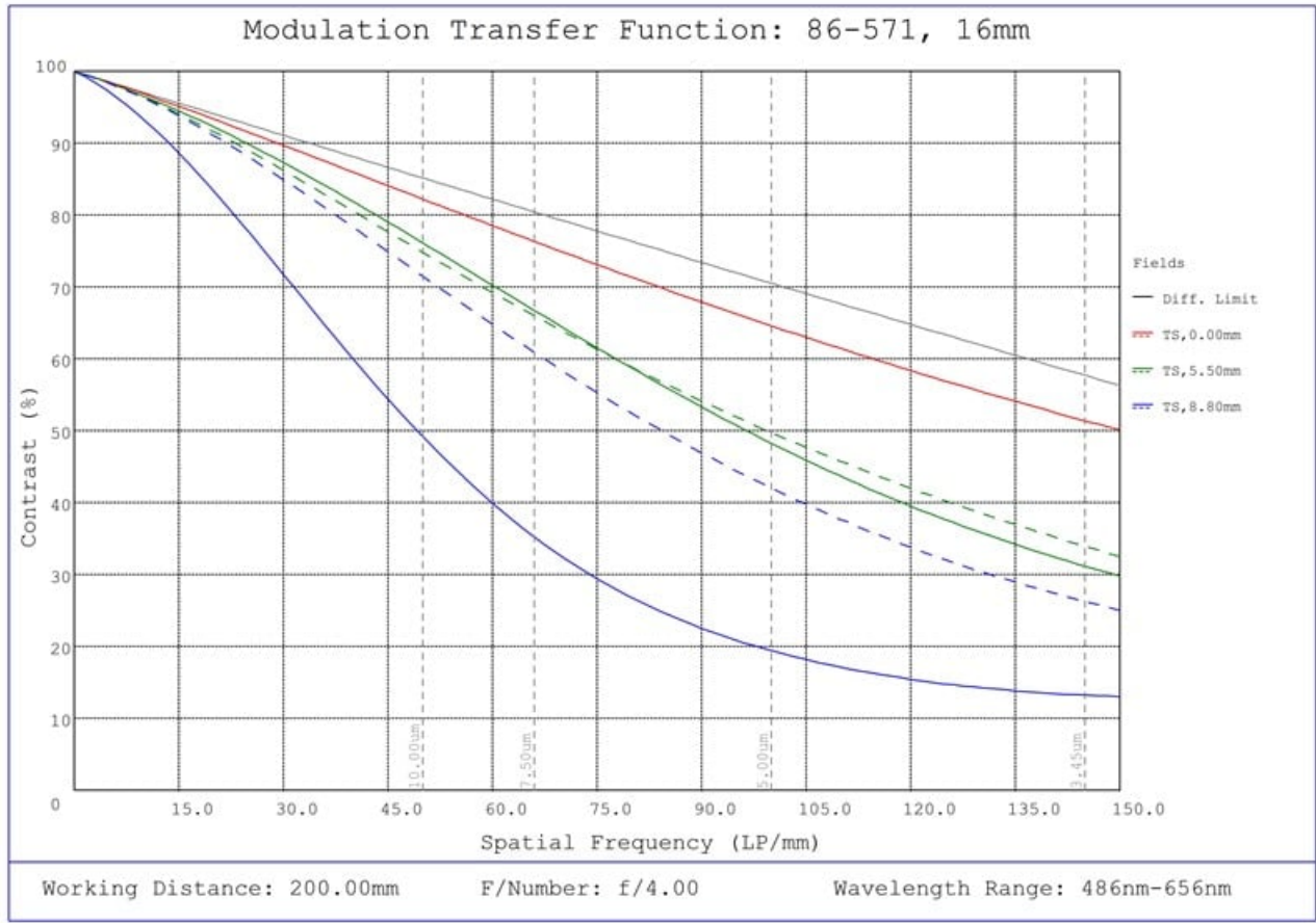
#86-571, 16mm Focal Length, HP Series Fixed Focal Length Lens, Modulated Transfer Function (MTF) Plot, 200mm Working Distance, f4
