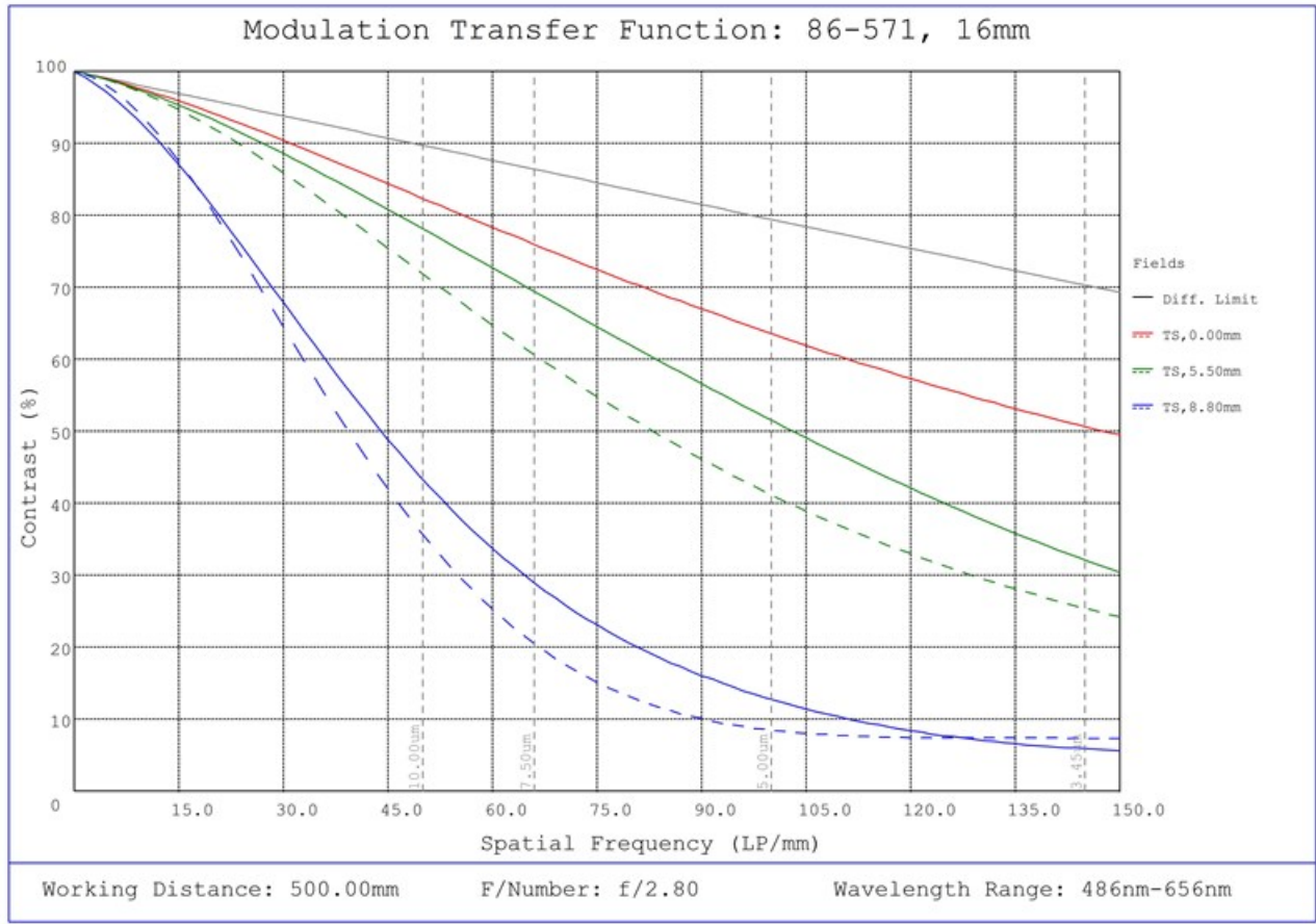
#86-571, 16mm Focal Length, HP Series Fixed Focal Length Lens, Modulated Transfer Function (MTF) Plot, 500mm Working Distance, f2.8
