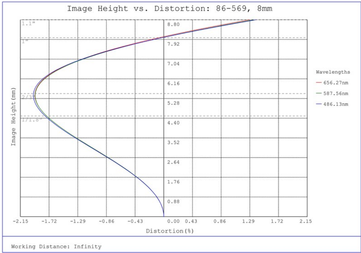
#86-569, 8mm Focal Length, HP Series Fixed Focal Length Lens, Distortion Plot
