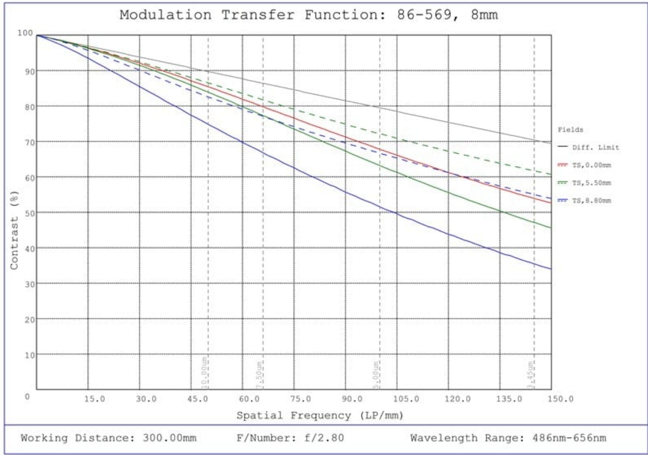
#86-569, 8mm Focal Length, HP Series Fixed Focal Length Lens, Modulated Transfer Function (MTF) Plot, 300mm Working Distance, f2.8
