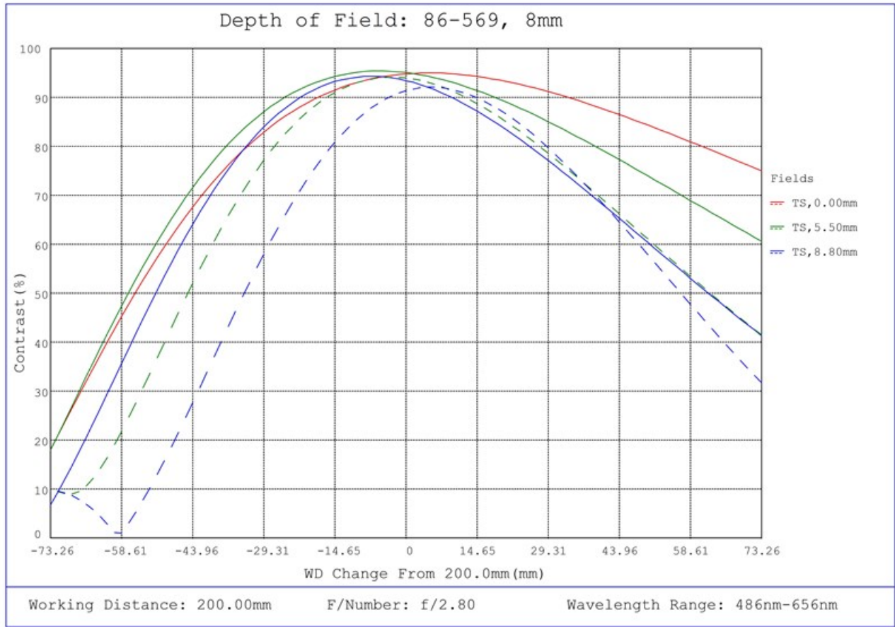
#86-569, 8mm Focal Length, HP Series Fixed Focal Length Lens, Depth of Field Plot, 200mm Working Distance, f2.8
