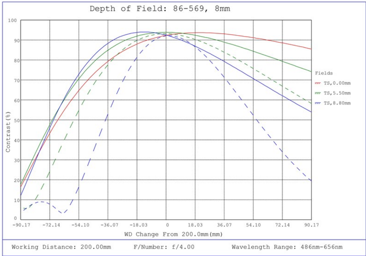
#86-569, 8mm Focal Length, HP Series Fixed Focal Length Lens, Depth of Field Plot, 200mm Working Distance, f4
