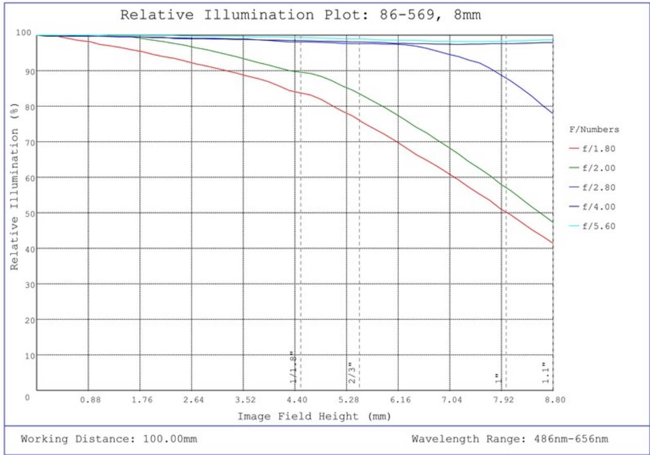
#86-569, 8mm Focal Length, HP Series Fixed Focal Length Lens, Relative Illumination Plot
