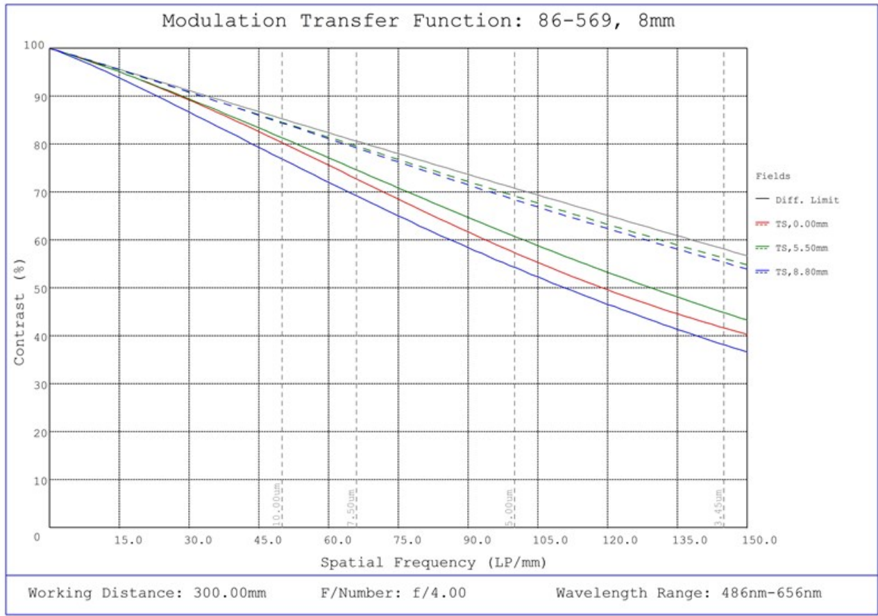
#86-569, 8mm Focal Length, HP Series Fixed Focal Length Lens, Modulated Transfer Function (MTF) Plot, 300mm Working Distance, f4
