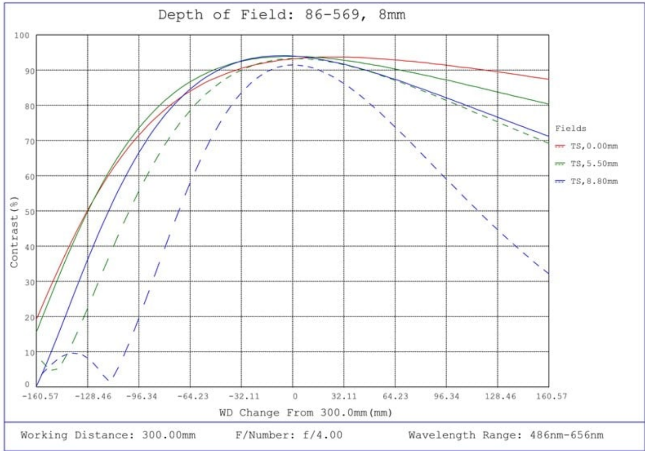
#86-569, 8mm Focal Length, HP Series Fixed Focal Length Lens, Depth of Field Plot, 300mm Working Distance, f4
