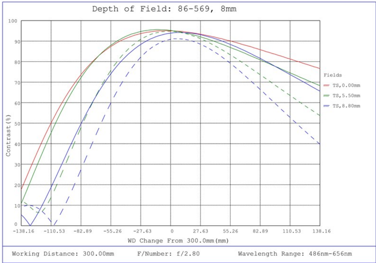
#86-569, 8mm Focal Length, HP Series Fixed Focal Length Lens, Depth of Field Plot, 300mm Working Distance, f2.8
