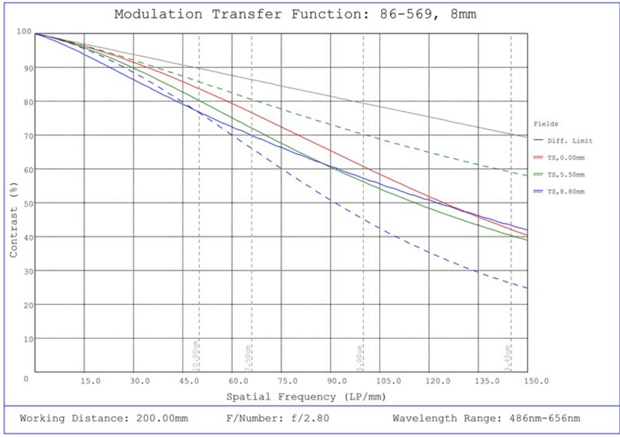
#86-569, 8mm Focal Length, HP Series Fixed Focal Length Lens, Modulated Transfer Function (MTF) Plot, 200mm Working Distance, f2.8
