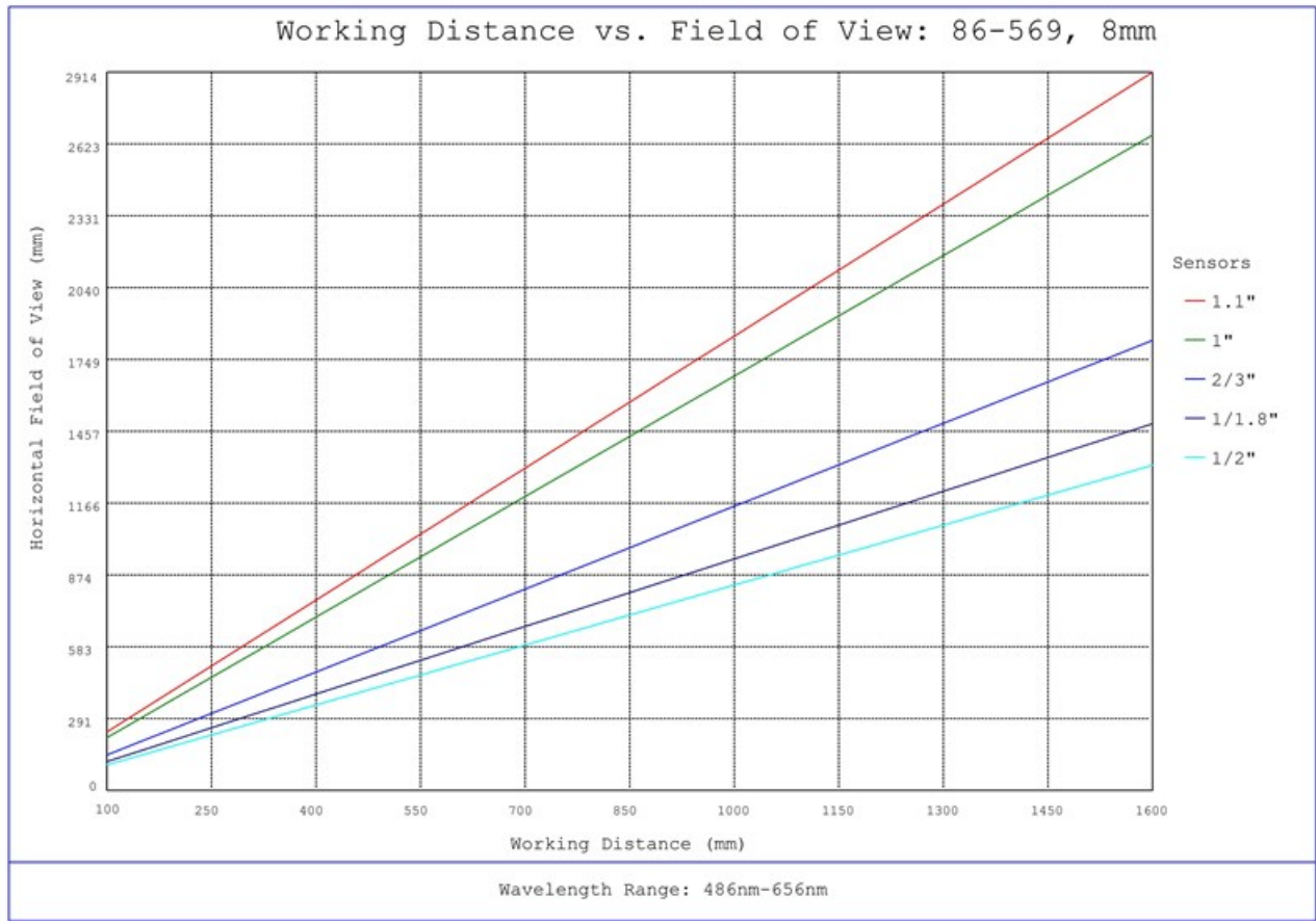
#86-569, 8mm Focal Length, HP Series Fixed Focal Length Lens, Working Distance versus Field of View Plot
