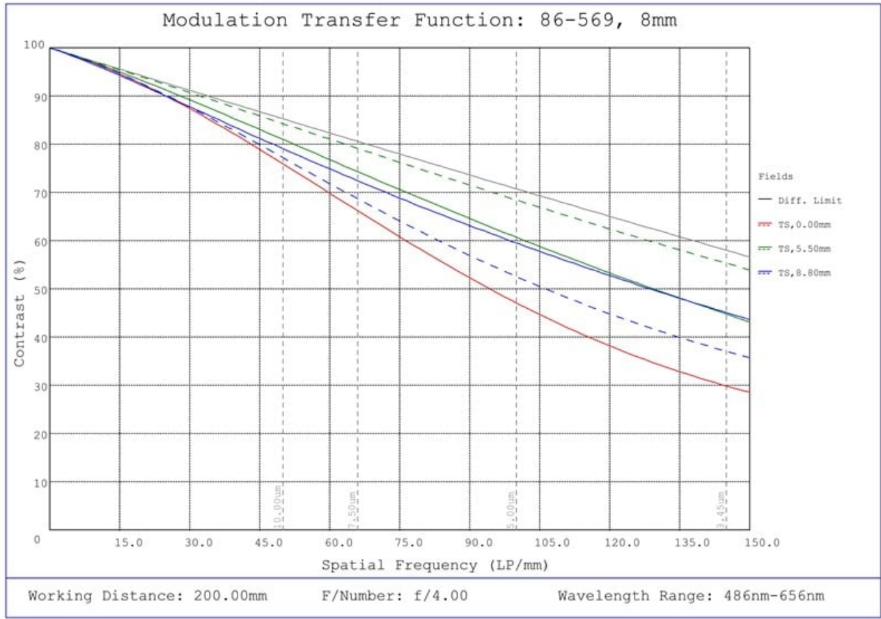
#86-569, 8mm Focal Length, HP Series Fixed Focal Length Lens, Modulated Transfer Function (MTF) Plot, 200mm Working Distance, f4
