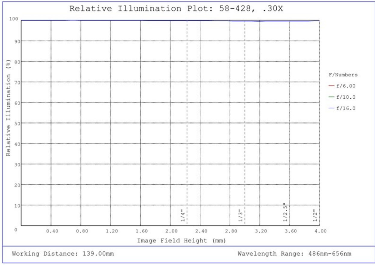
#58-428, 0.30X SilverTL™ Telecentric Lens, Relative Illumination Plot
