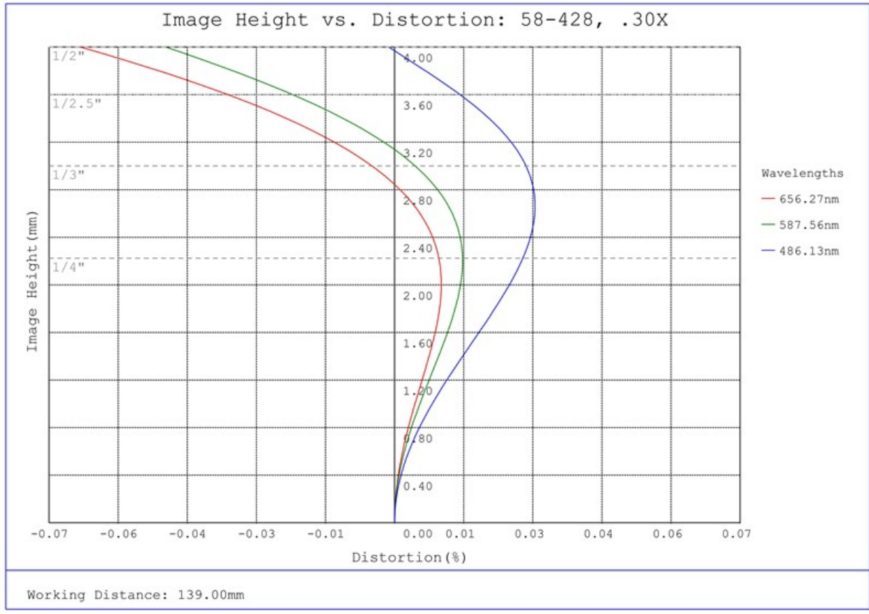
#58-428, 0.30X SilverTL™ Telecentric Lens, Distortion Plot
