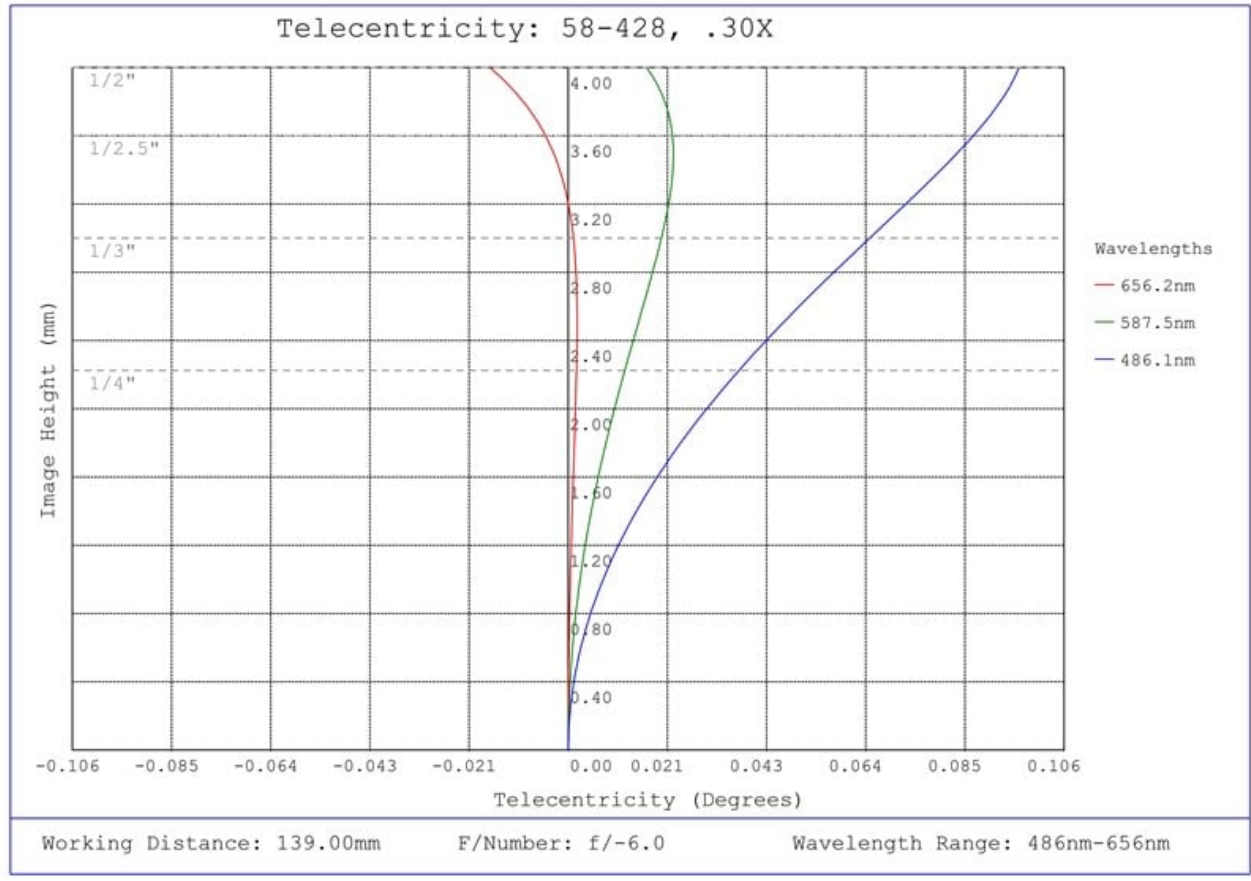
#58-428, 0.30X SilverTL™ Telecentric Lens, Telecentricity Plot
