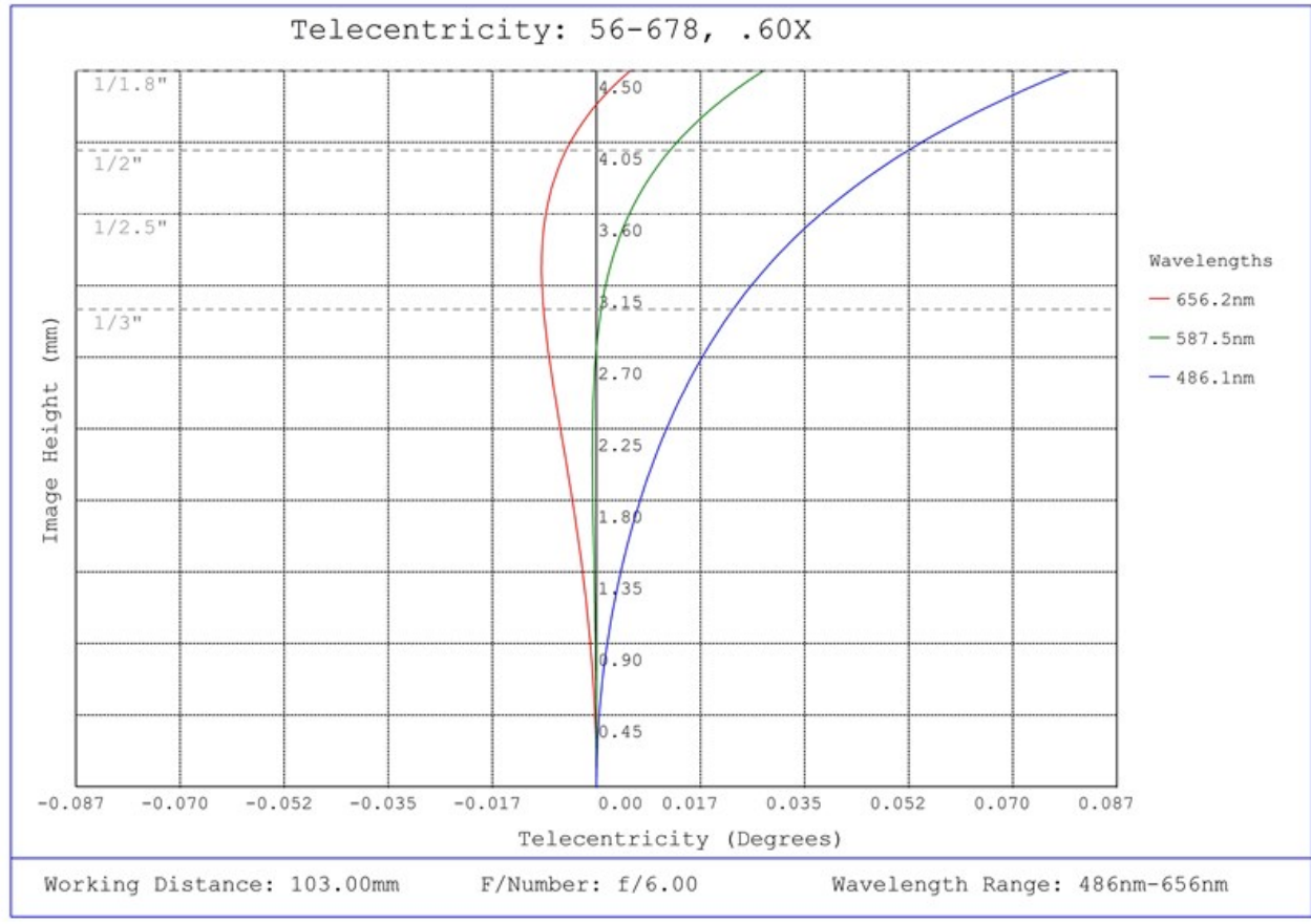
#56-678, 0.60X SilverTL™ Telecentric Lens, Telecentricity Plot
