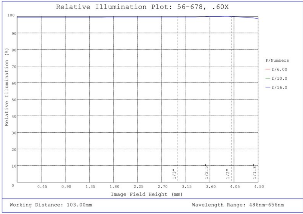
#56-678, 0.60X SilverTL™ Telecentric Lens, Relative Illumination Plot
