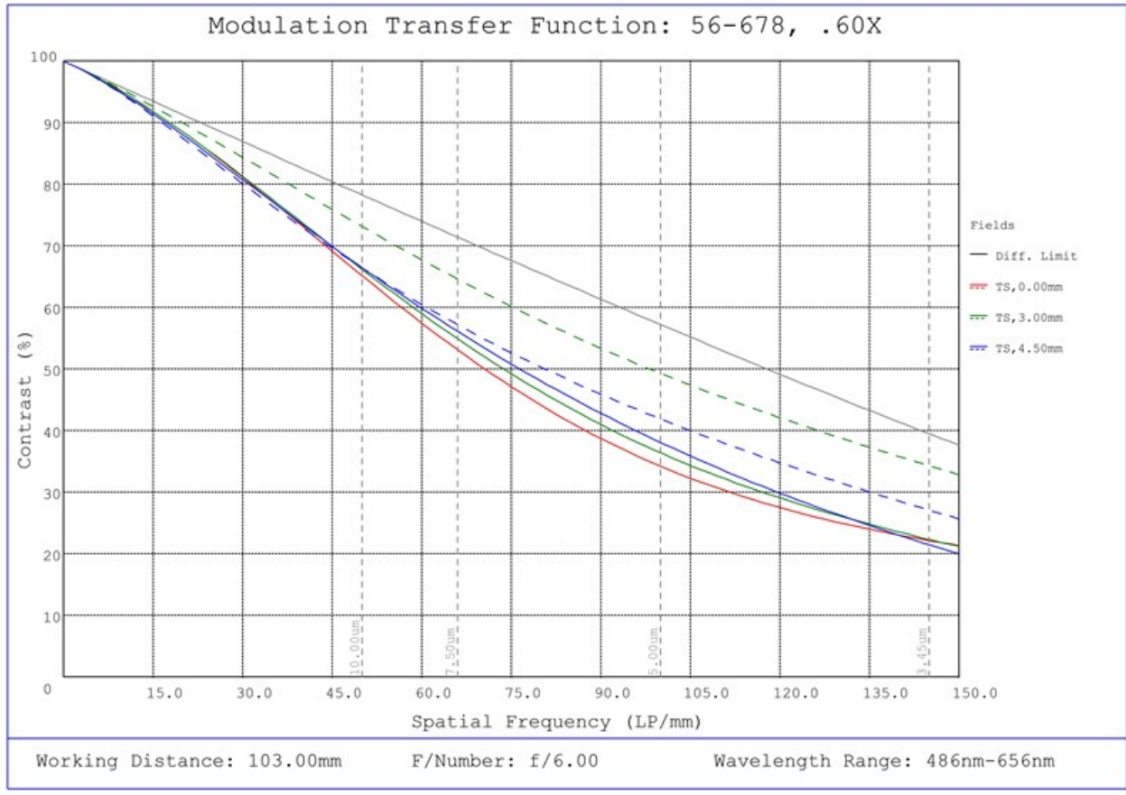
#56-678, 0.60X SilverTL™ Telecentric Lens, Modulated Transfer Function (MTF) Plot, 103mm Working Distance, f6
