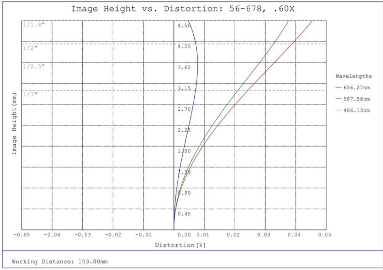
#56-678, 0.60X SilverTL™ Telecentric Lens, Distortion Plot
