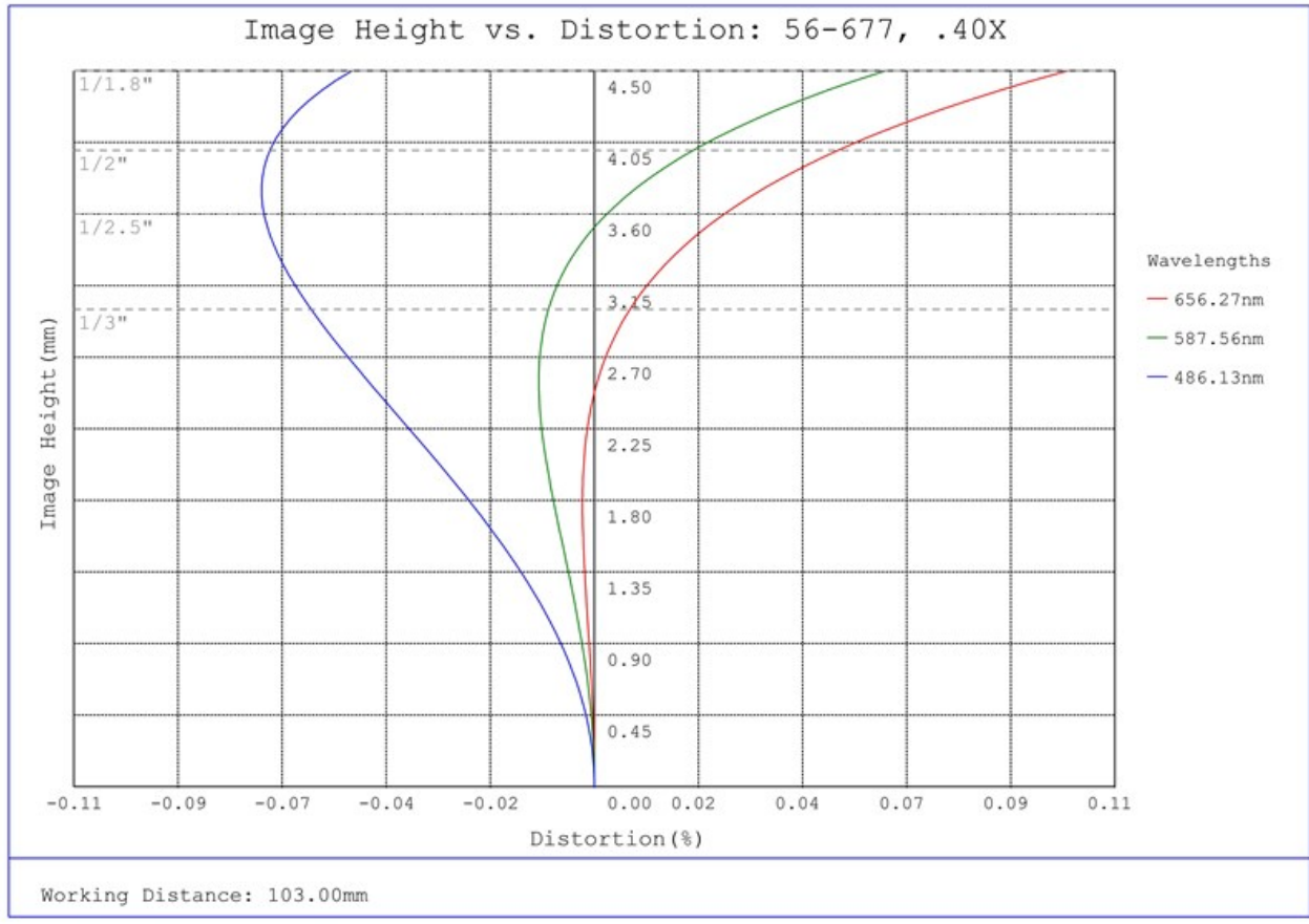
#56-677, 0.40X SilverTL™ Telecentric Lens, Distortion Plot
