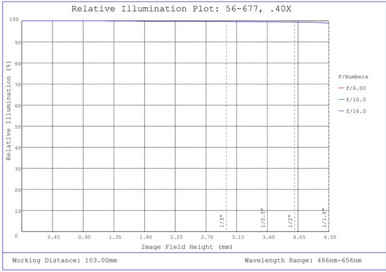
#56-677, 0.40X SilverTL™ Telecentric Lens, Relative Illumination Plot
