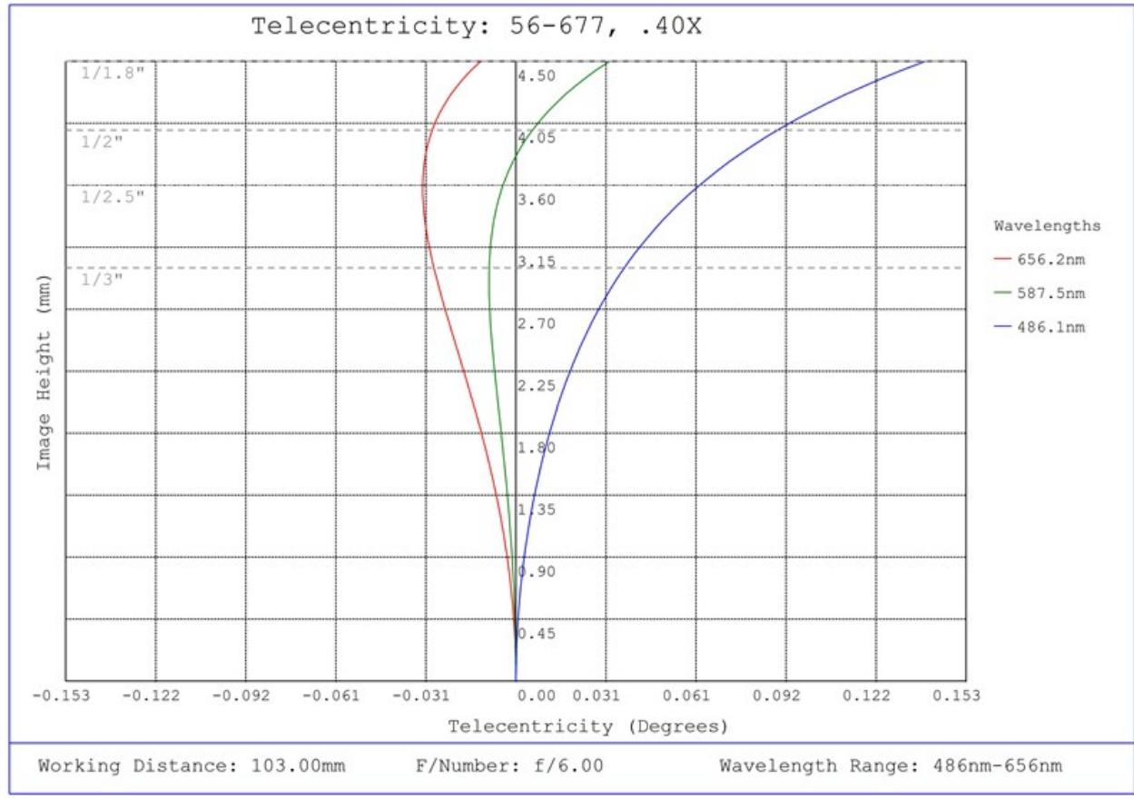
#56-677, 0.40X SilverTL™ Telecentric Lens, Telecentricity Plot
