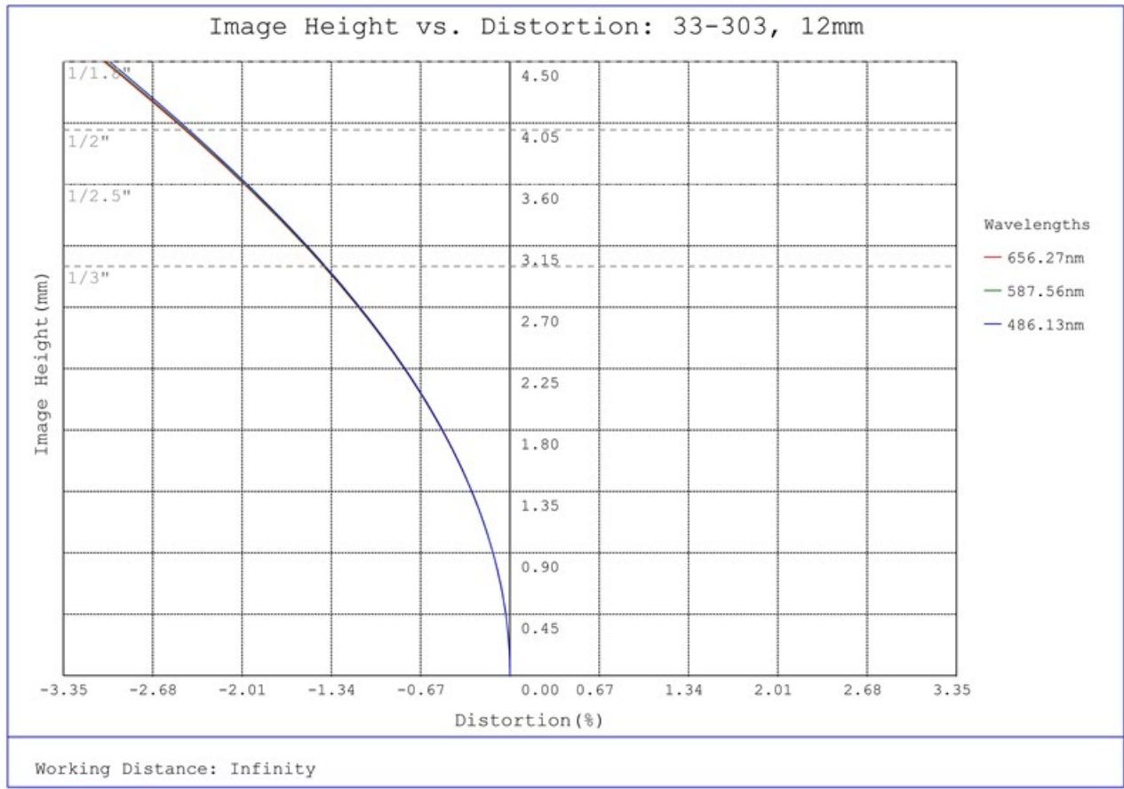
#33-303, 12mm UC Series Fixed Focal Length Lens, Distortion Plot
