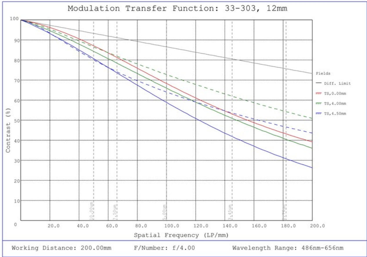
#33-303, 12mm UC Series Fixed Focal Length Lens, Modulated Transfer Function (MTF) Plot, 200mm Working Distance, f4
