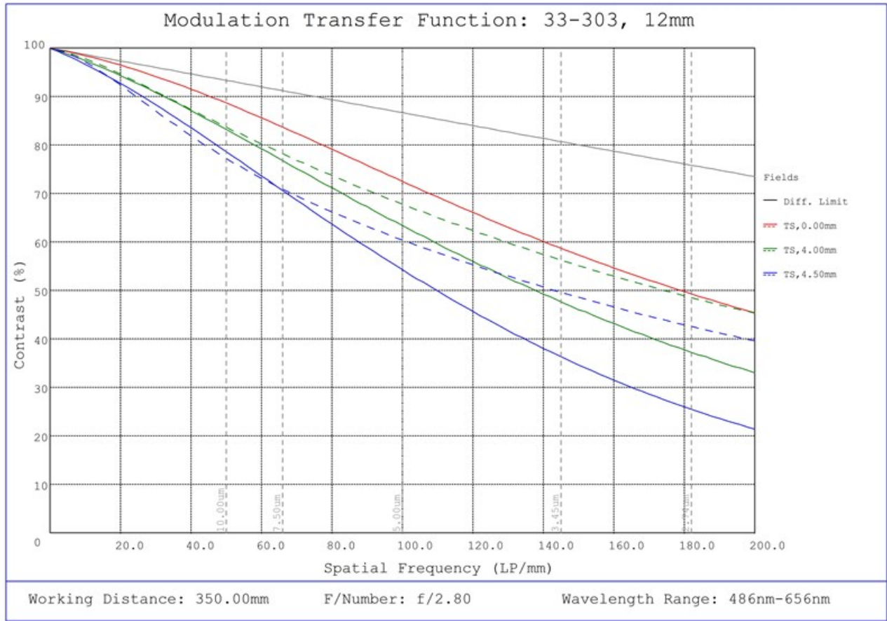
#33-303, 12mm UC Series Fixed Focal Length Lens, Modulated Transfer Function (MTF) Plot, 350mm Working Distance, f2.8
