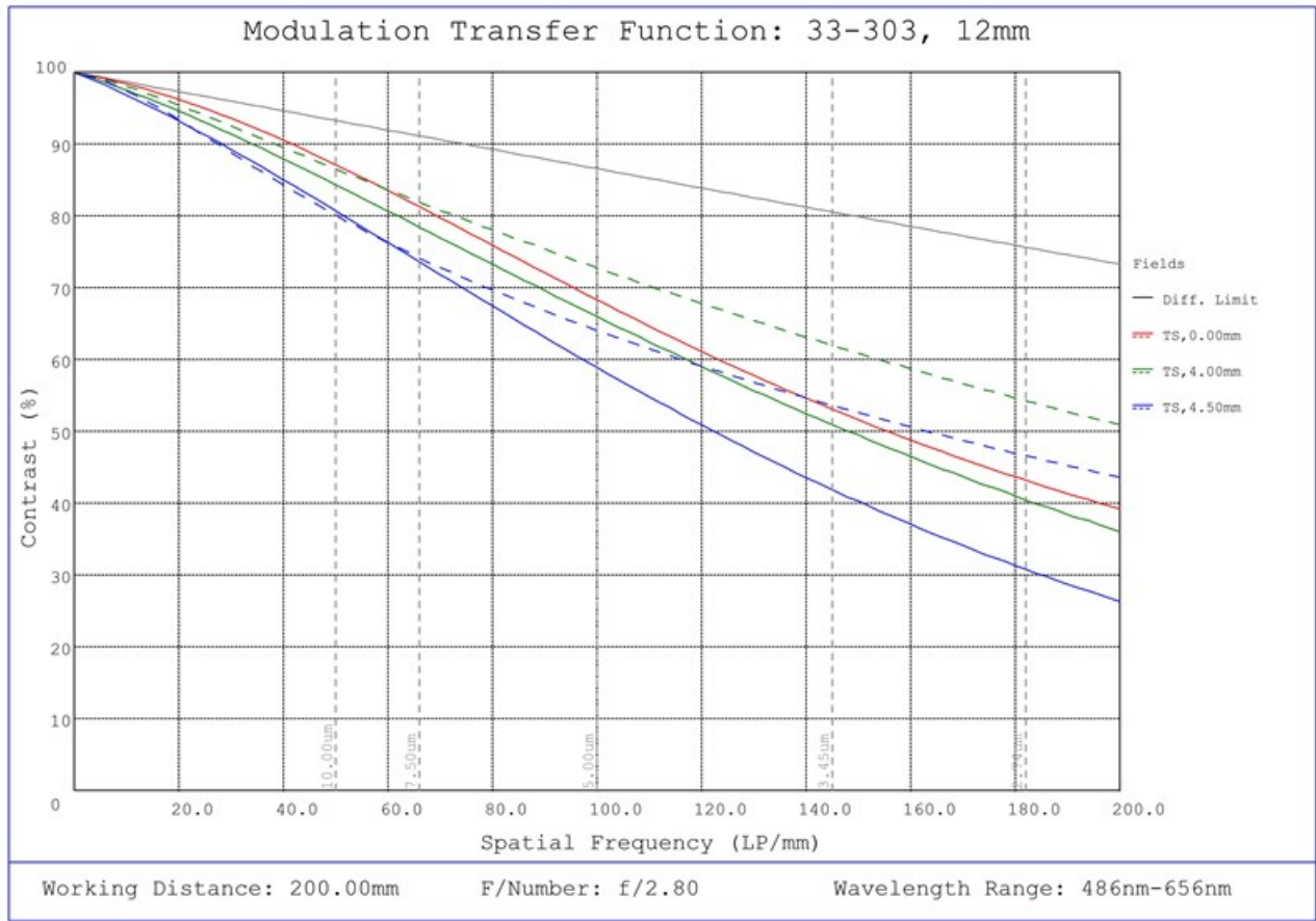
#33-303, 12mm UC Series Fixed Focal Length Lens, Modulated Transfer Function (MTF) Plot, 200mm Working Distance, f2.8
