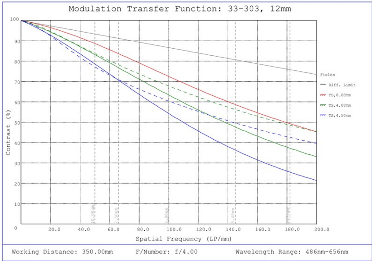
#33-303, 12mm UC Series Fixed Focal Length Lens, Modulated Transfer Function (MTF) Plot, 350mm Working Distance, f4
