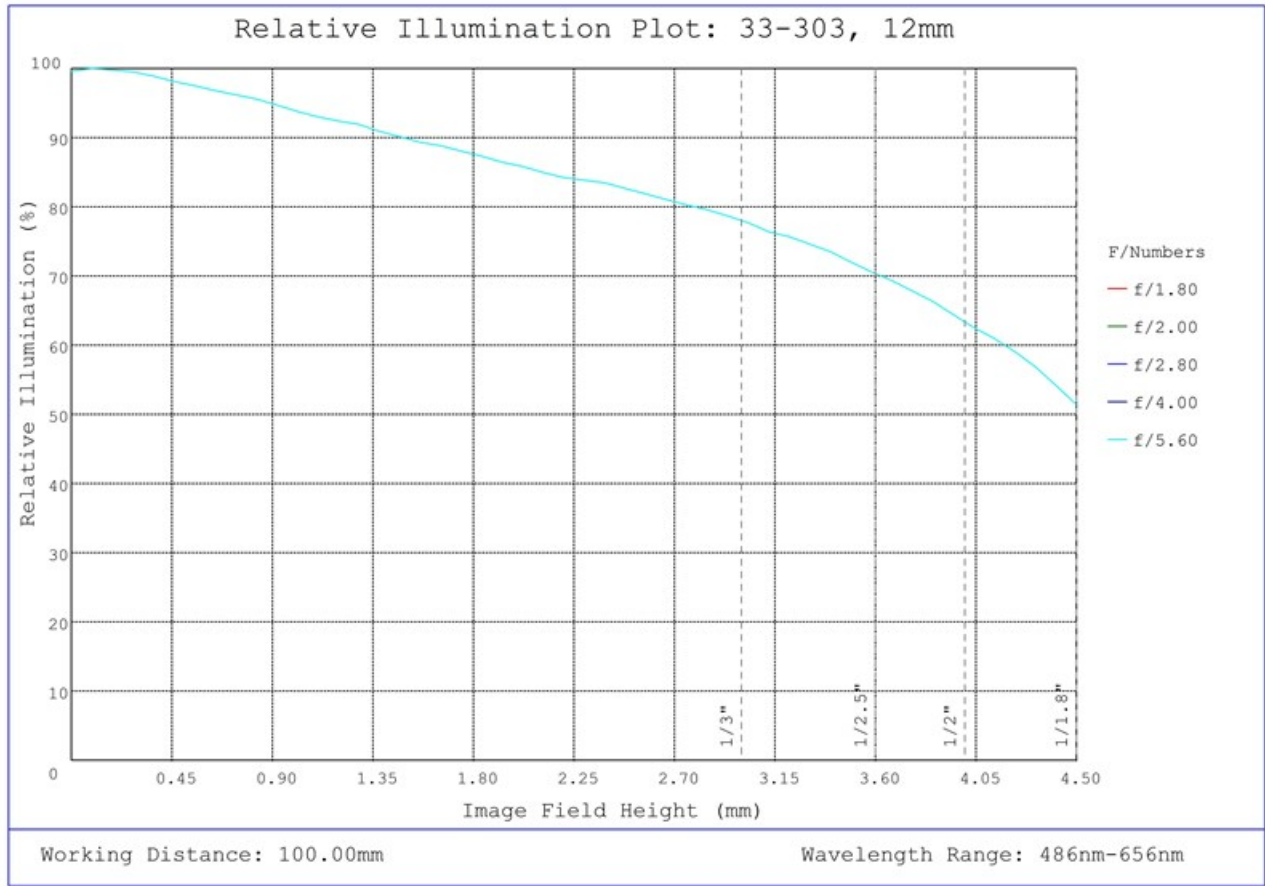
#33-303, 12mm UC Series Fixed Focal Length Lens, Relative Illumination Plot
