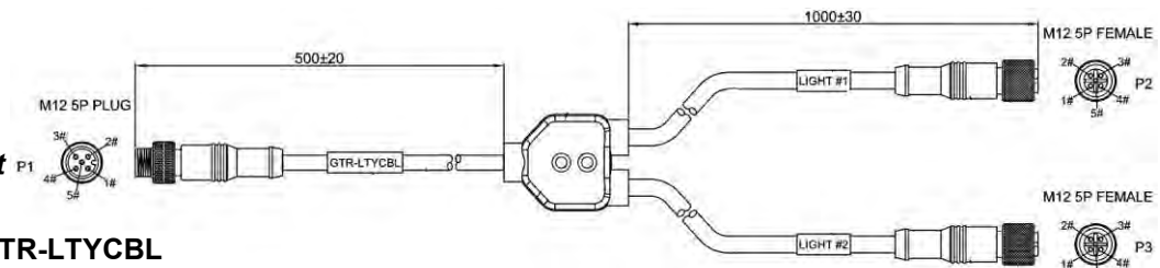
Light Breakout Cable
